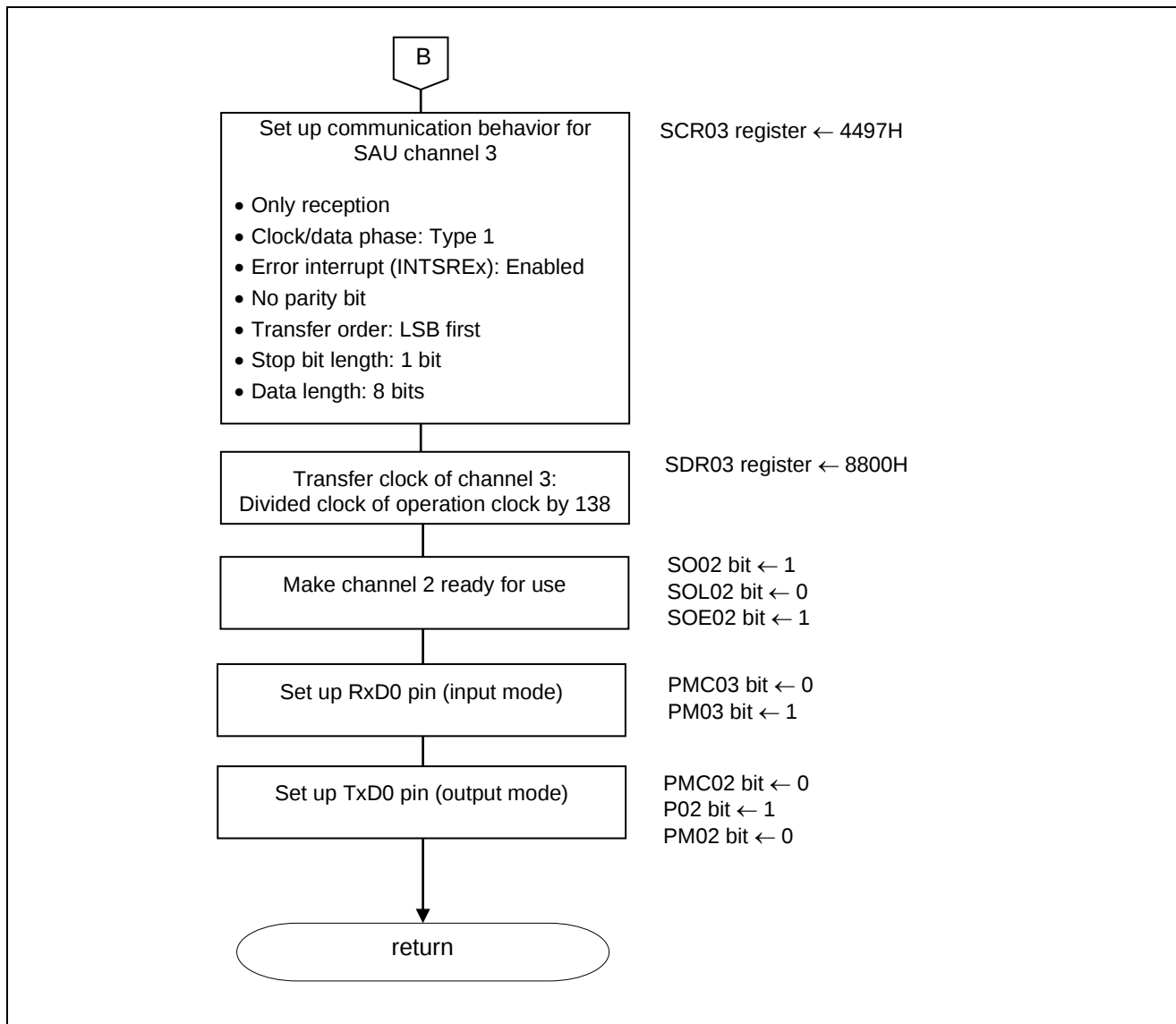
Figure 5.9 UART1 Setup (3/3)
