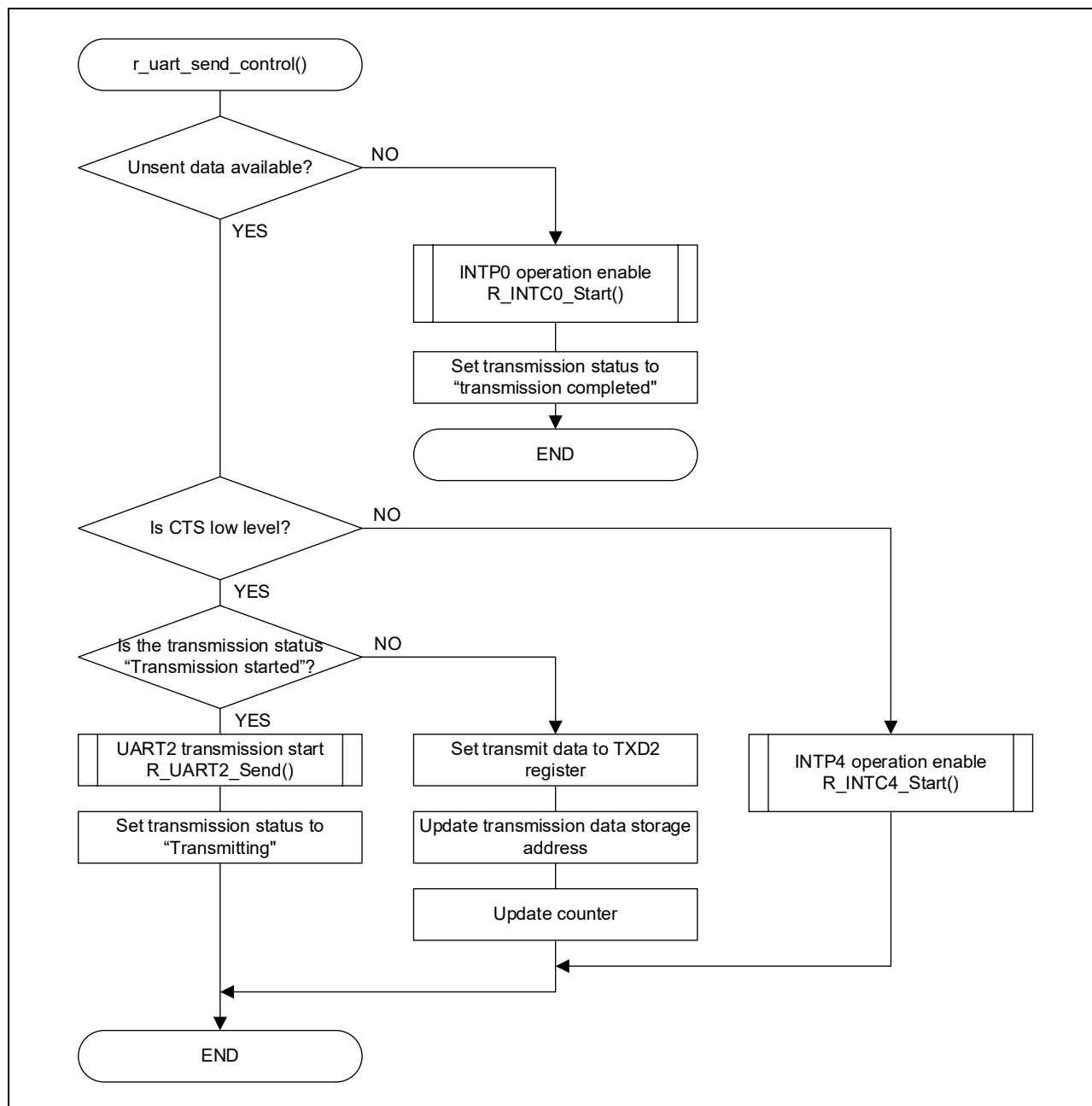
Figure 4-9 Transmission Control Function
