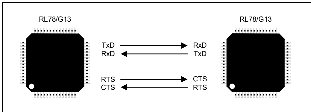
Figure 1-1 Flow Control Block Diagram
