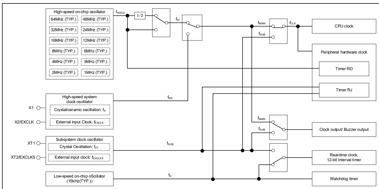
Figure 1.2 Block Diagram of Clock Generator (RL78/G13)
