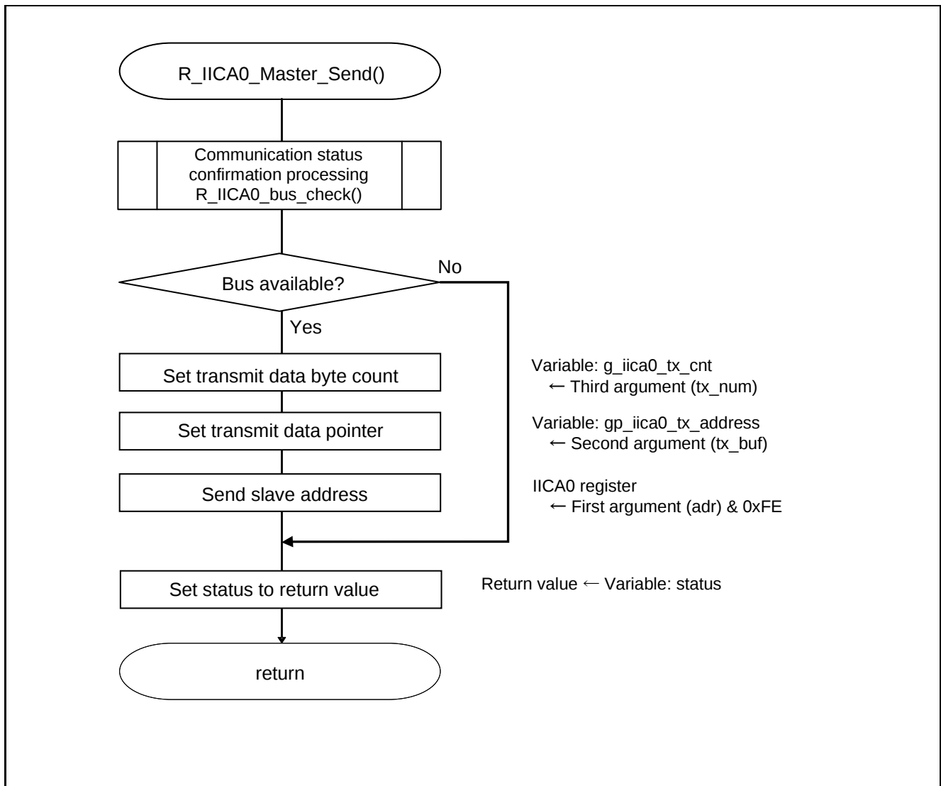
Figure 5.12 Master Transmission Start Request Processing
