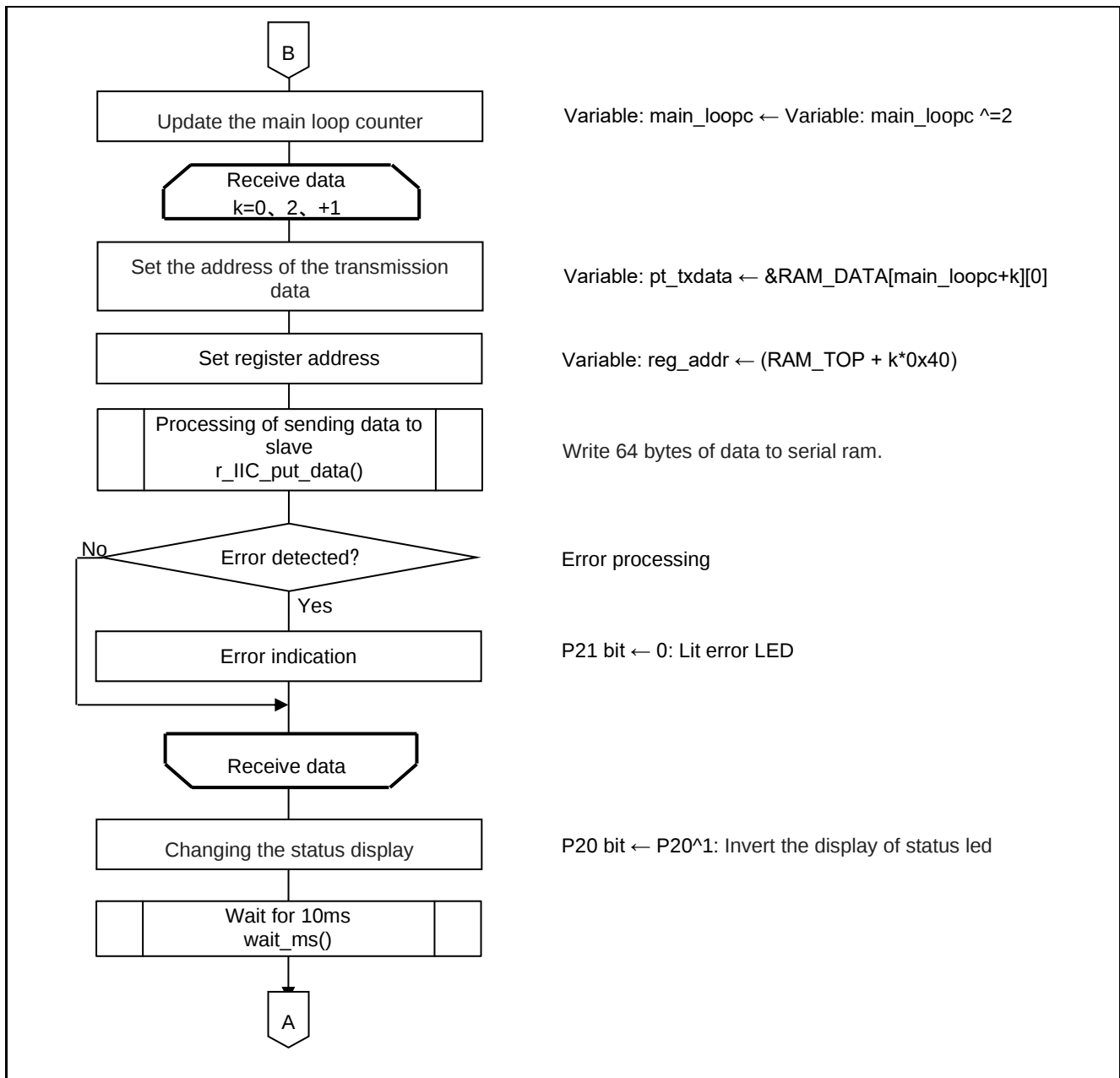
Figure 5.3 Main Processing (3/3)
