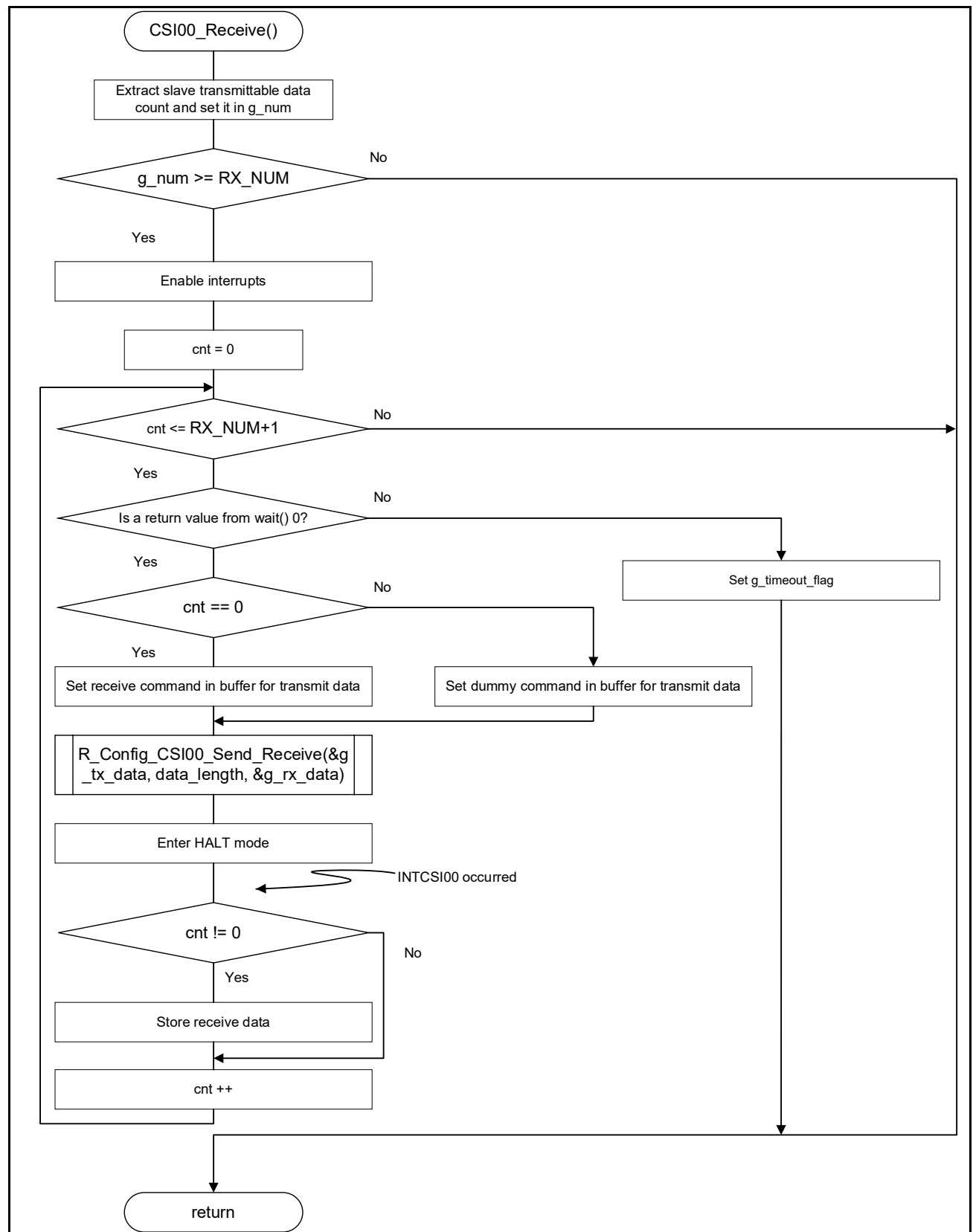
Figure 5-6 CSI Reception
