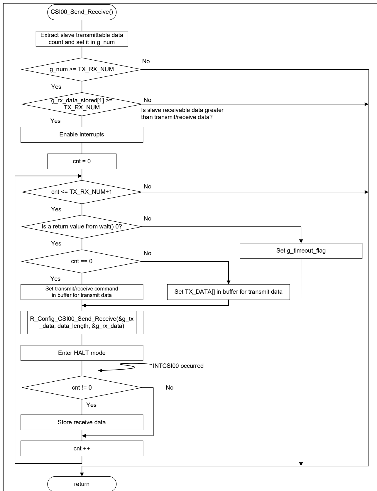
Figure 5-4 CSI Transmission/Reception
