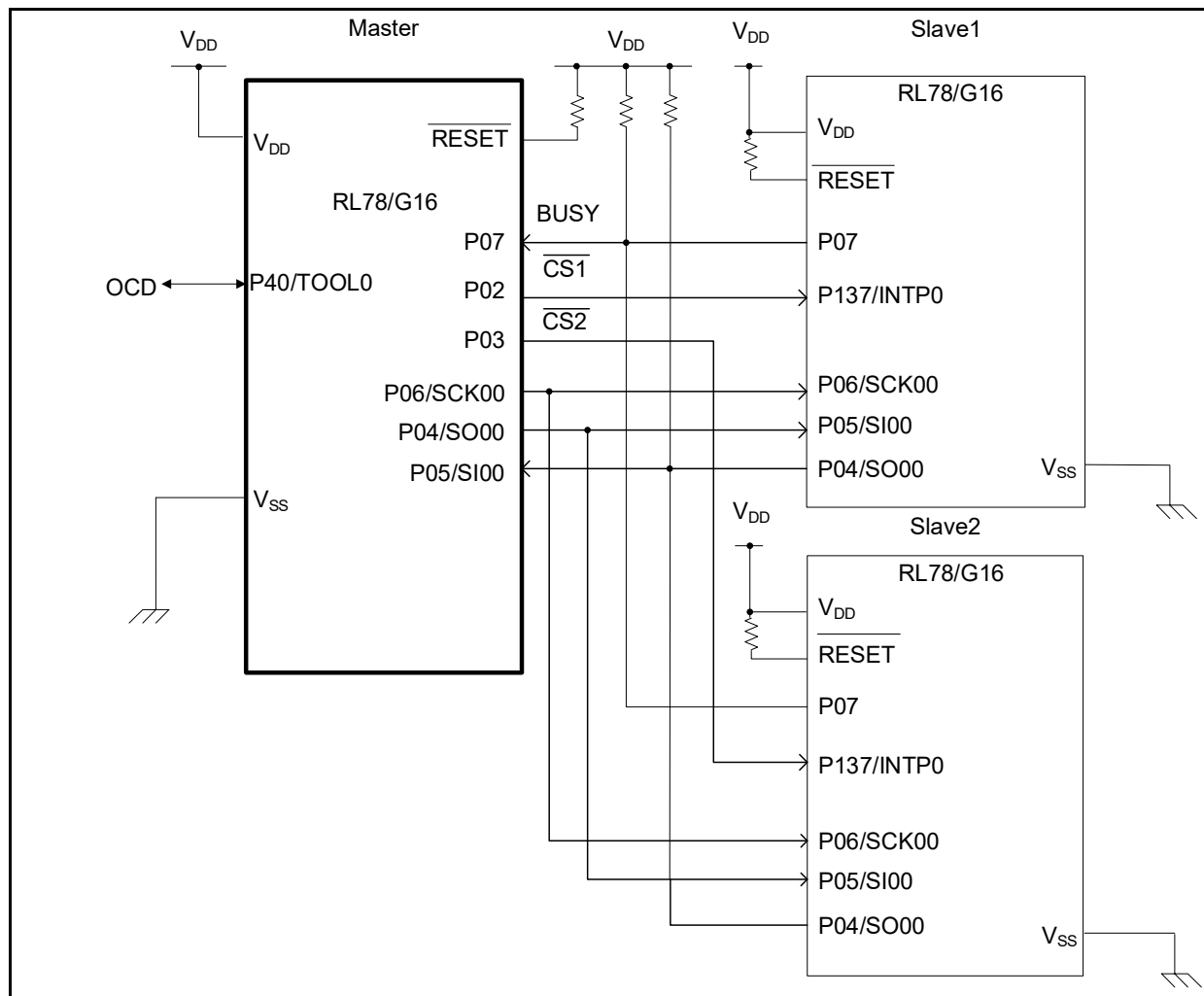
Figure 4-1 Hardware Configuration
