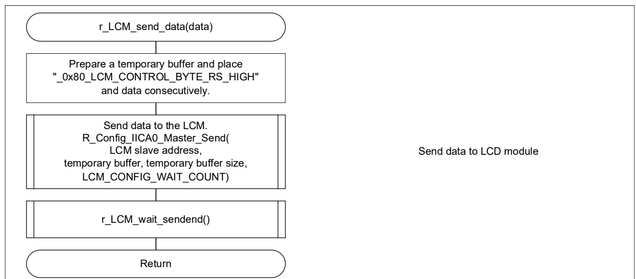
Figure 4.10 LCD Module Data Transmission Processing
