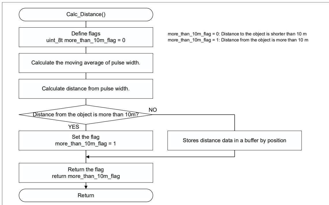
Figure 4.2 Process of Converting High level Width Measurement Results into Distance.
