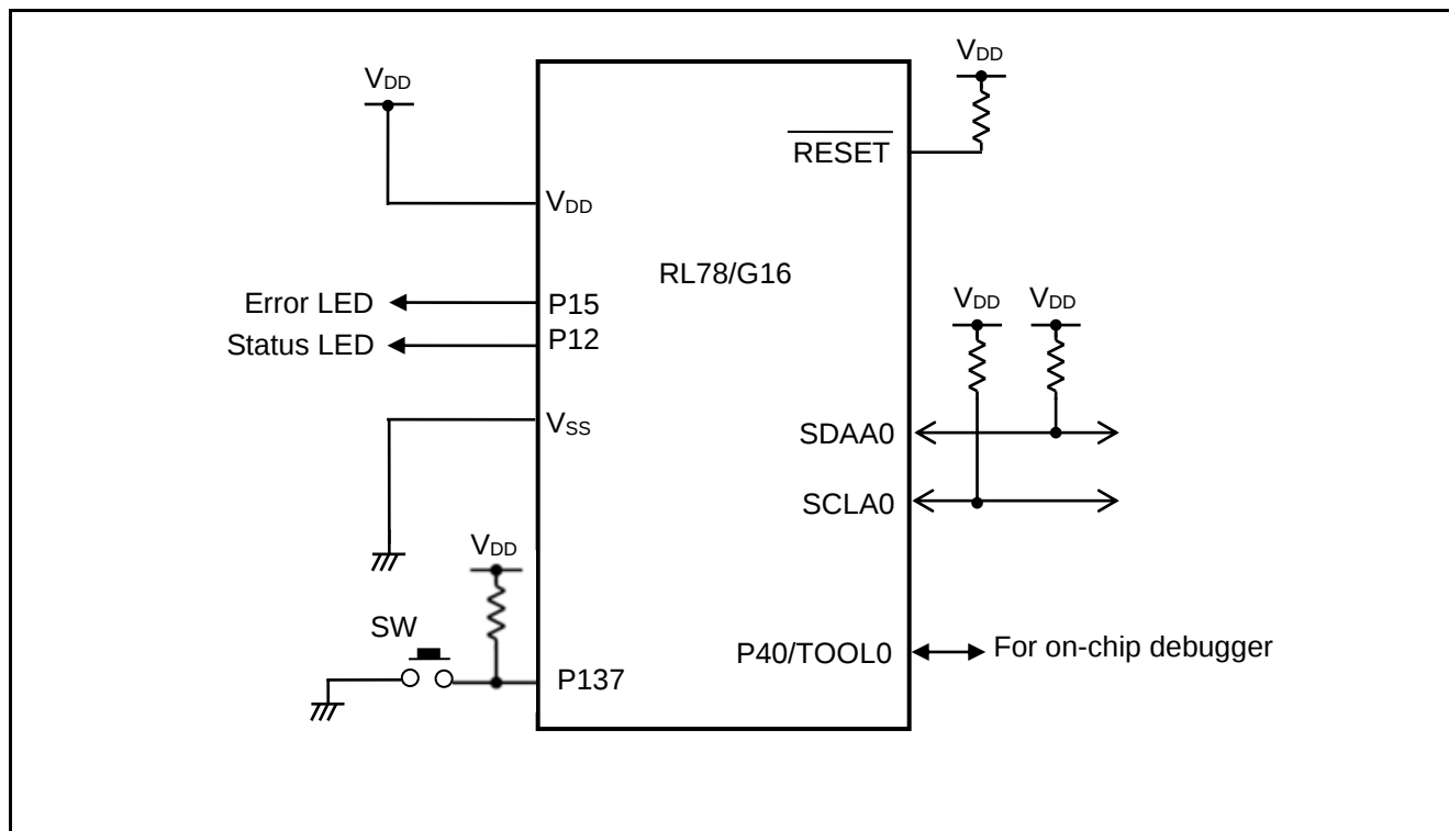
Figure 4.1 Hardware Configuration
