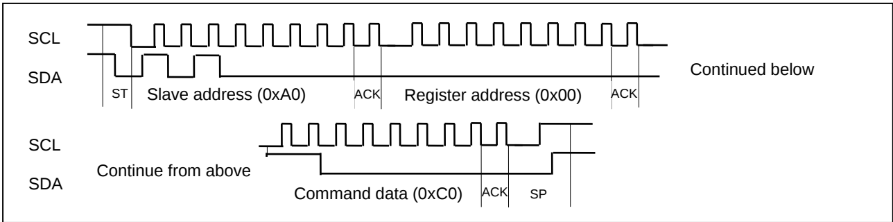
Figure. 1.10 Command Setting Timing Chart
