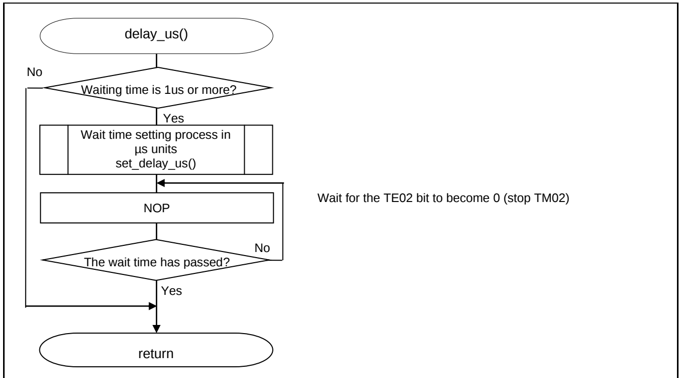
Figure 5.21 Time Wait Processing In \mu\text{s} units
