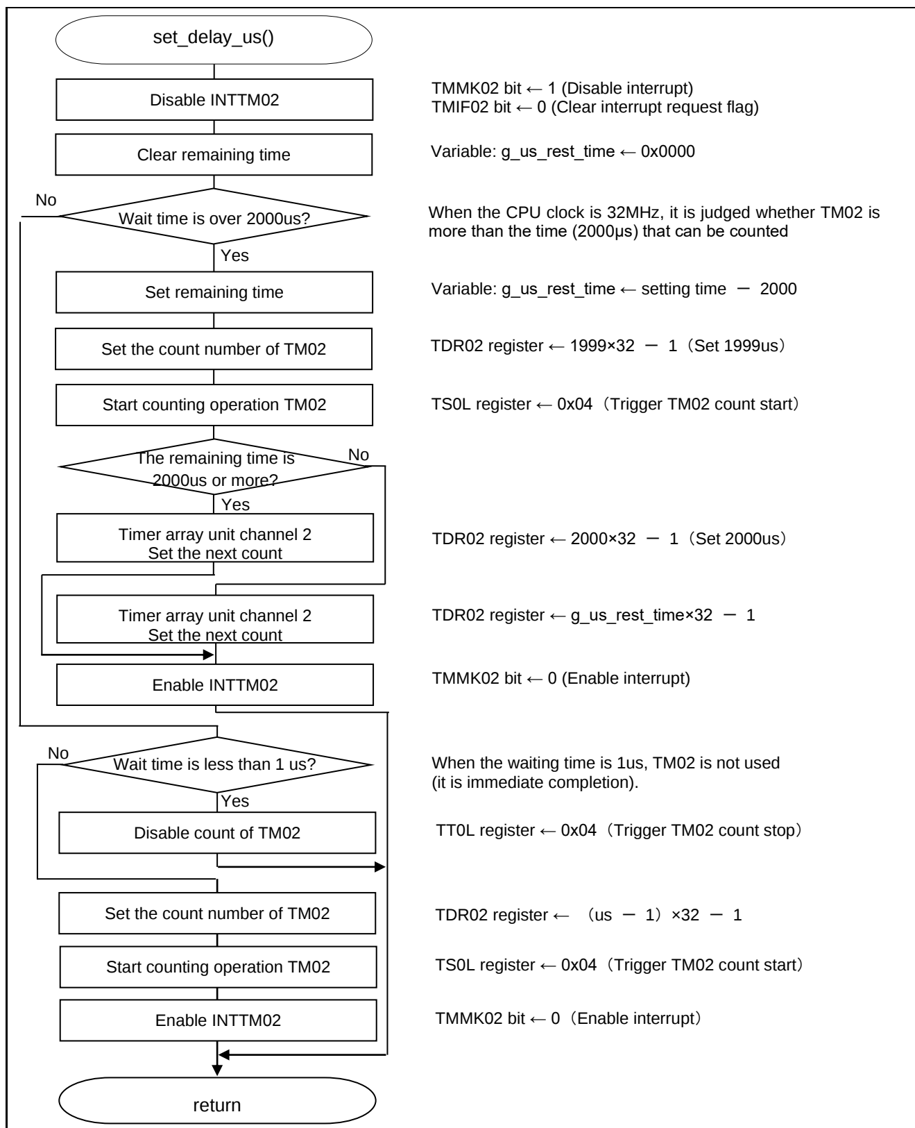
Figure 5.22 Wait Time Setting Process In \mu\text{s} units
