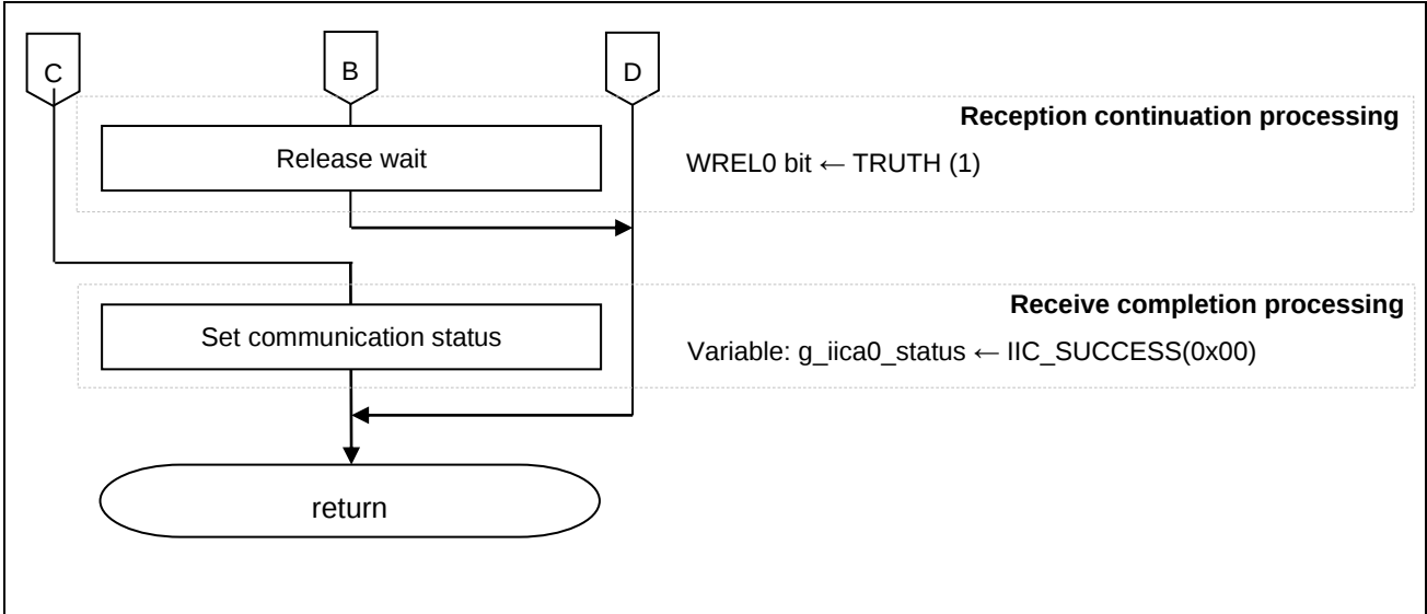
Figure 5.20 IICA0 Interrupt Processing (3/3)
