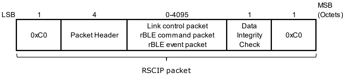
Figure 3-2 RSCIP packet
