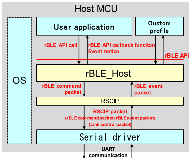
Figure 3-1 Host MCU Processing Flow
