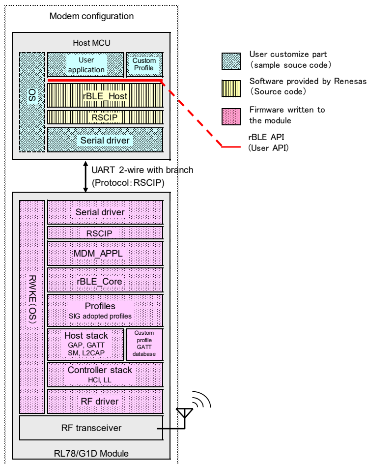
Figure 1-1 Software Structure
