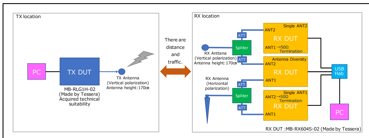
Figure 9. ANT1: Horizontal polarization ANT2: Vertical polarization
