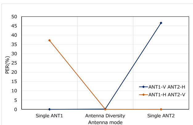
Figure 12. PER characteristics of Test 1
