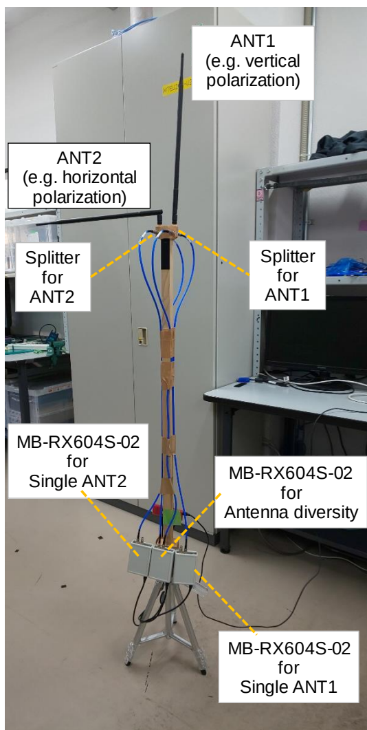
Figure 10. receiving system
