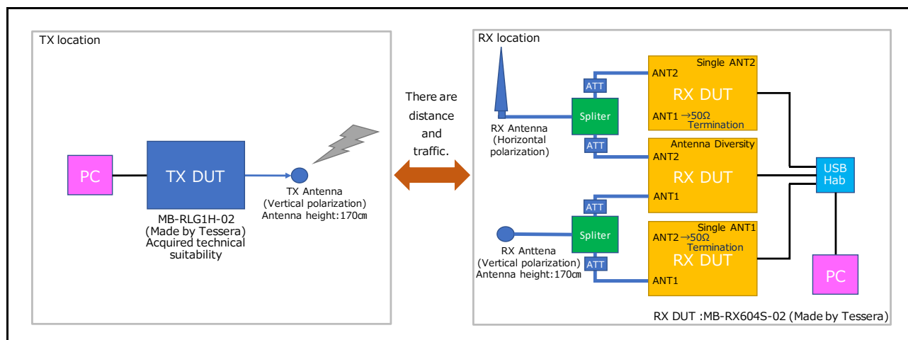
Figure 8. ANT1: Vertical polarization ANT2: Horizontal polarization
