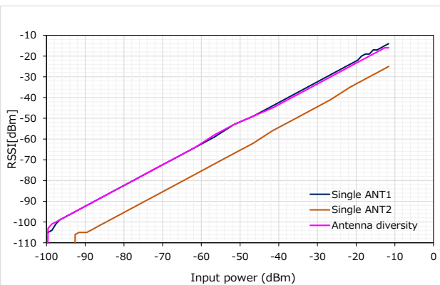
Figure 5. RSSI (ATT10dB on ANT2 side)
