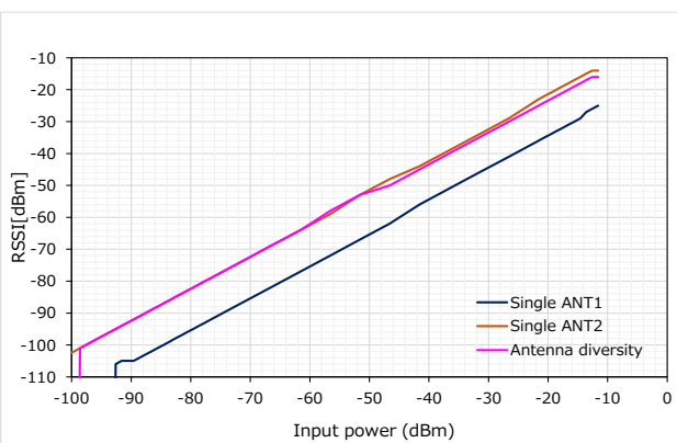
Figure 7. RSSI (ATT10dB on ANT1 side)
