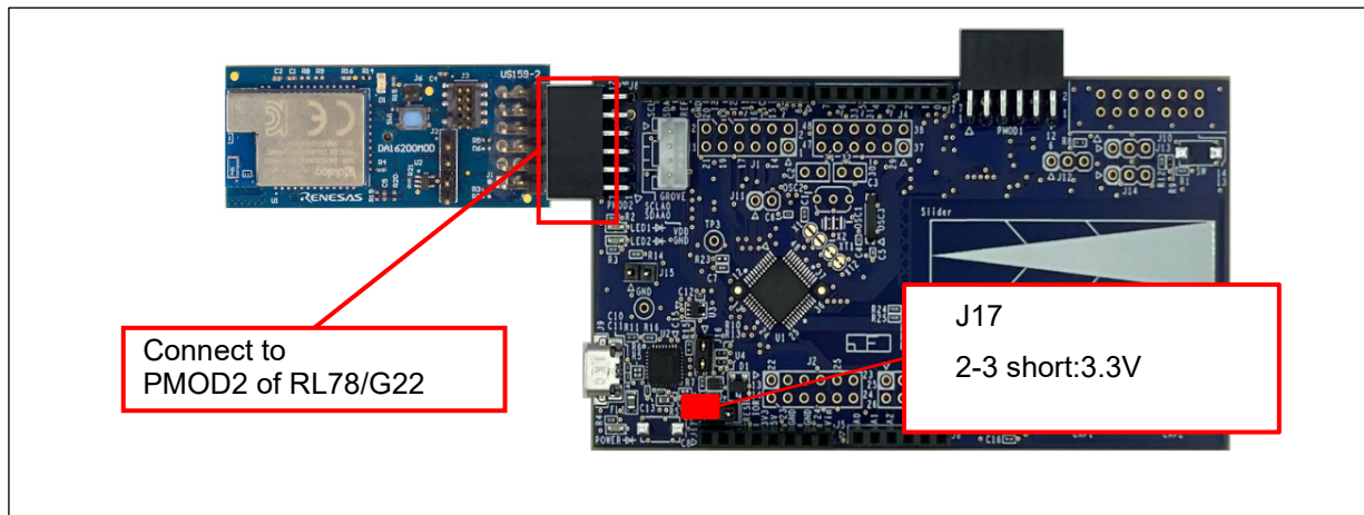
Figure 2-1 Connect RL78/G22 FPB and DA16200 / DA16600
