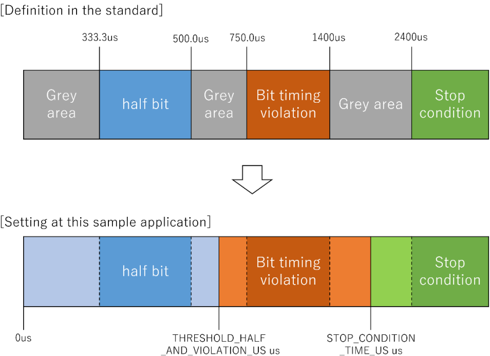
Figure 4-15 Definition in the standard for Receiver and the sample application setting (starting at the beginning of a logical bit)
