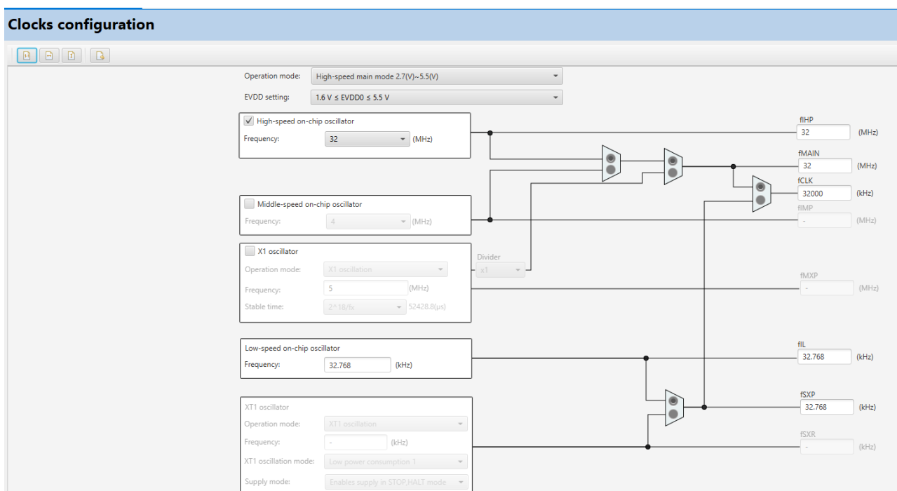
Figure 4-8 Clock setting
