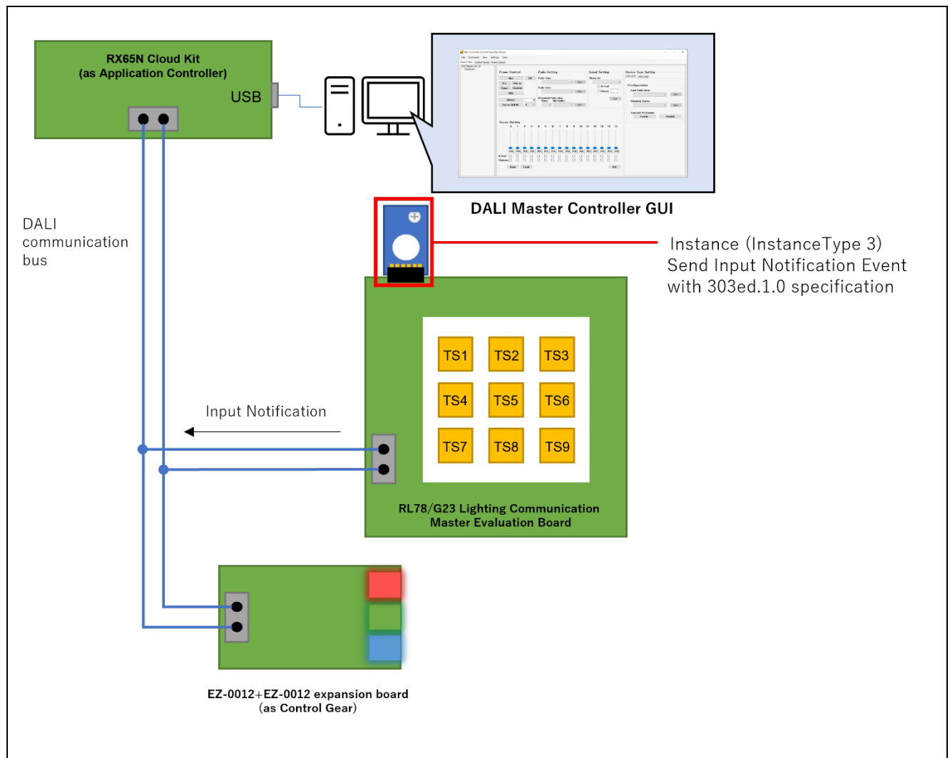
Figure 4-8 System configuration example (using RX65N Cloud kit + DALI-2 option board)
