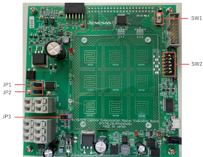
Figure 4-5 RL78/G23 Lighting Communication Master Evaluation Board Components
