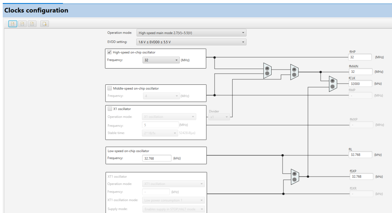
Figure 4-10 Clock setting
