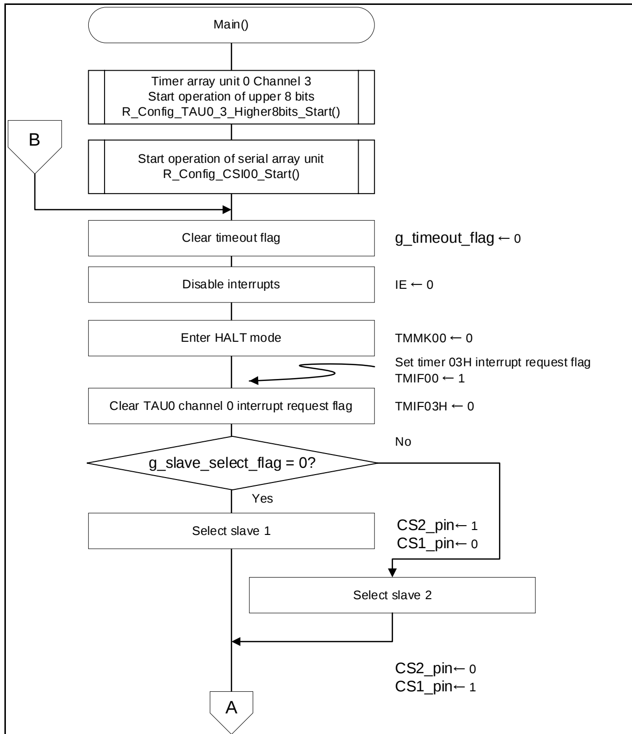
Figure 5-1 Main Processing 1/2
