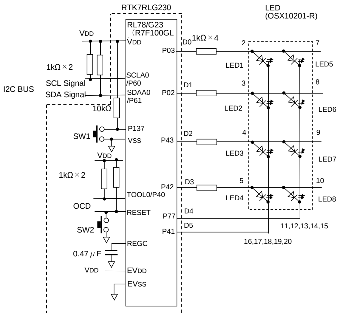
Figure 3-1 Hardware Configuration
