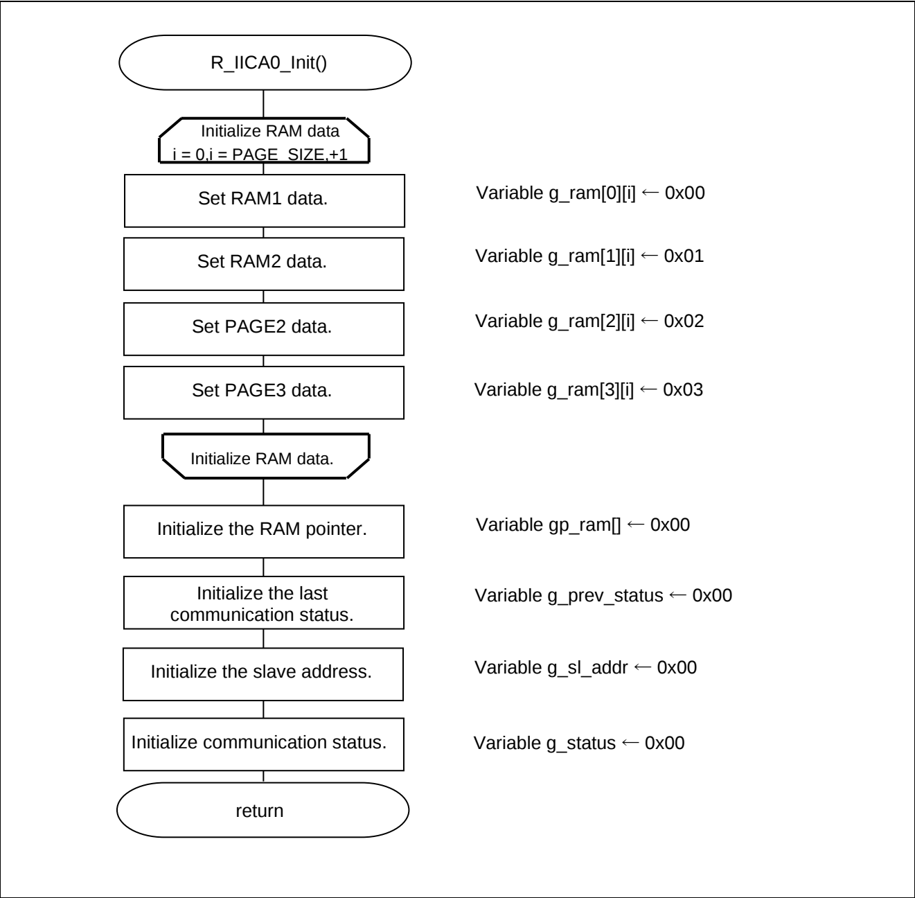
Figure 4-5 IICA0 Variables Initialization Processing Function
