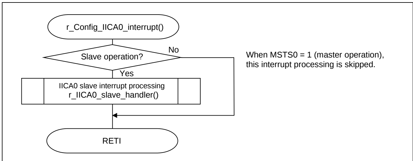
Figure 4-8 IICA0 Interrupt Processing Function
