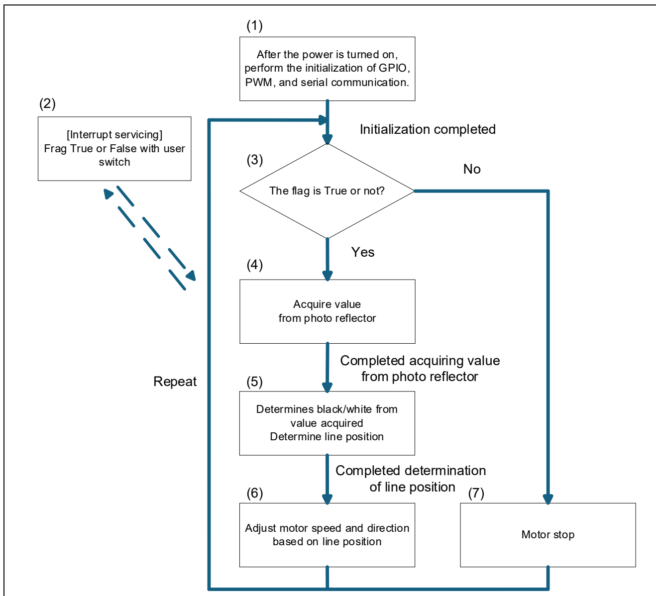
Figure 1-7 Overview of Operation
