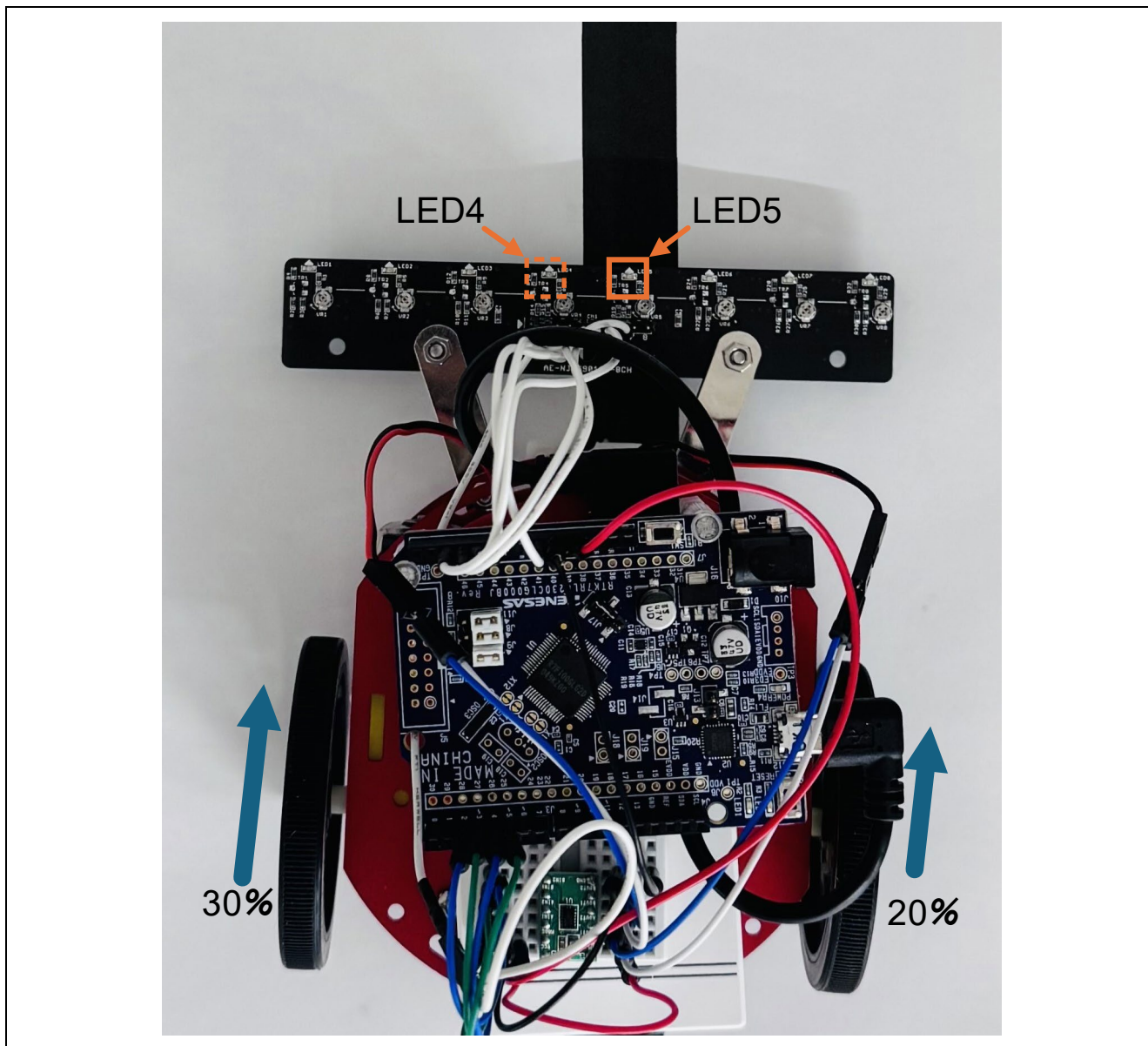
Figure 4-3 Image Figure Linear Auxiliary Operation
