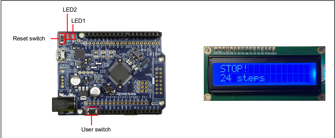
Figure 4-13 Position of the LED1 and switches and the display of the LCD module when ending the counting
