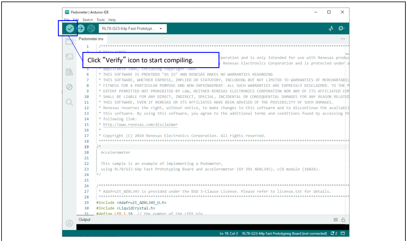
Figure 4-9 Compile sketch
