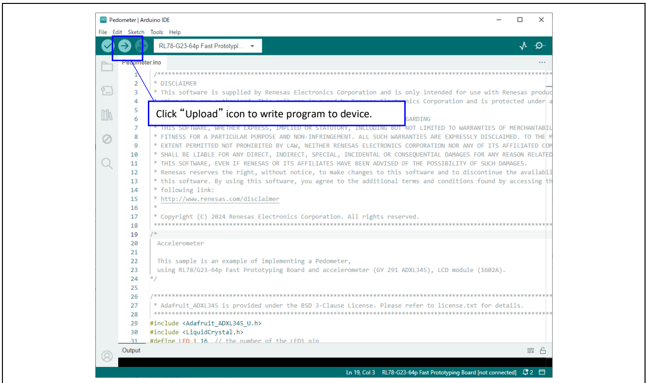
Figure 4-10 Write sketch to board
