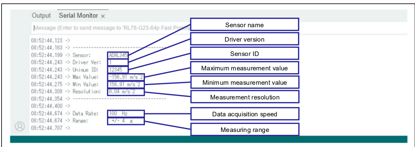
Figure 4-2 Content displayed on the serial monitor during development
