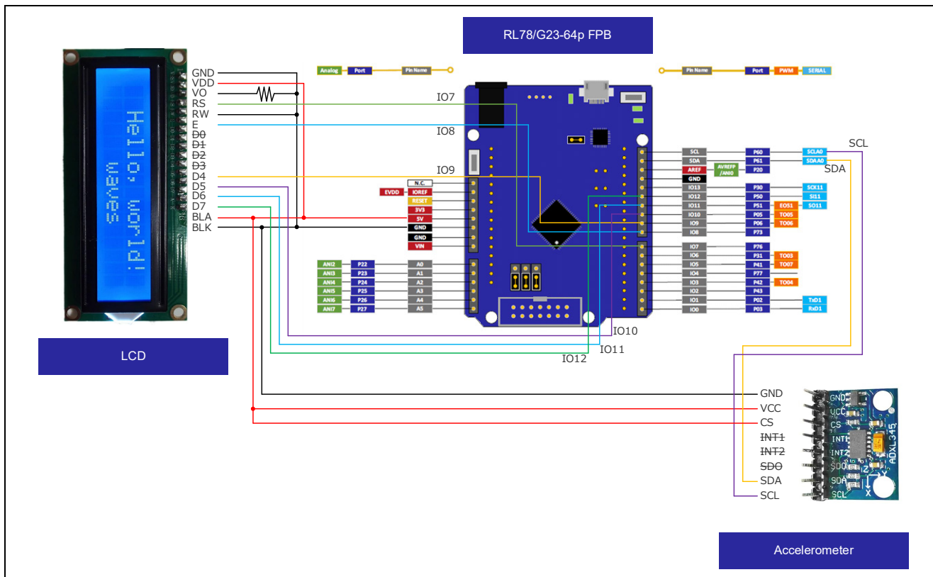
Figure 3-1 Connection of boards
