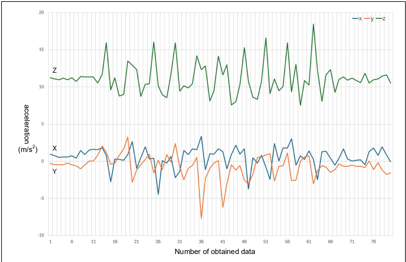
Figure 4-3 Changes of the acceleration along the three axes during walking
