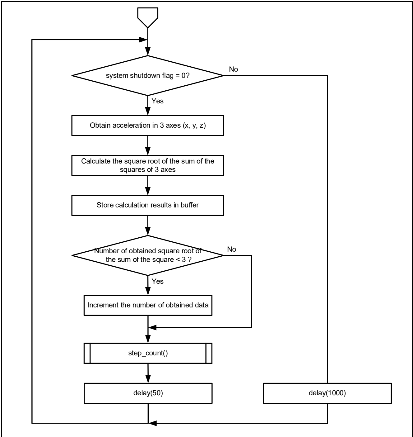
Figure 4-15 Flowchart of main processing (2/2)
