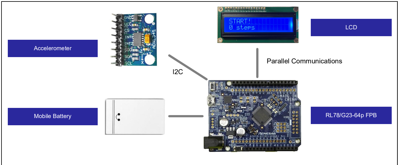
Figure 1-3 System configuration during step measurement
