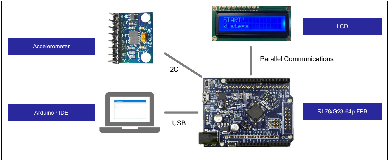
Figure 1-2 System configuration during development
