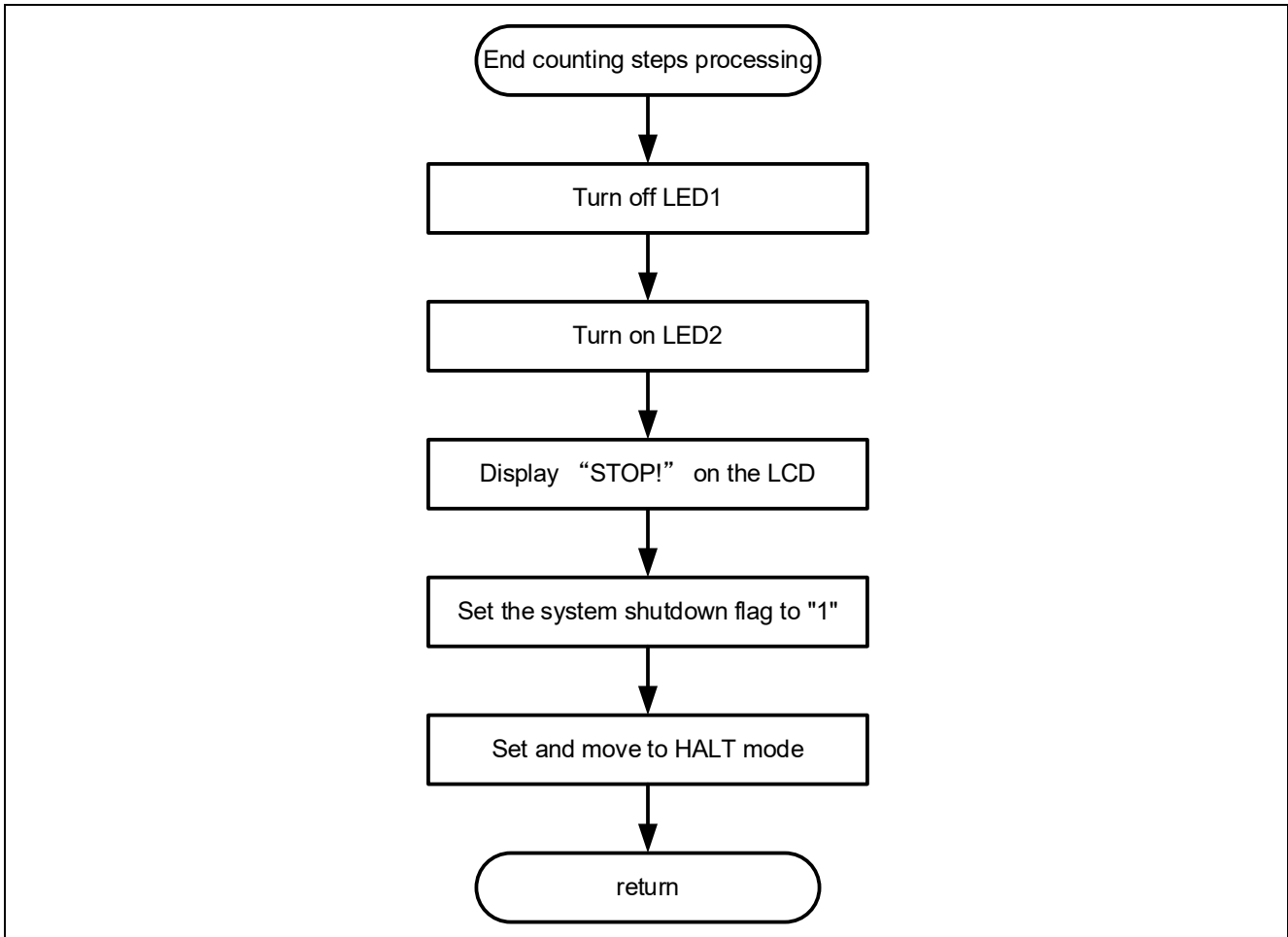
Figure 4-17 Flowchart of stop_system
