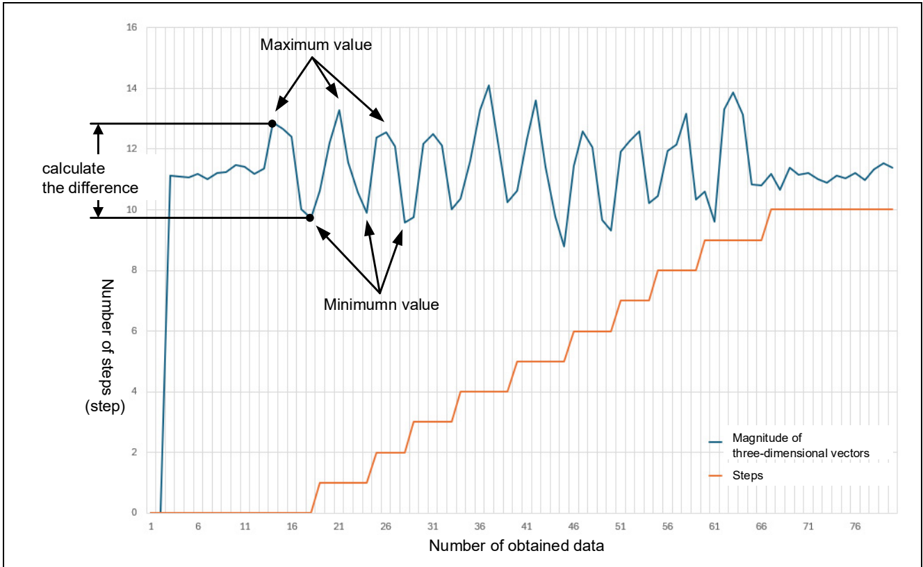
Figure 4-4 The counting steps
