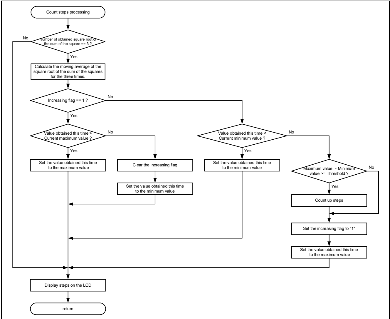
Figure 4-16 Flowchart of step_count
