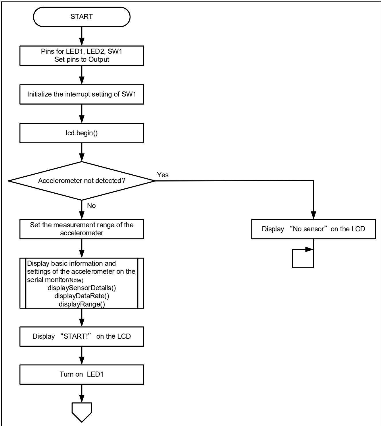
Figure 4-14 Flowchart of main processing (1/2)
