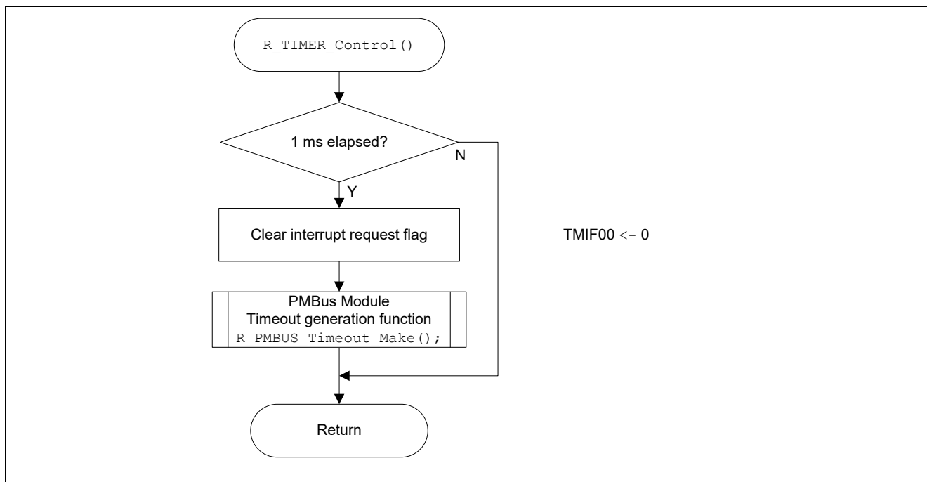
Figure 5.5 Timer Control Processing
