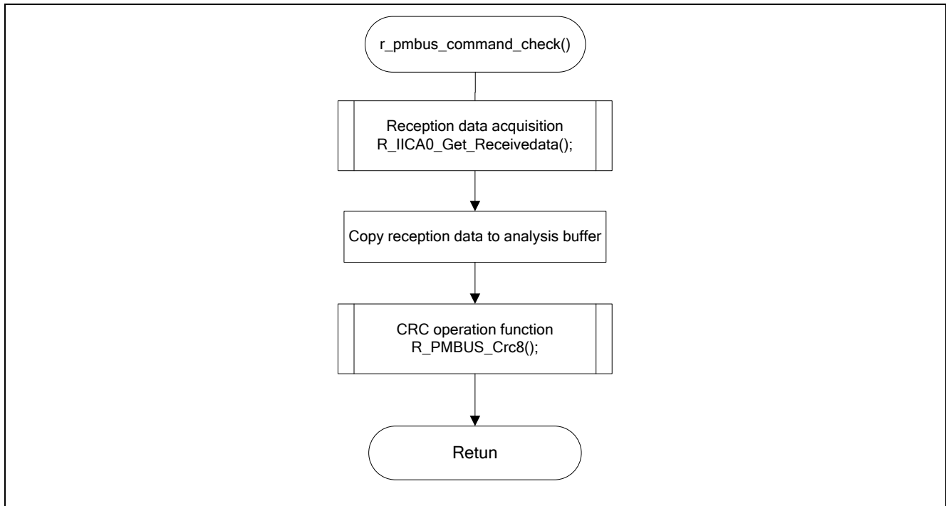
Figure 5.15 Command Analysis
