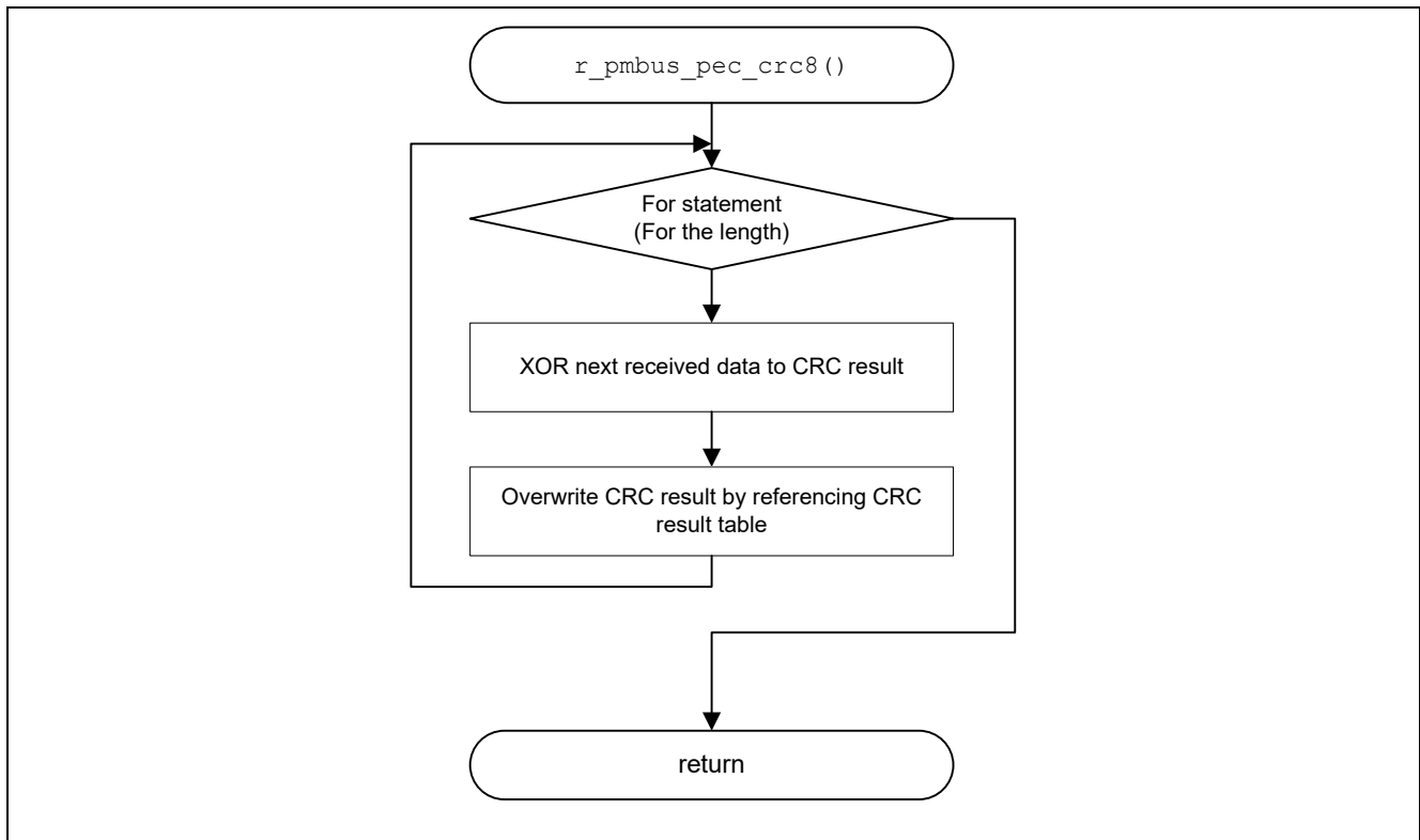
Figure 5.13 CRC8 Calculation
