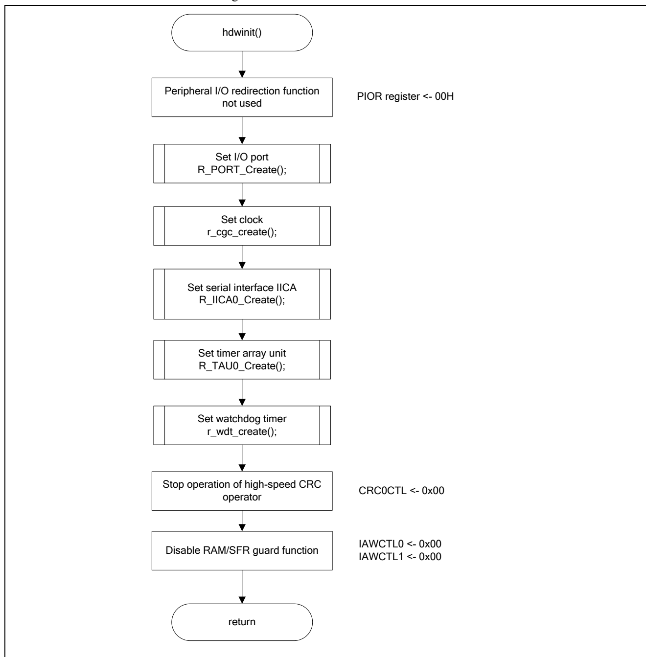
Figure 5.3 System Function
