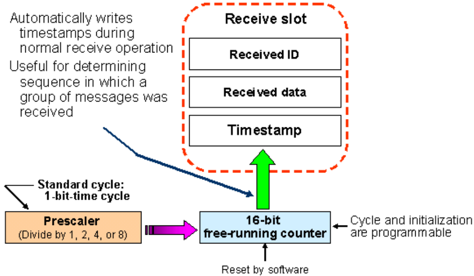
Figure 9. CAN Timestamp is available in each mailbox.
