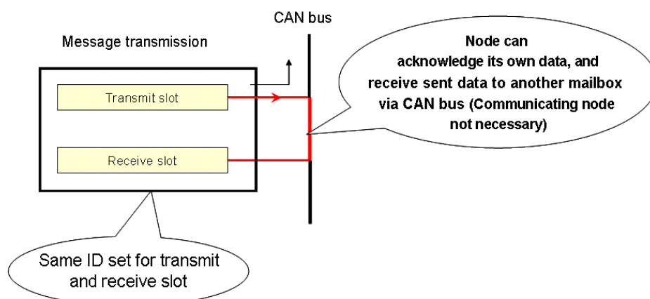
Figure 7. External Loopback: The message is transmitted onto the CAN bus and can be received back on the same node.
