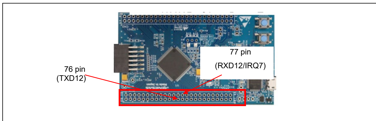
Figure 1-2 Jumper Cable Mounting Position
