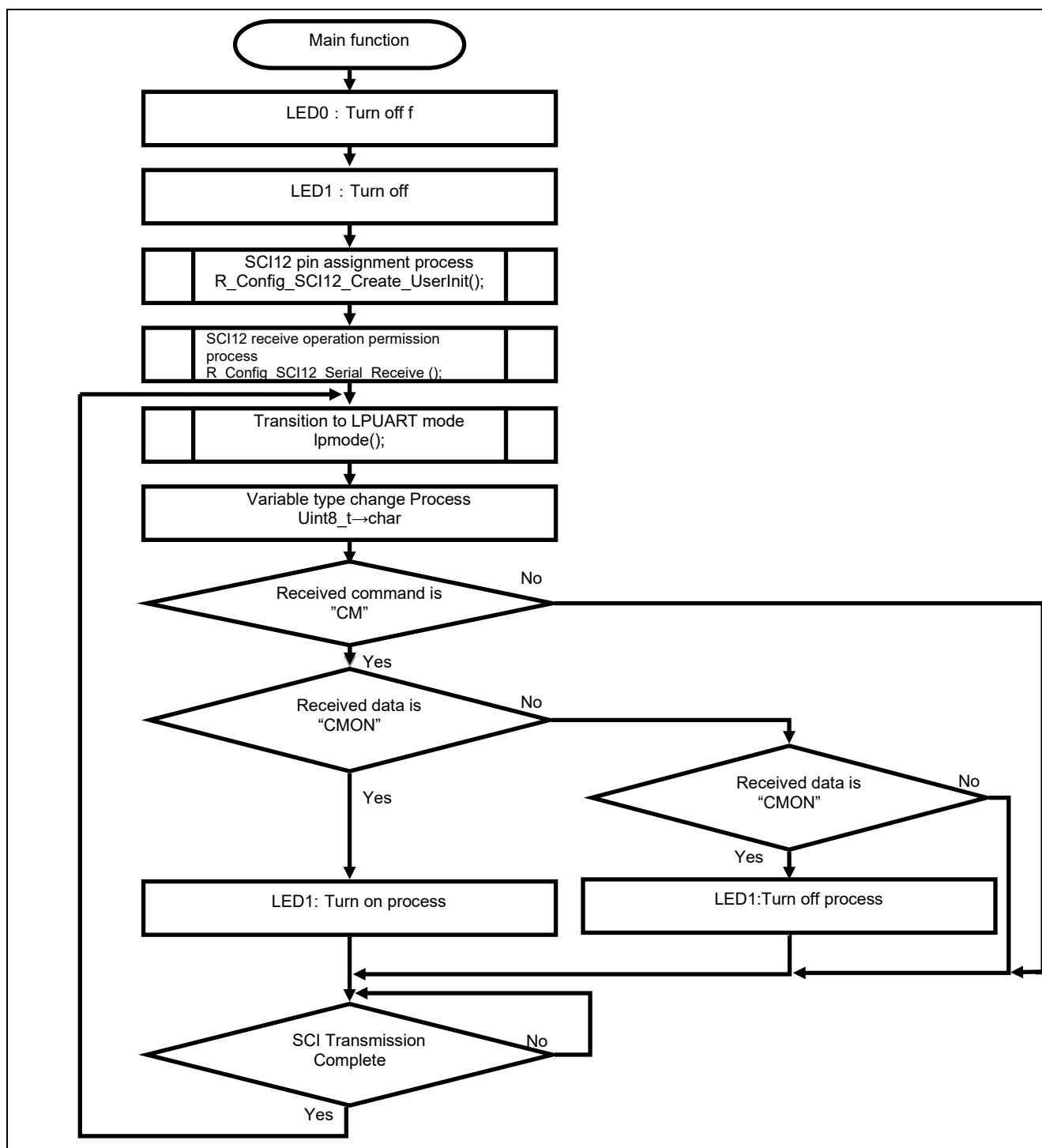
Figure 5-1 Main Function Flow
