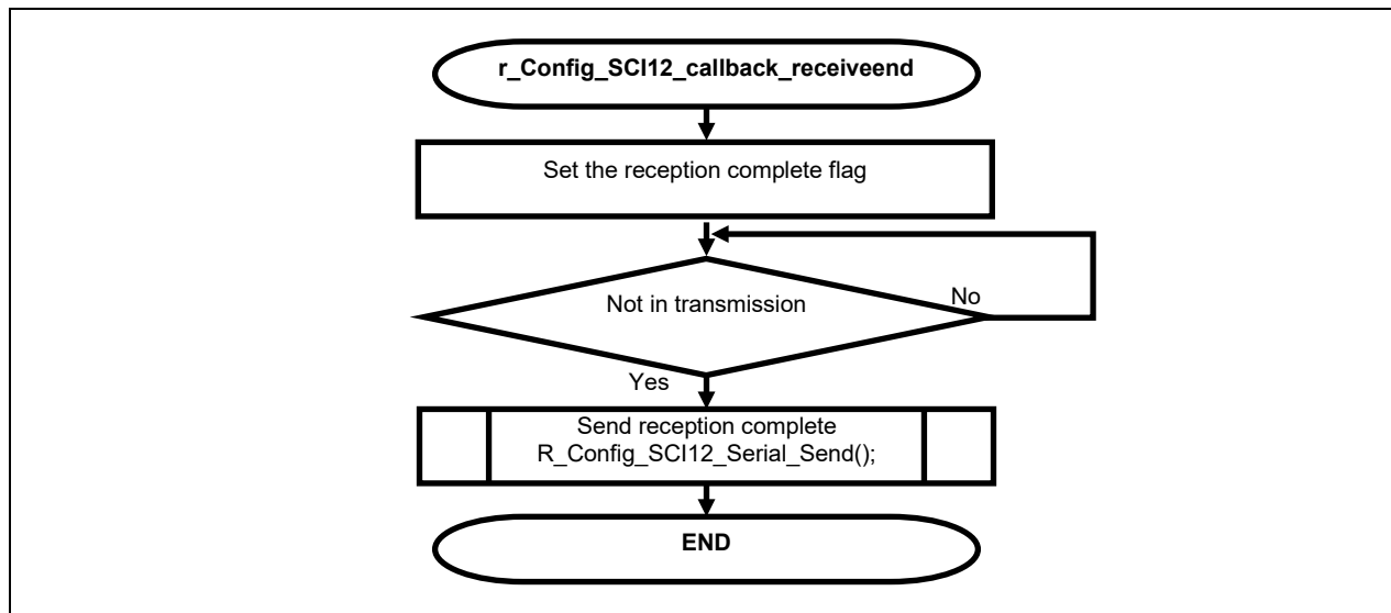
Figure 5-6 Flow of r_Config_SCI12_callback_receiveend
