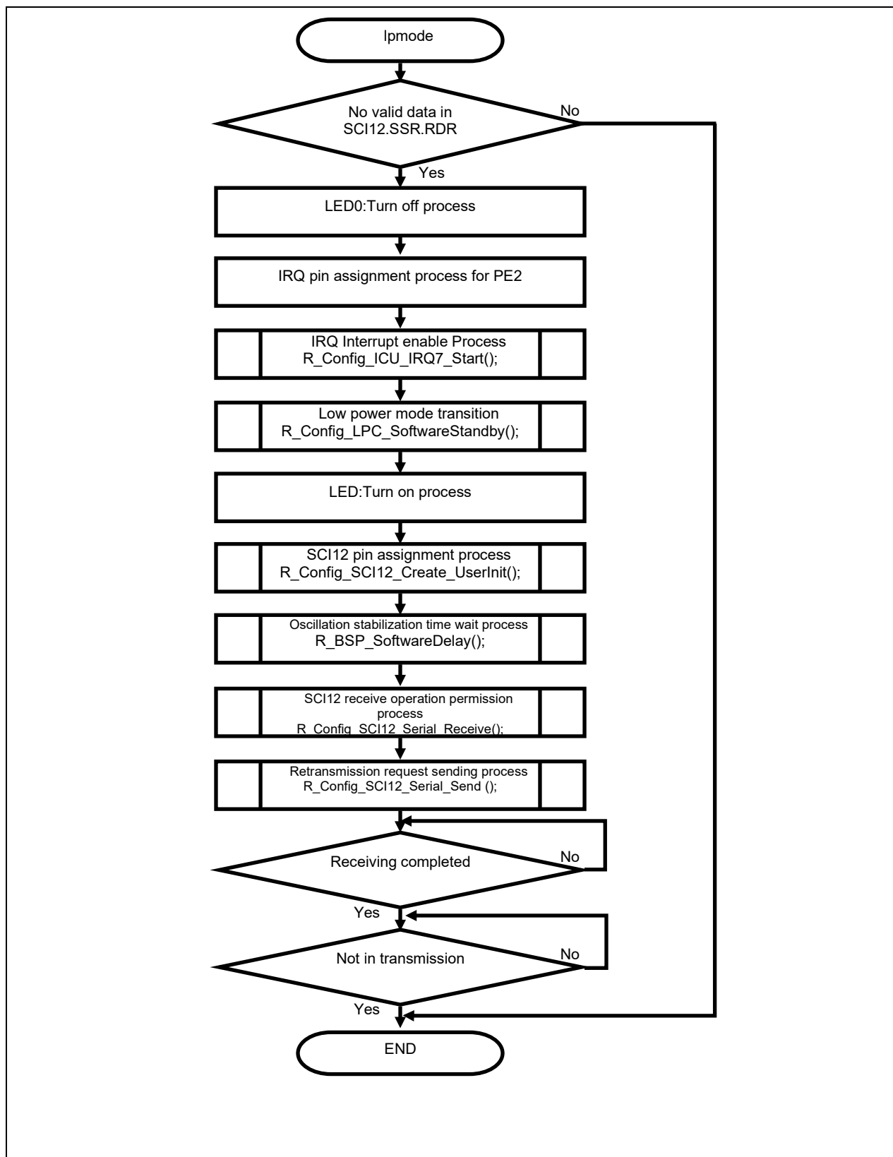
Figure 5-2 Ipmode Function Flow
