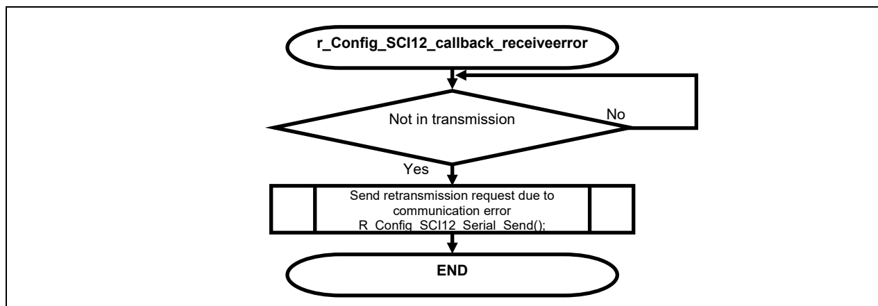
Figure 5-5 Flow of r_Config_SCI12_callback_receiveerror
