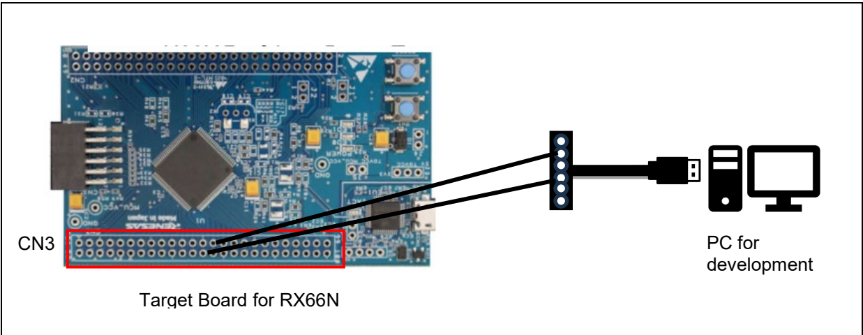
Figure 3-2 Target Board for RX66N Connection diagram
