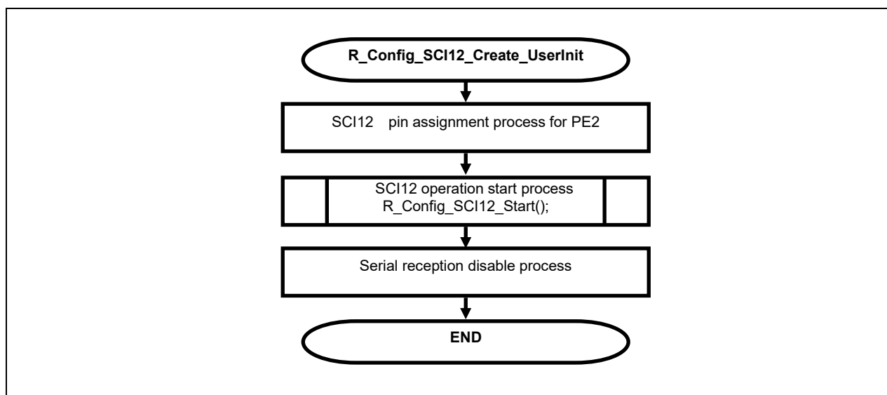
Figure 5-3 Flow of R_Config_SCI12_Create_UserInit
