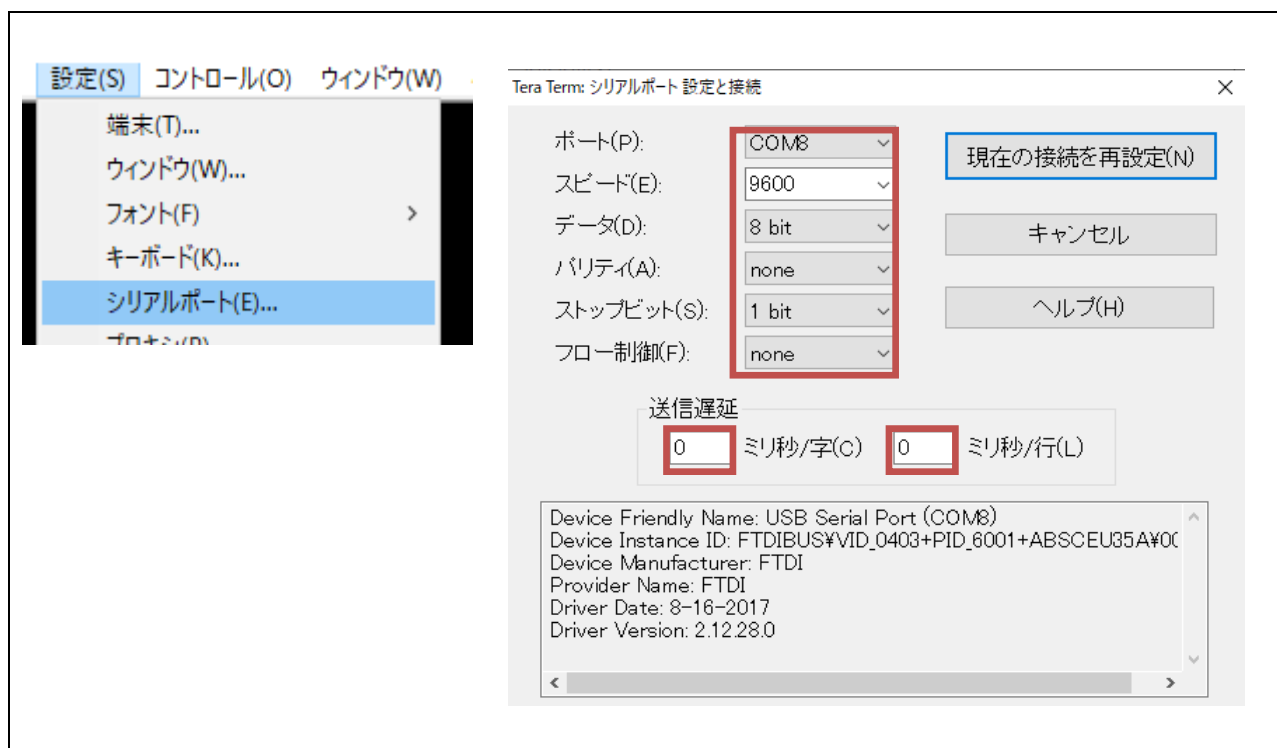
Figure 1-6 Serial Communication Settings
