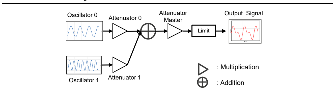
Figure 3.8 Sine Wave Generation Processing
