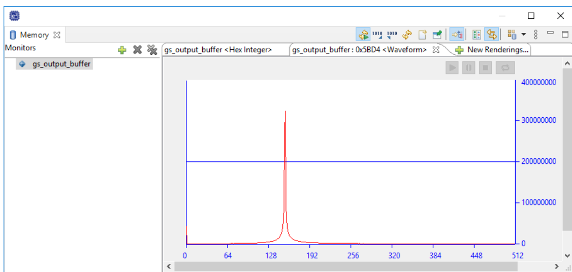
Figure 5.2 Waveform Rendering Display Example (Frequency Magnitude Characteristics Produced by FFT Processing)
