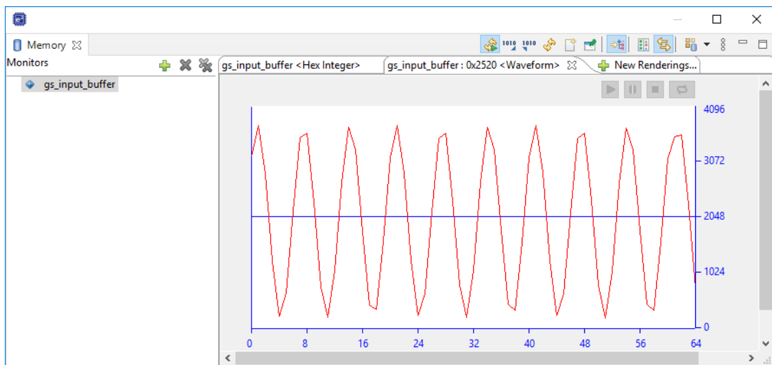
Figure 5.1 Waveform Rendering Display Example (Data Stored in Input Buffer)
