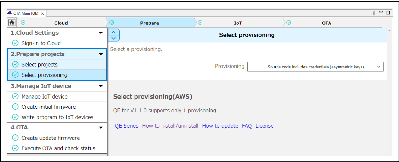
Figure 4-38 Provisioning Selection
