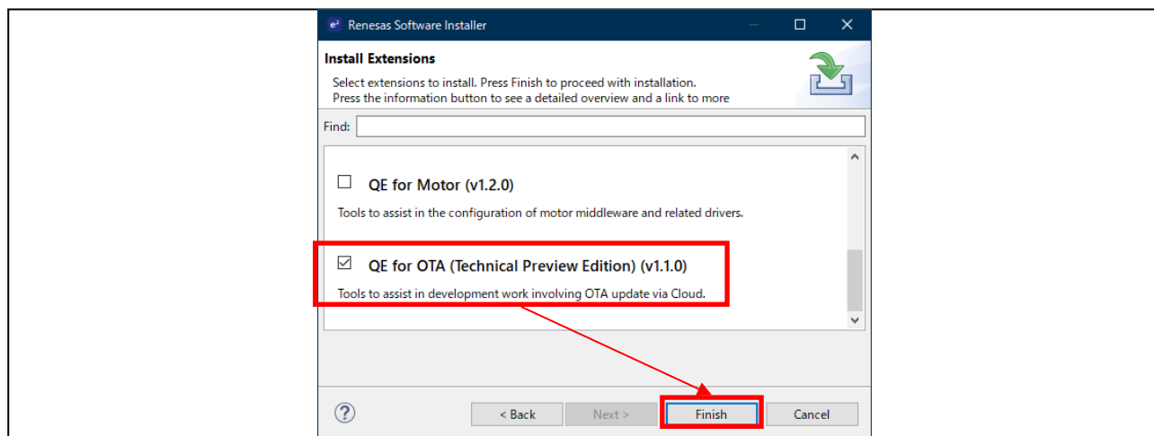
Figure 2-2 Install Extensions
