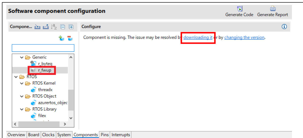
Figure 4-37 Download Components
