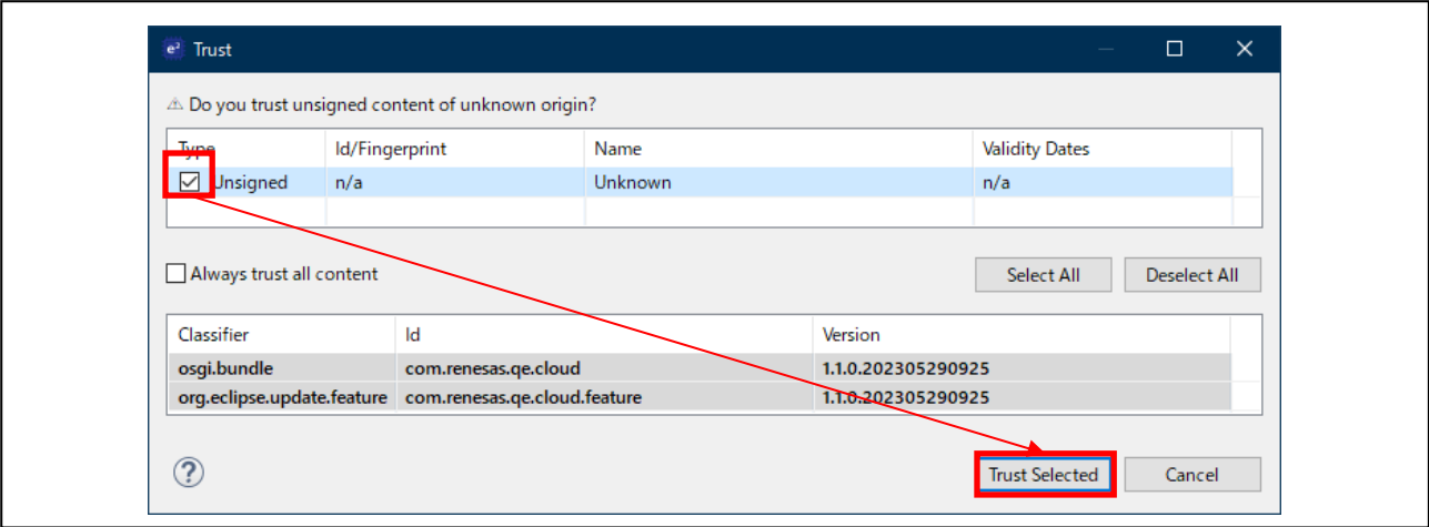
Figure 2-6 Trusted Tool
