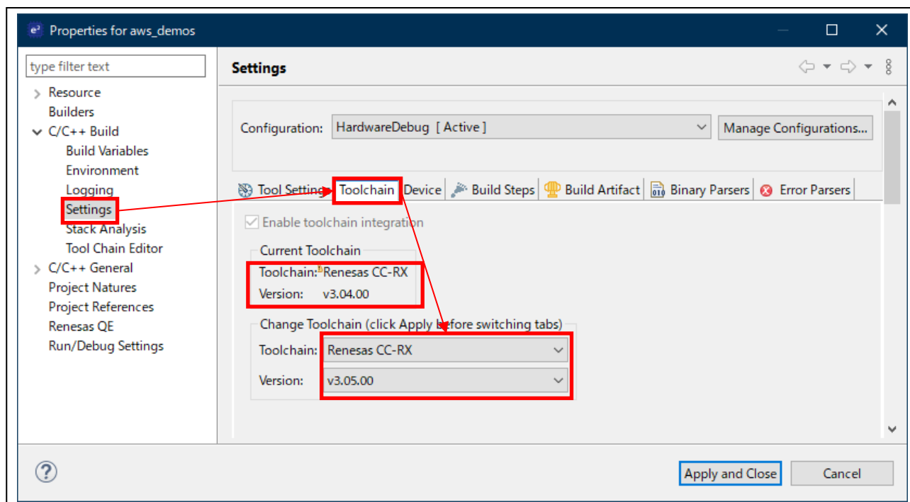
Figure 4-43 Toolchain Version
