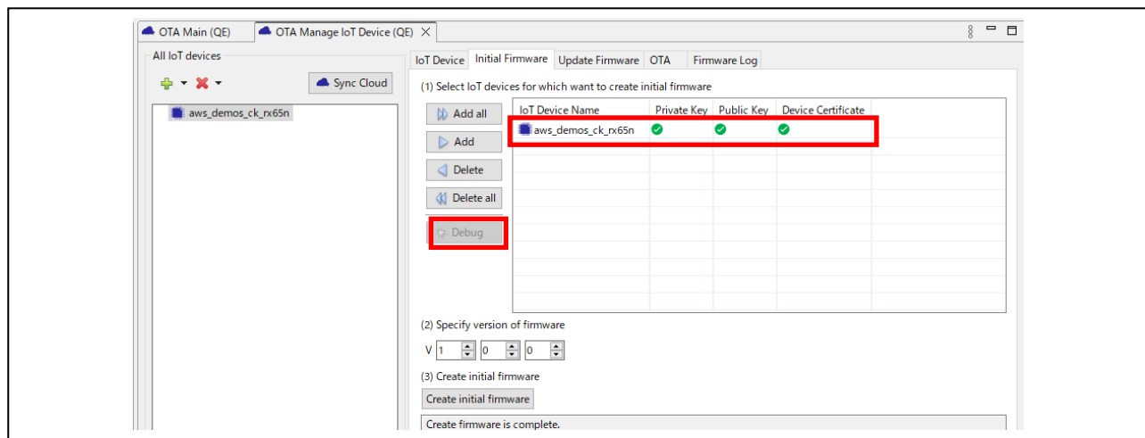
Figure 4-53 Debug Button
