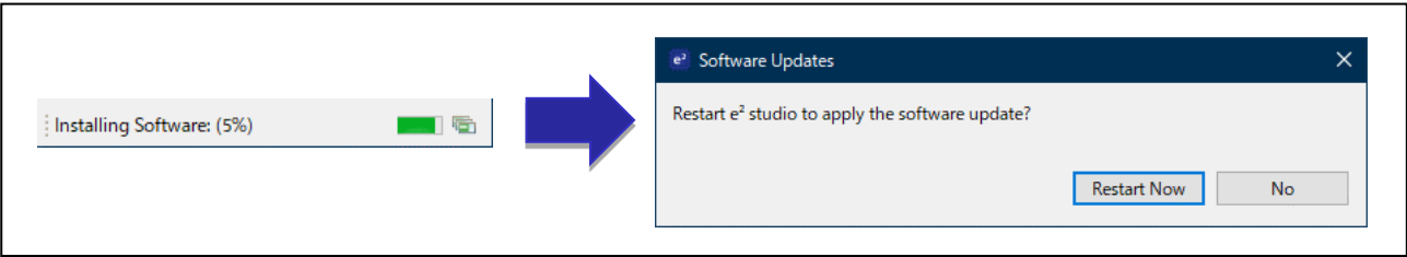
Figure 2-7 Installation Status
