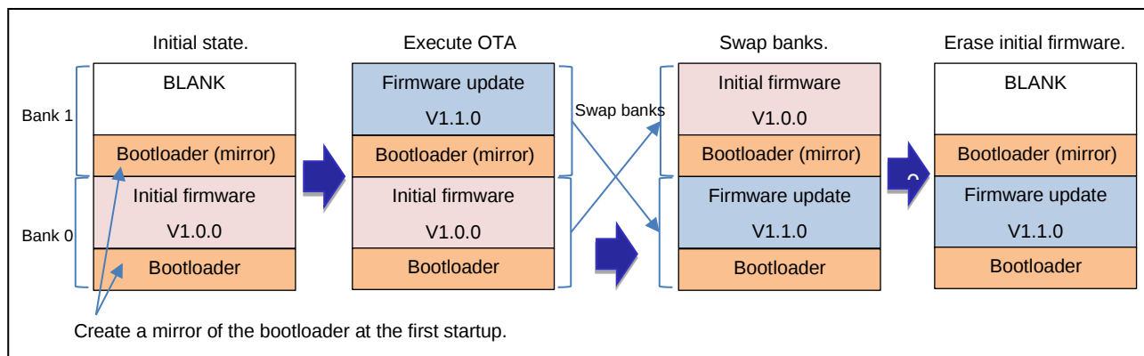
Figure 4-1 OTA Image
