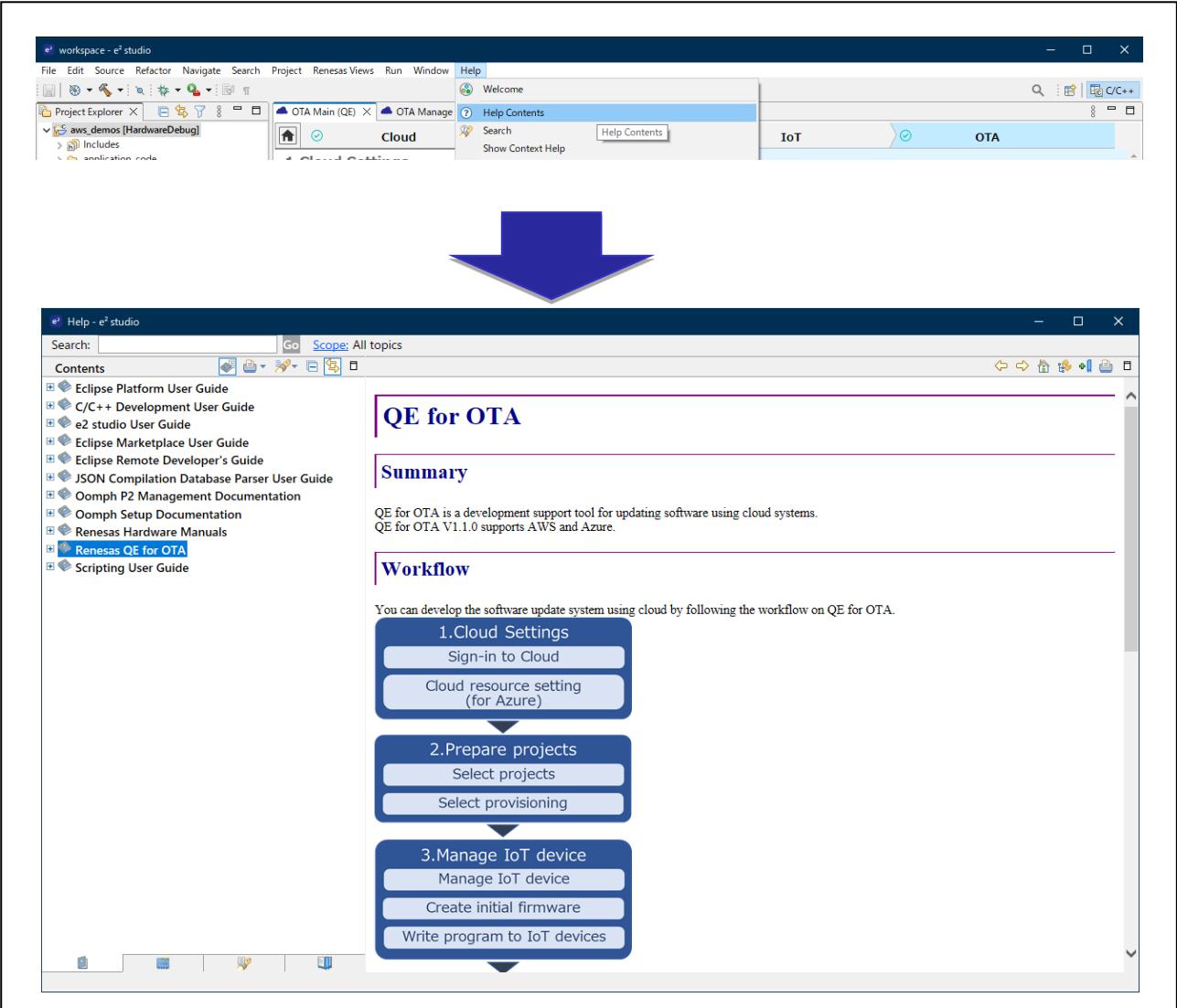
Figure 5-1 Help Function
