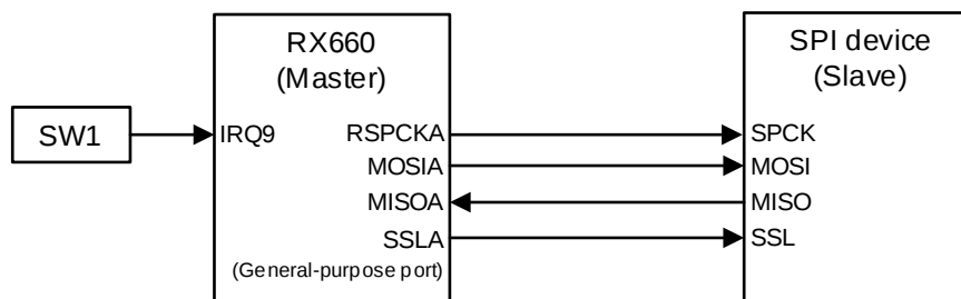
Figure 2.1 Hardware Configuration
