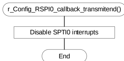
Figure 4.7 Outline Flow of the r_Config_RSPI0_callback_transmitend() Function
