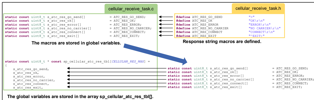
Figure 12. How response string macros are stored
