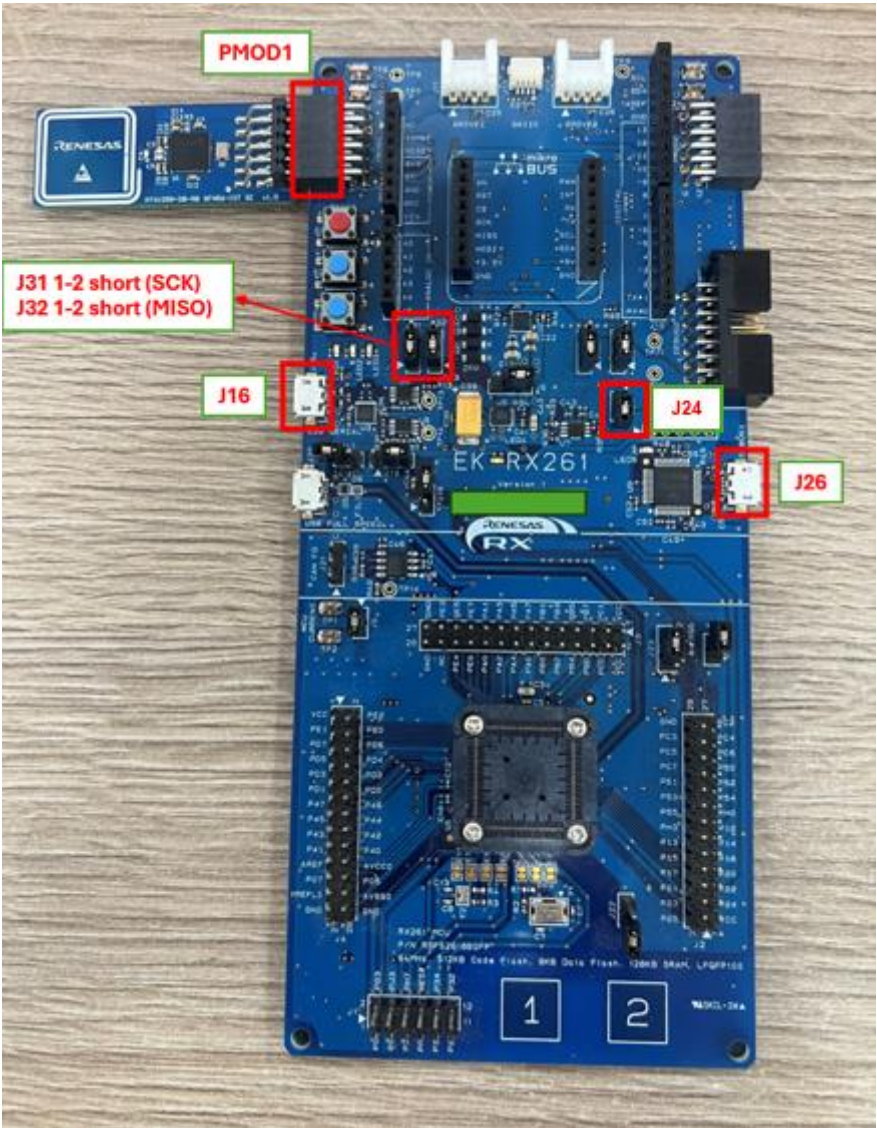
Figure 4.1 Hardware Setup
