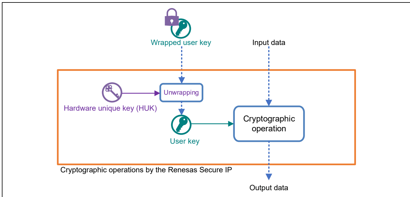
Figure 3-2 How Keys are Handled during Cryptographic Operations by the RSIP CM Driver
