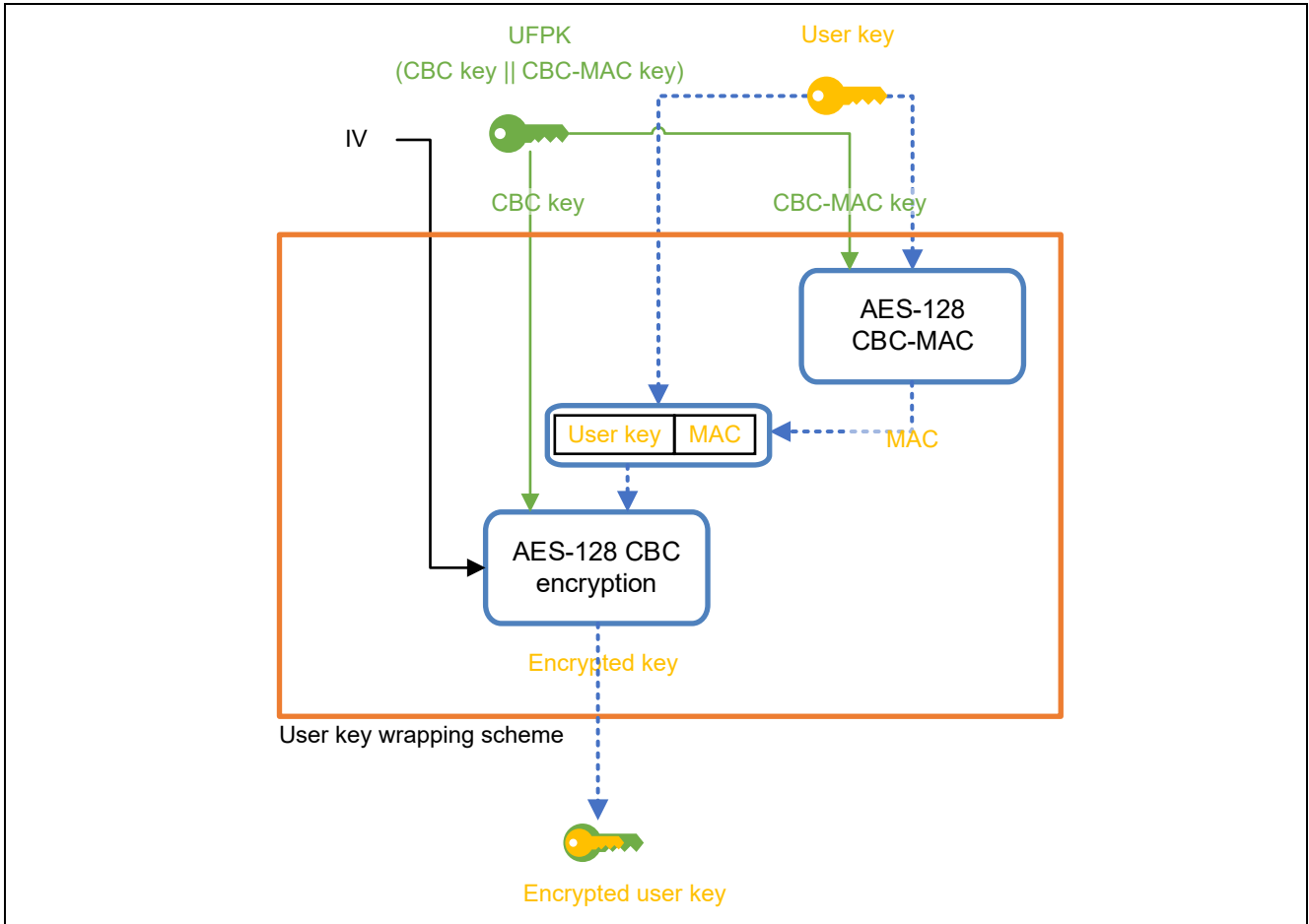
Figure 3-4 User Key Wrapping Scheme during Key Injection
