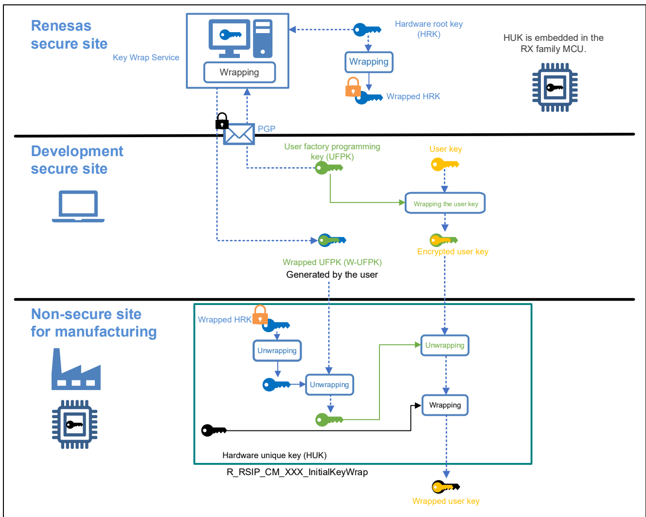
Figure 3-3 Key Injection by Using Encrypted Keys
