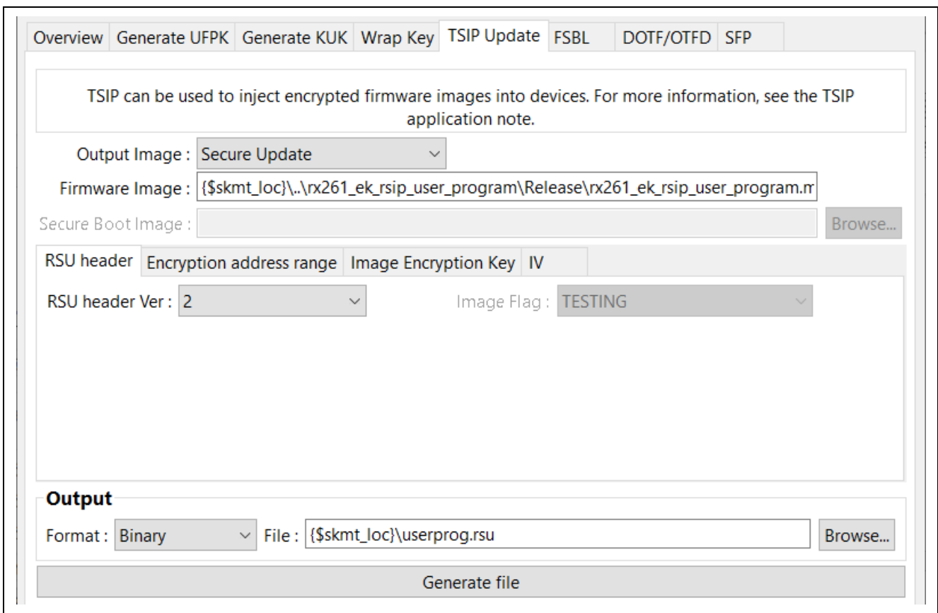
Figure 6.14 Generating an Encrypted File (TSIP UPDATE Tab – RSU header Tab)
