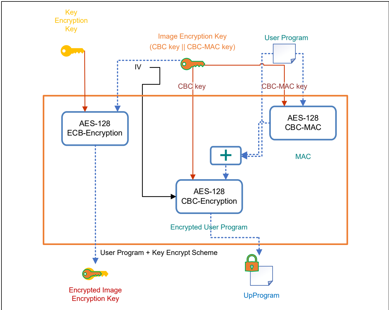
Figure 3.10 Firmware and Session Key Encryption Method
