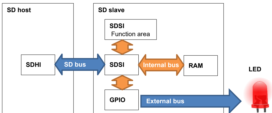
Figure 5-1 Block Diagram
