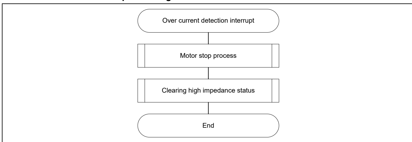
Figure 3-10 Over Current Detection Interrupt Handling
