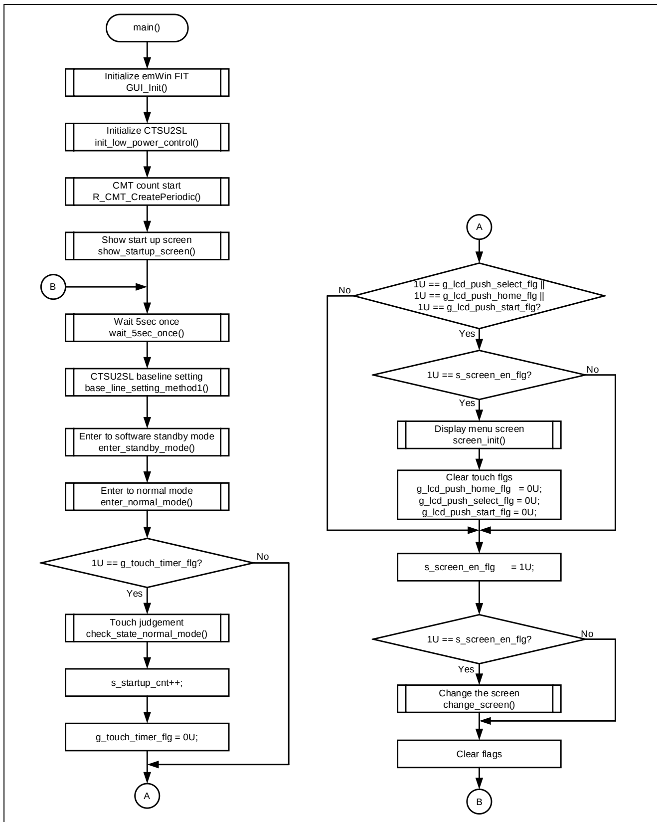
Figure 3-4 Overall flowchart
