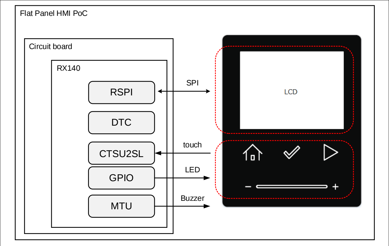
Figure 1-2 System configuration
