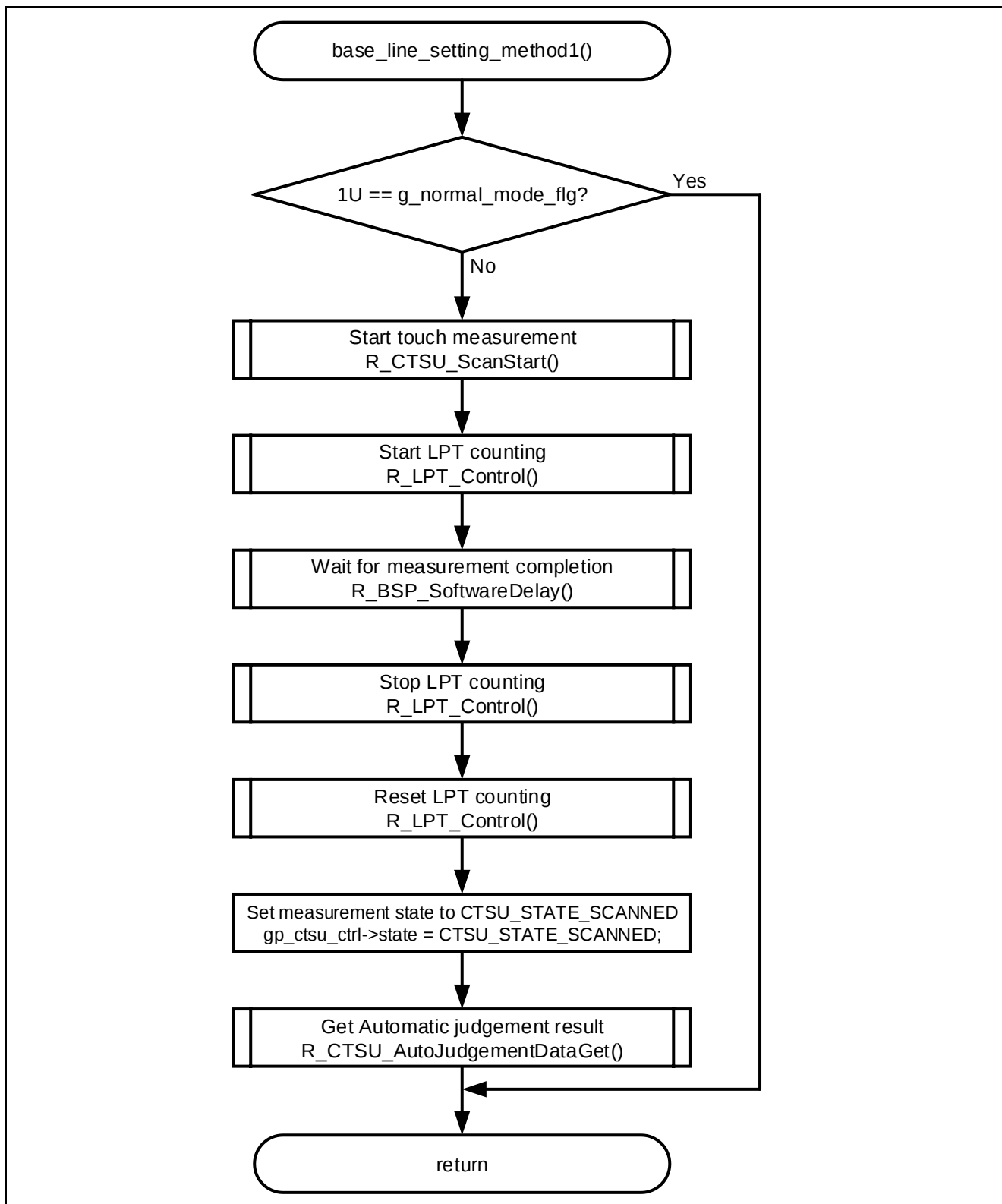
Figure 3-11 Flowchart of CTSU2SL baseline settings
