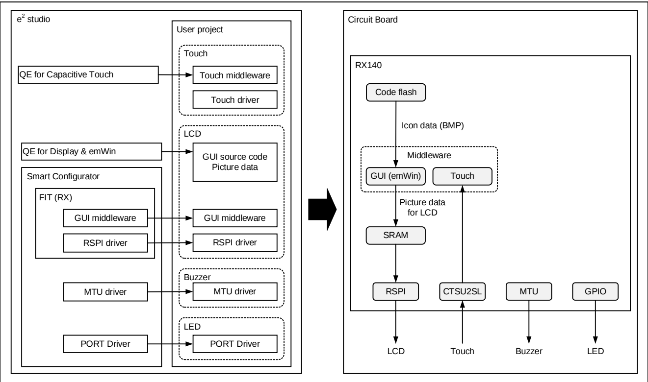
Figure 1-3 Software configuration
