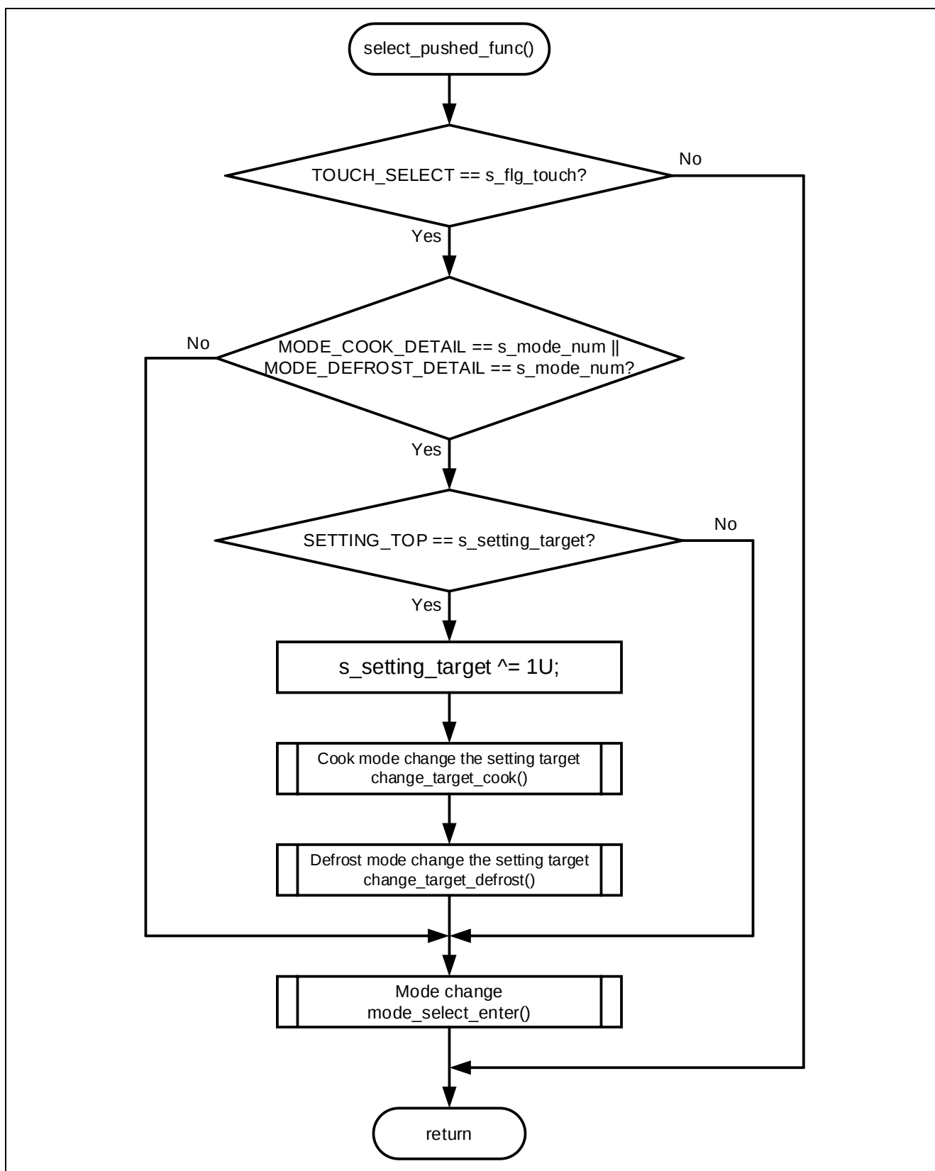
Figure 3-8 Flowchart when the "select" button is touched
