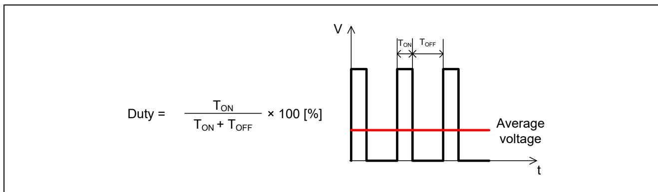
Figure 3-2 PWM Control
