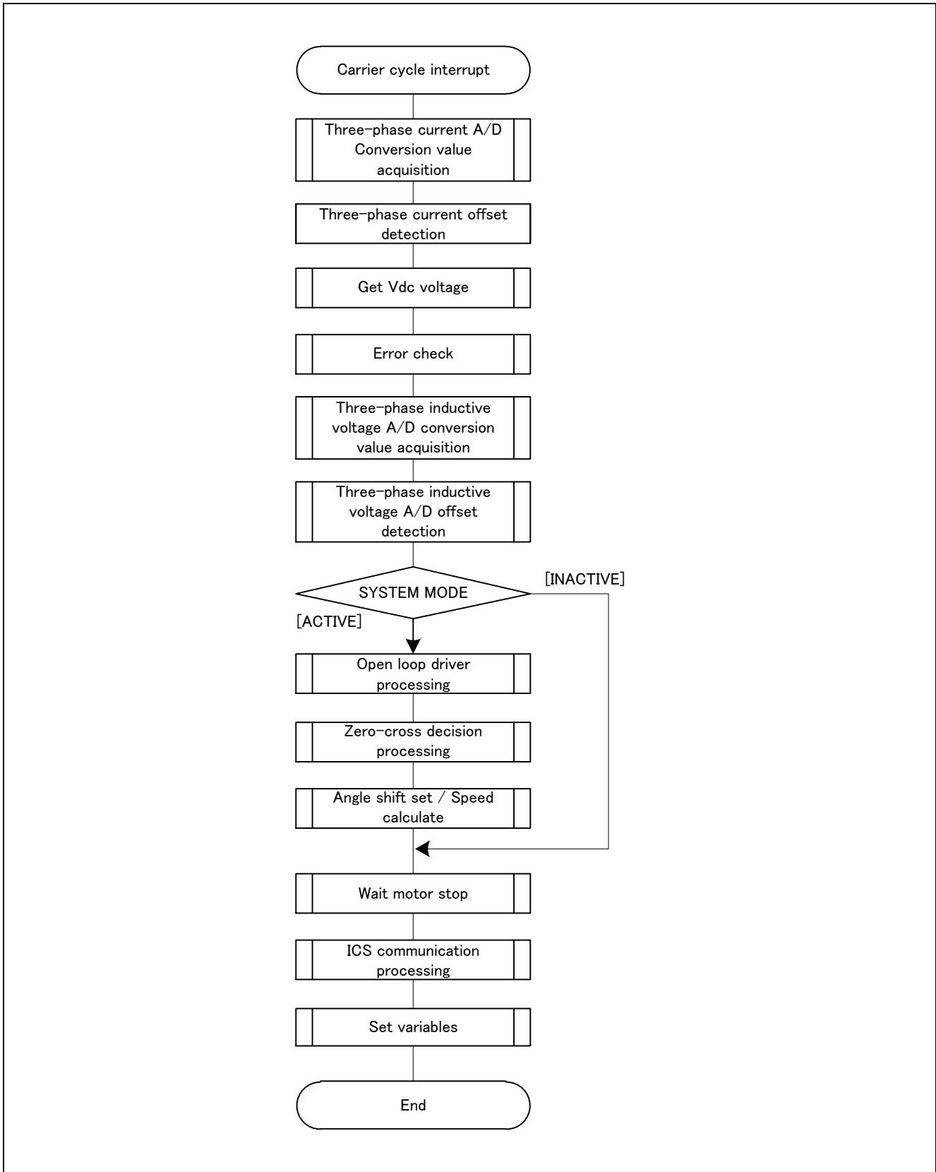
Figure 3-8 50 [μs] Cycle Interrupt Handling
