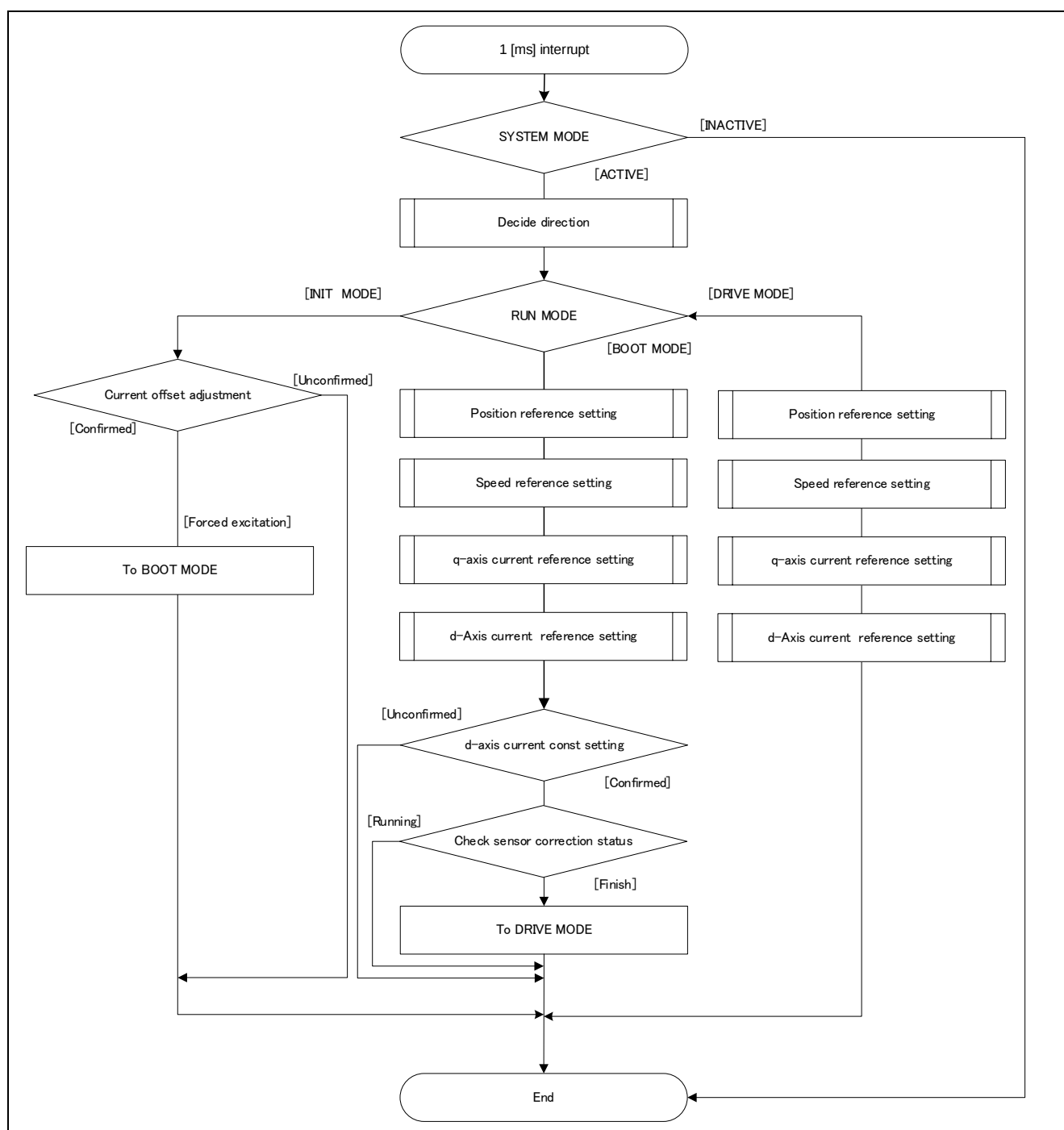
Figure 3-17 1 [ms] Interrupt Handling
