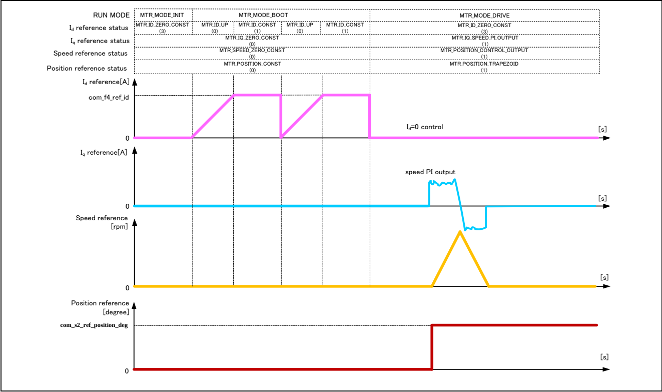
Figure 3-8 Startup Position Control of Vector Control PMSM with digital Magnet sensor Software
