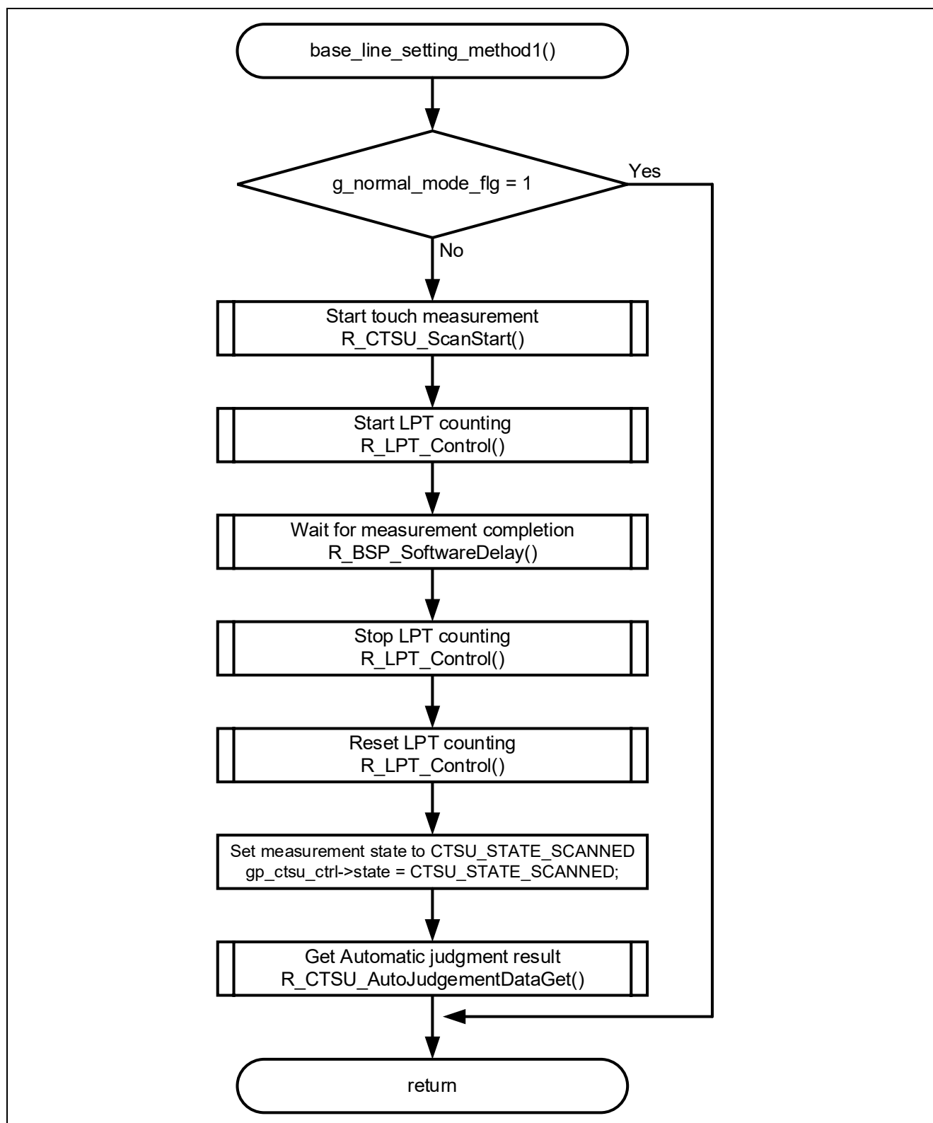
Figure 4-11 Flowchart of CTSU2SLa baseline settings
