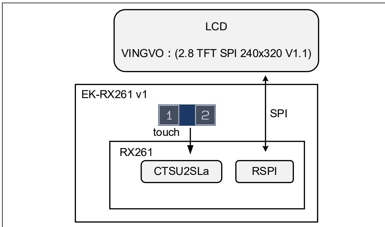
Figure 1-1 System configuration
