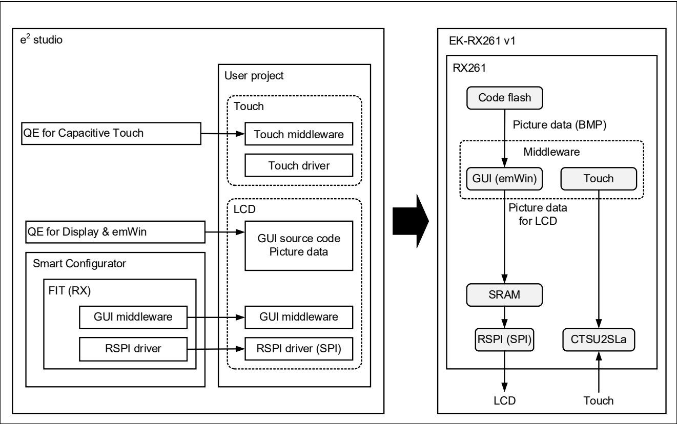
Figure 1-2 Software configuration
