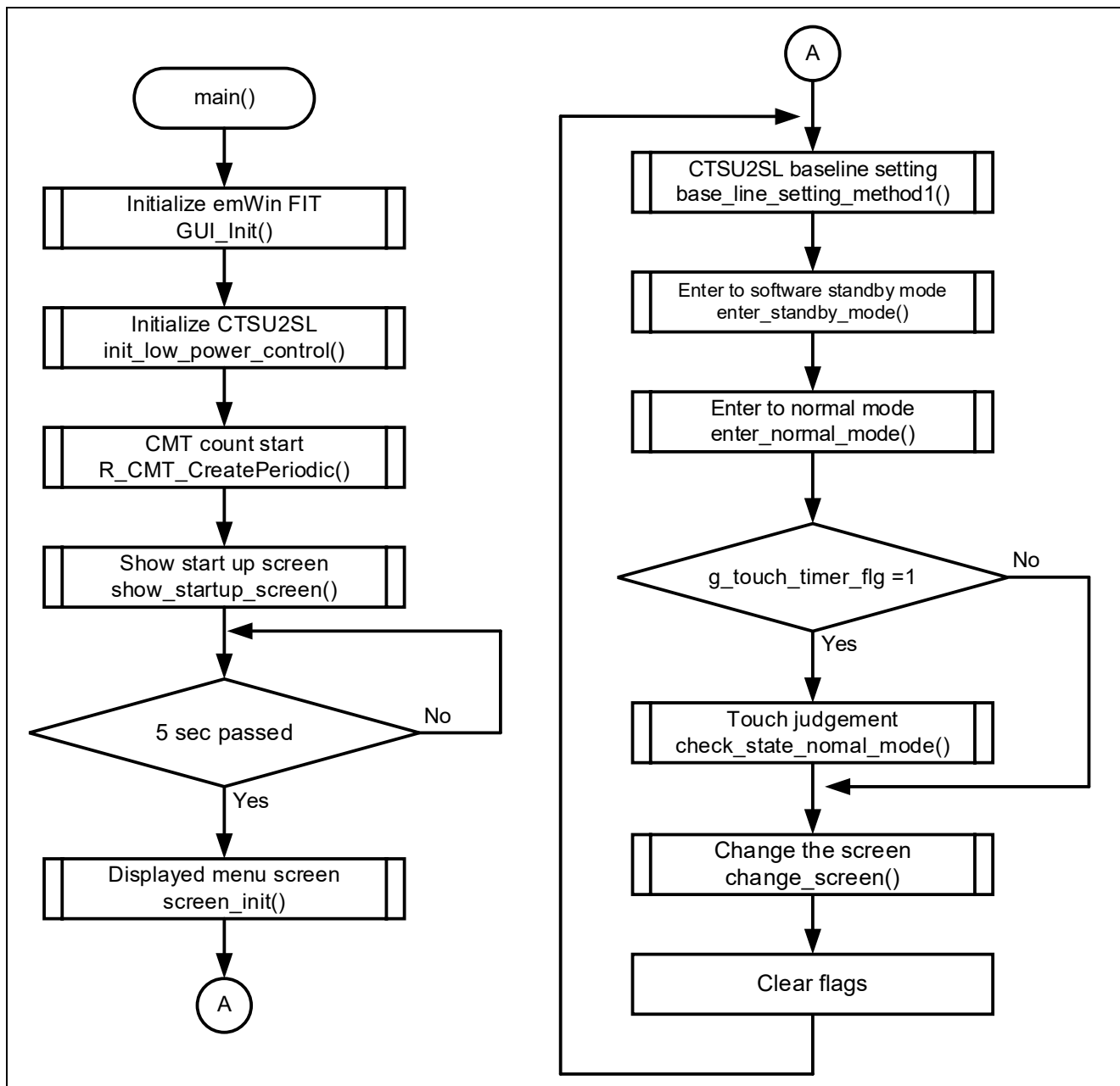
Figure 4-4 Overall flowchart
