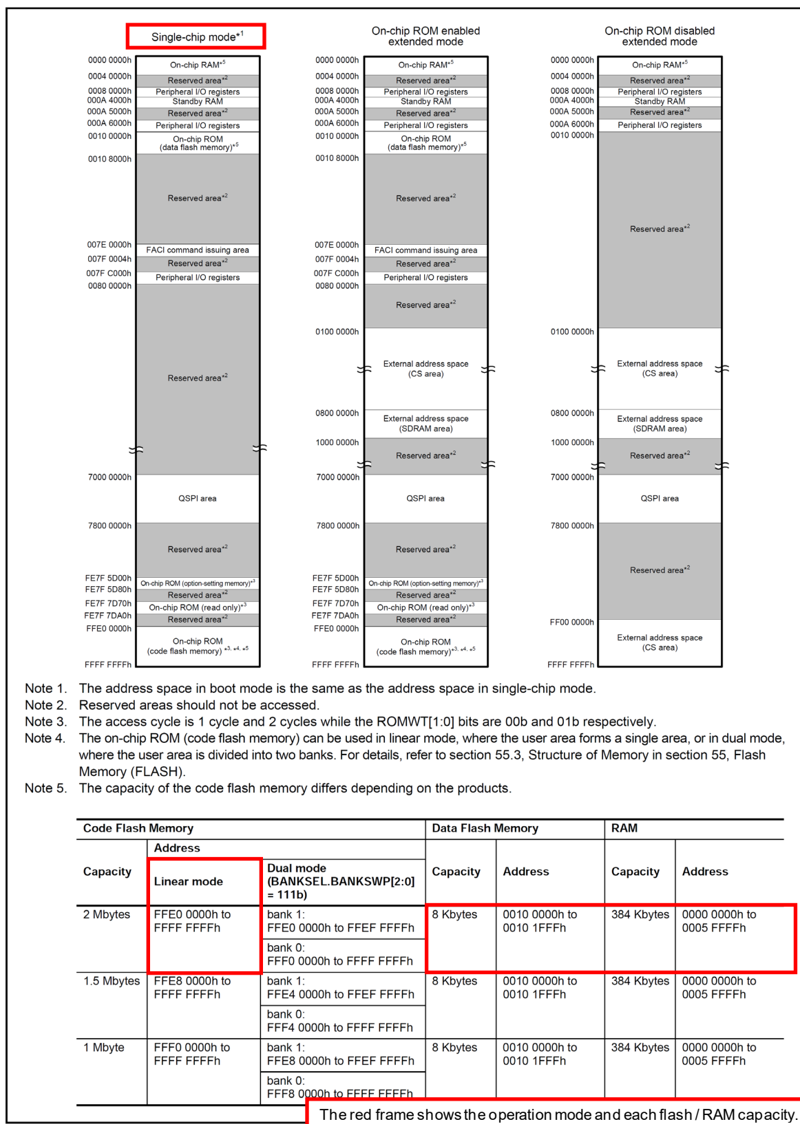
Figure 4-1: RX671 Memory map
