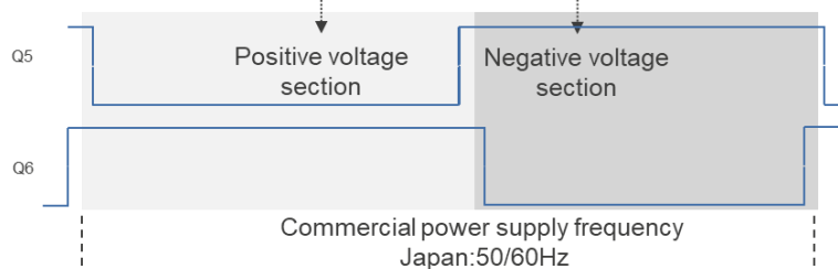
Figure 4 Totem Pole PFC (interleaved) operation and switching waveforms
