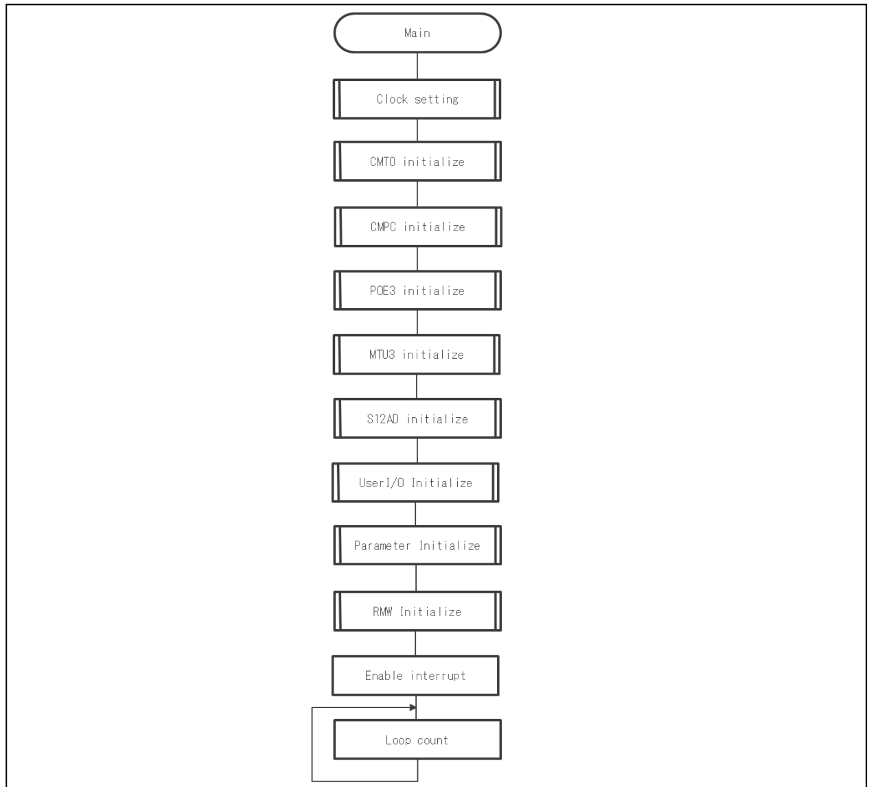
Figure 15 Main Process
