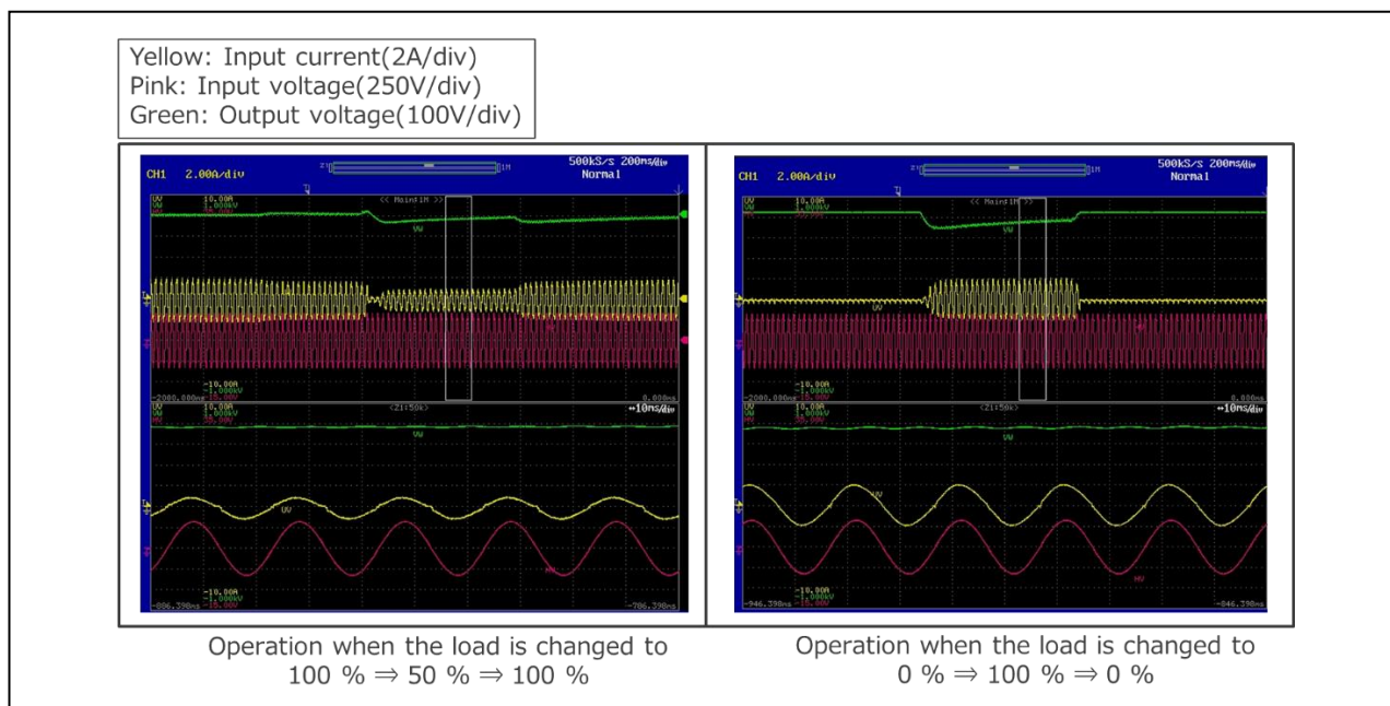
Figure 27 Output-Waveform at Load Variation
