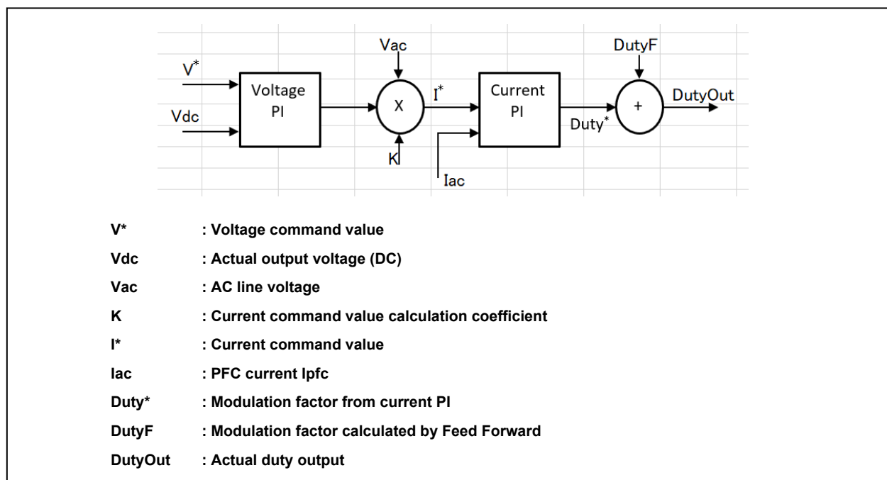
Figure 14 AC-DC Control Logic Diagram
