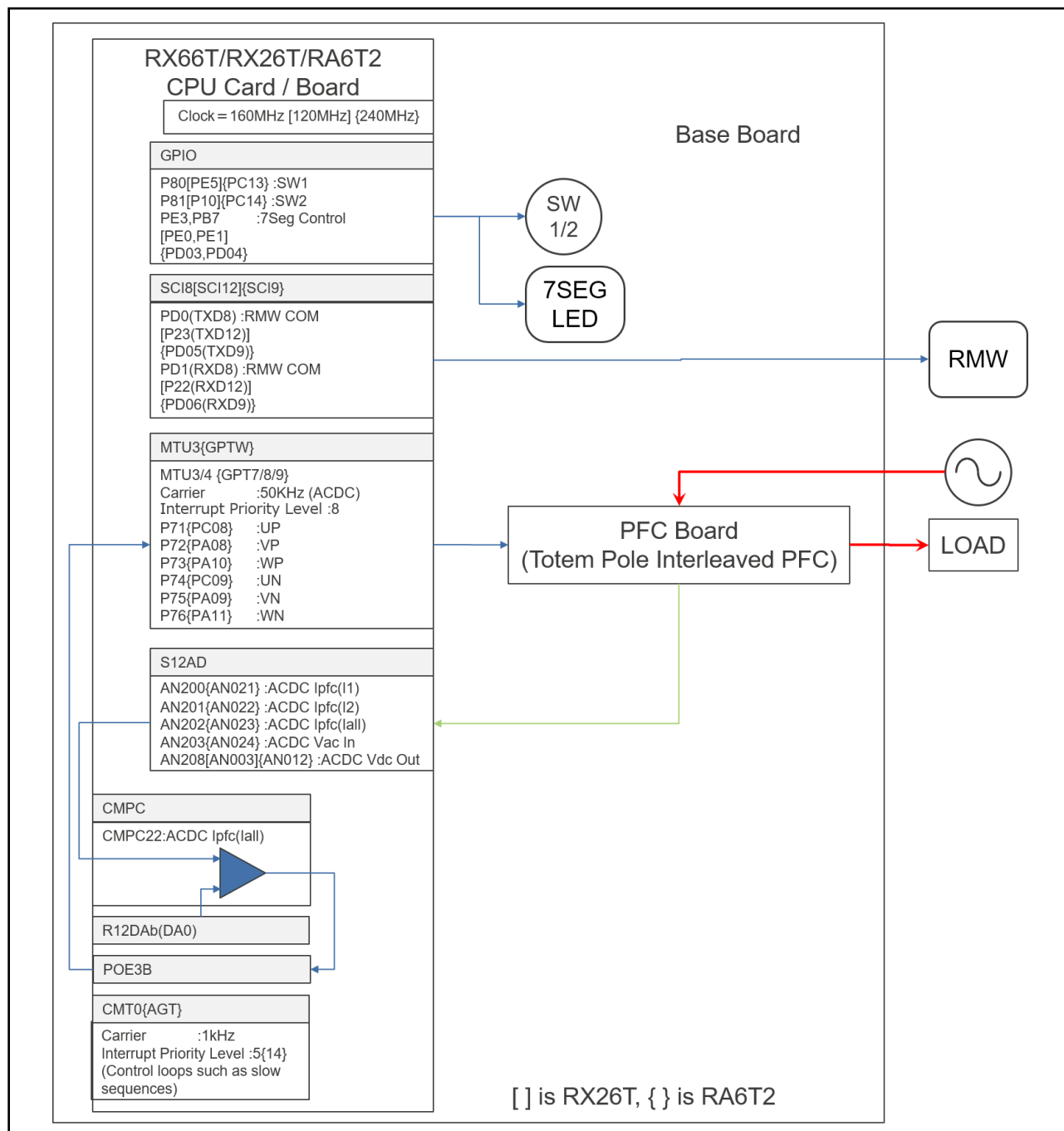
Figure 10 MCU Function Connection Configuration Diagram
