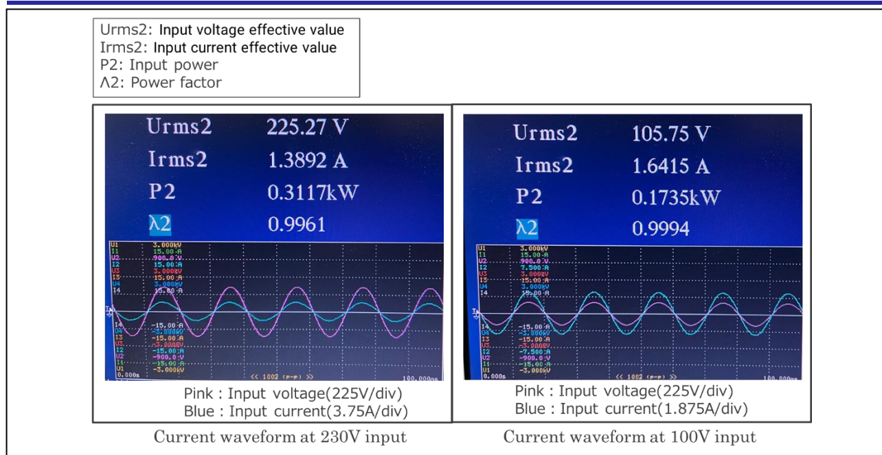
Figure 26 Current wave form when inputting 230V/100V
