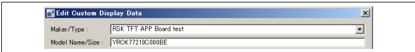
Figure 5.8 Name Registration
