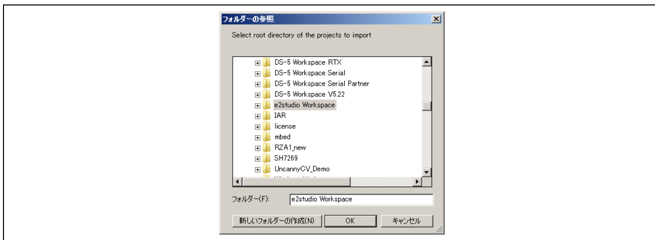
Figure 5.3 Browse Folders
