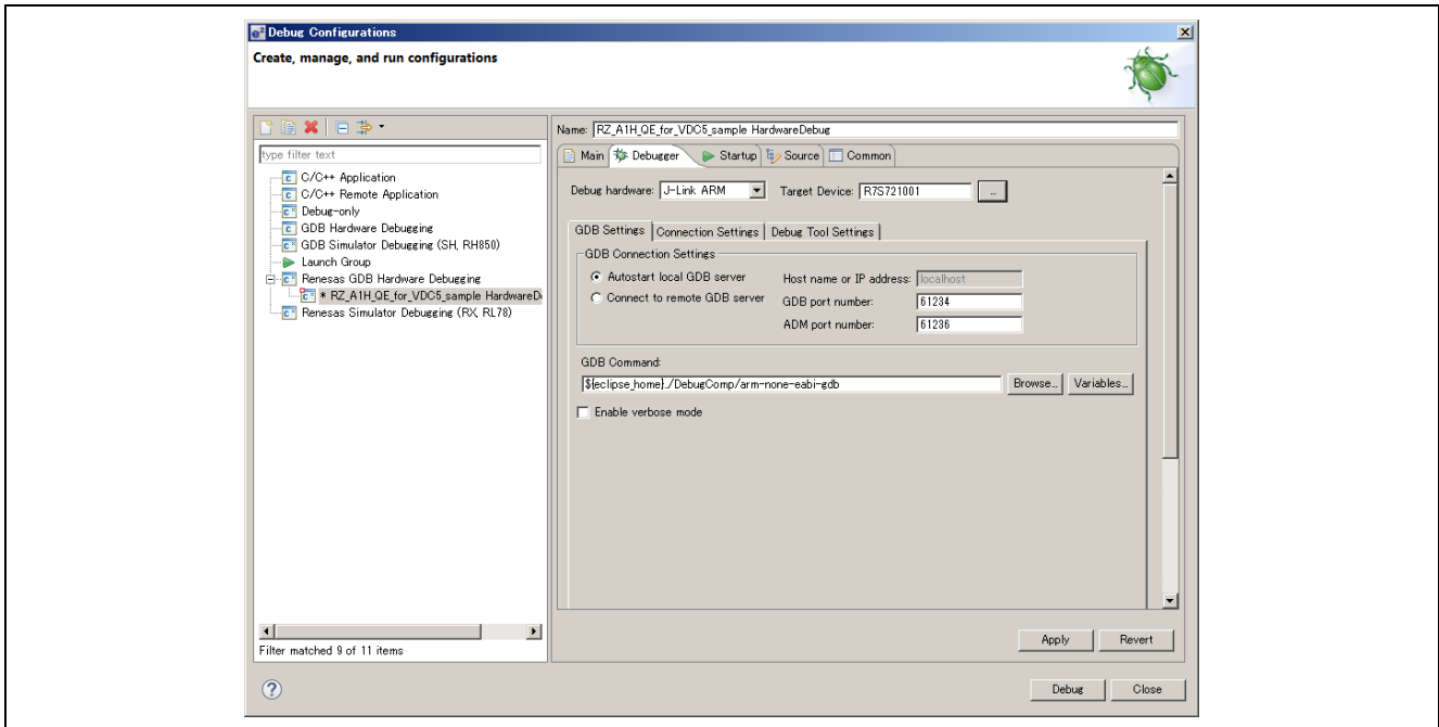
Figure 5.20 Debugger Settings
