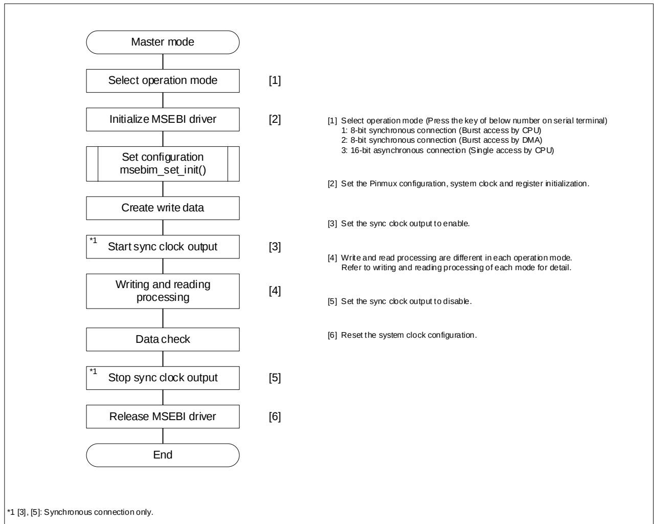
Figure 5.1 Main processing of MSEBI master
