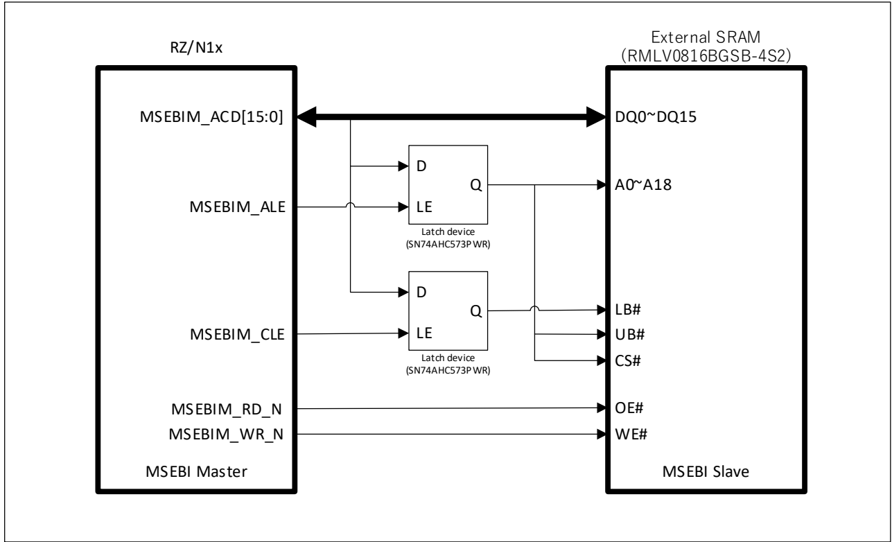
Figure 1.2 Block diagram (16-bit asynchronous connection)
