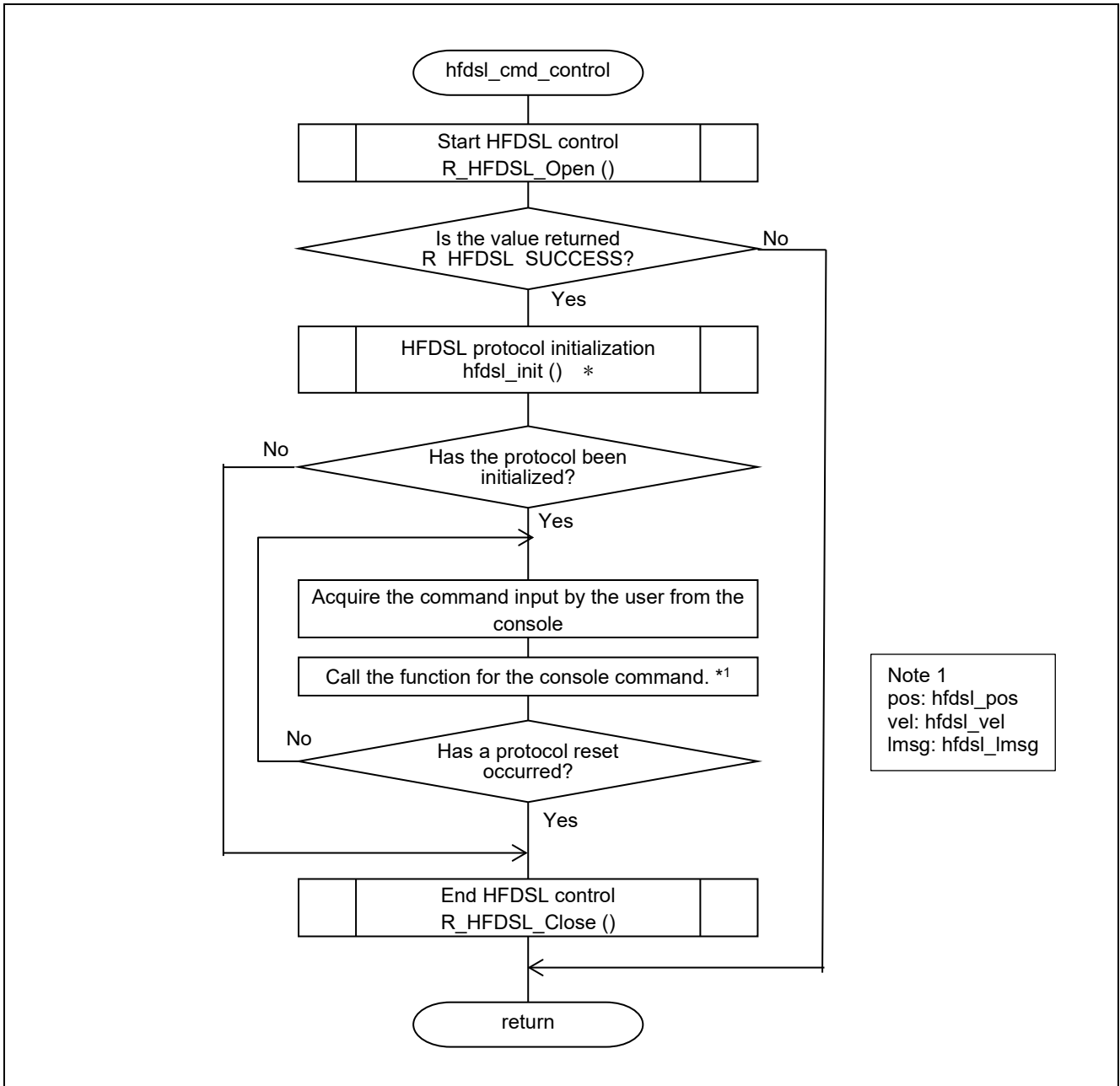
Figure 4.5 Flowchart hfdsl_cmd_control
