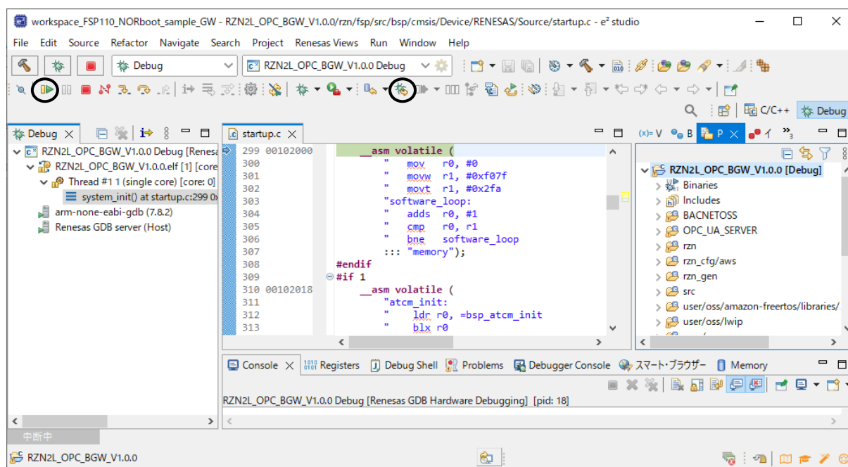
Fig.4-17 Break at system_init()
