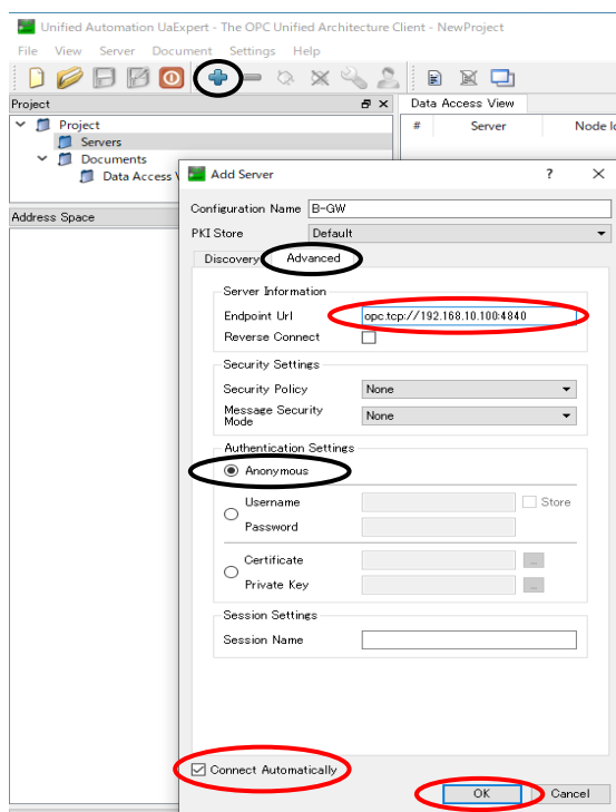
Fig.4-20 UaExpert Add server
