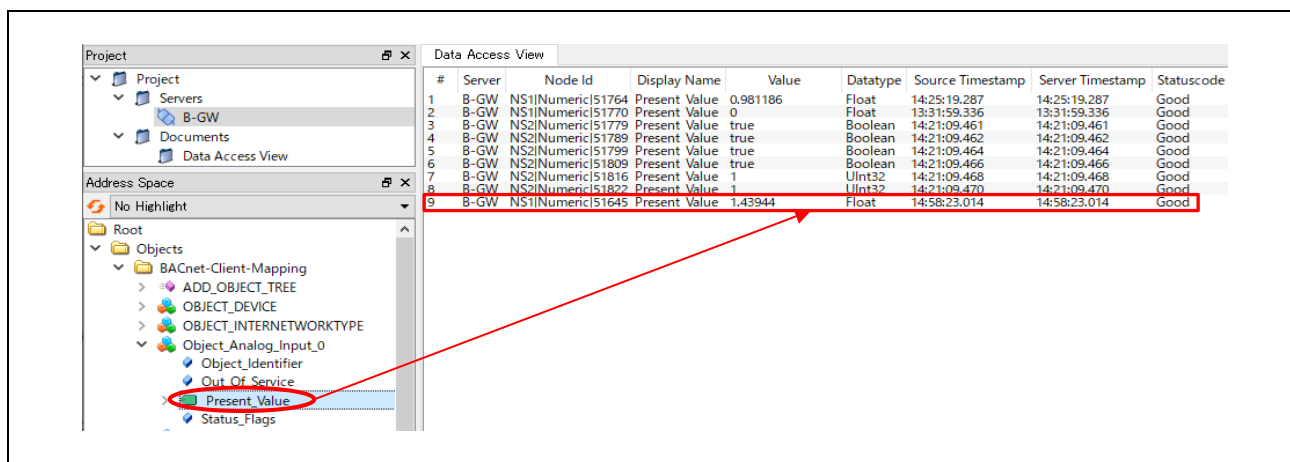
Fig.4-47 B-SS pseudo input value reading
