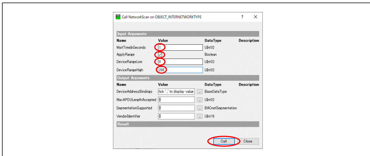
Fig.4-27 UaExpert OPC UA NetworkScan Method call(2)
