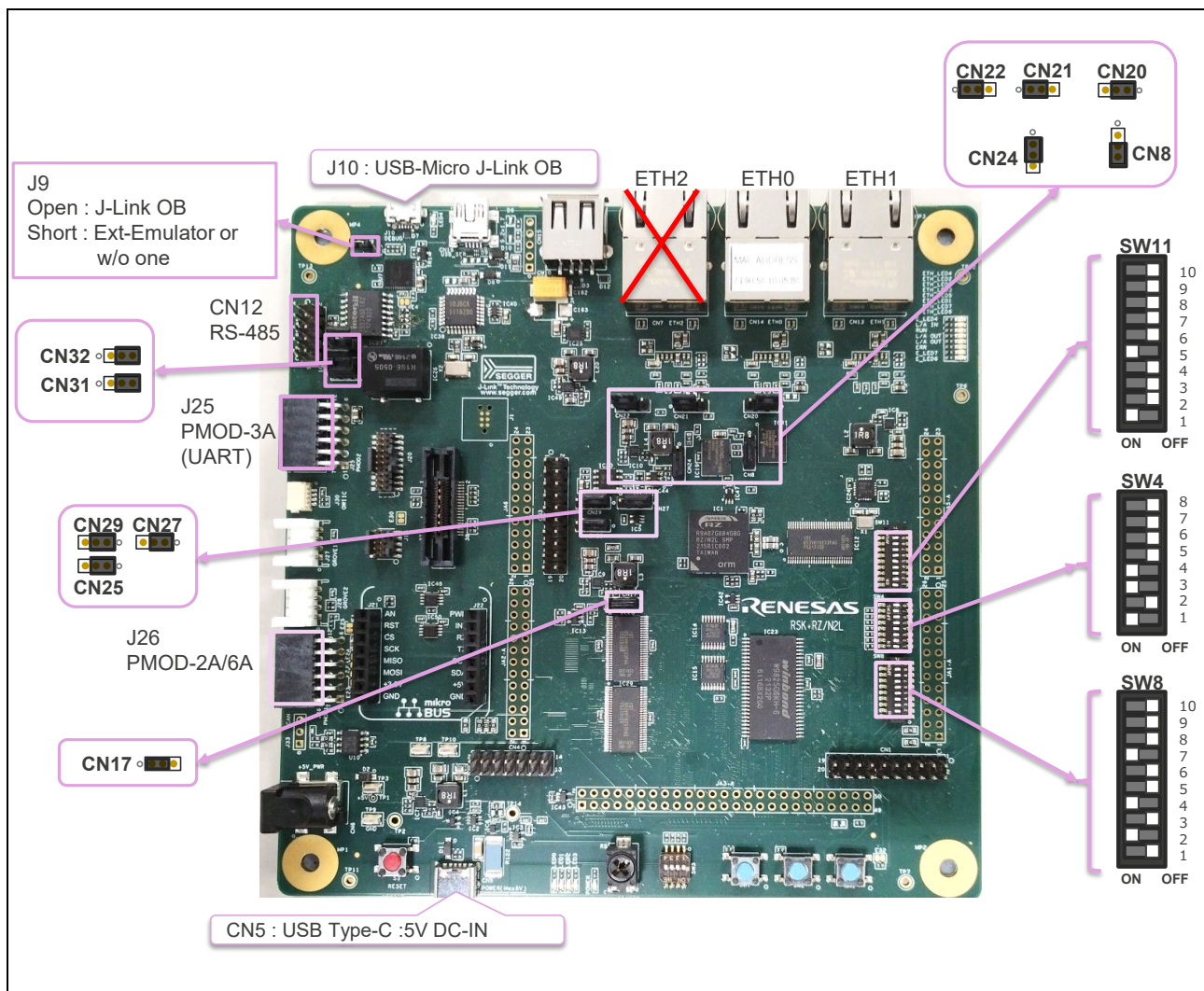
Fig. 2-1 Board Configuration
