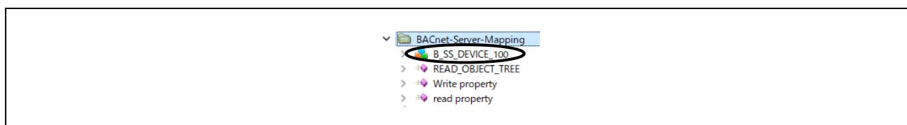
Fig.4-41 UaExpert OPC UA ADD_OBJECT_TREE Method call(4)
