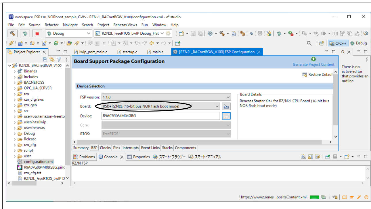
Fig.3-2 Boot mode
