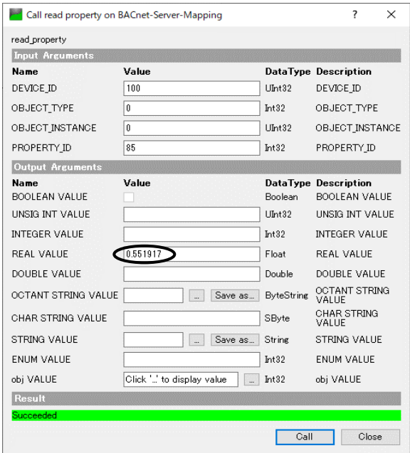
Fig.4-36 UaExpert OPC UA Read property Method call(3)
