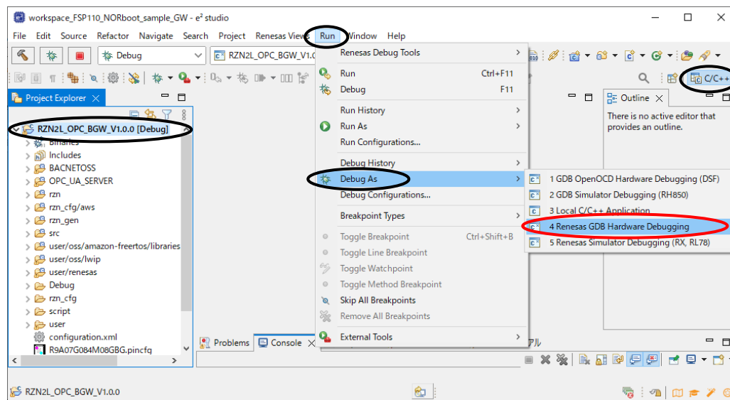
Fig.4-14 Run menu Debug As
