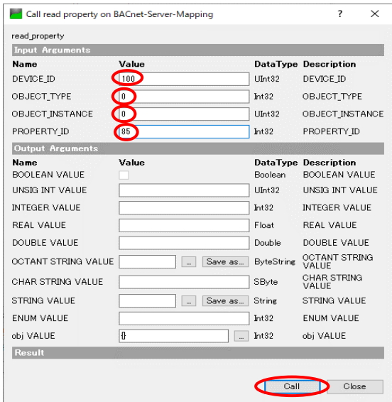
Fig.4-35 UaExpert OPC UA Read property Method call(2)
