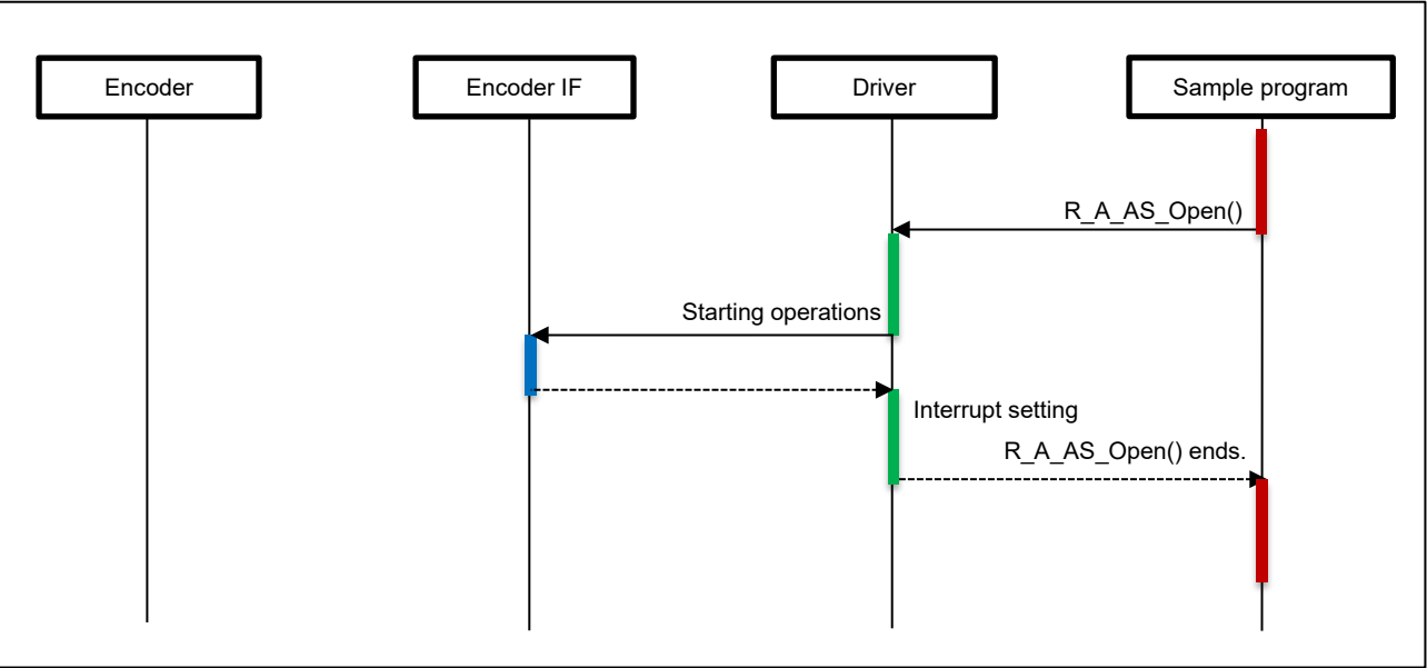
Figure 4.11 Startup Sequence Diagram
