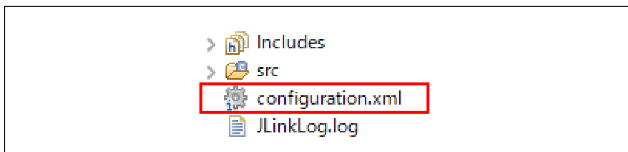
図 6.8 Configuration.xml
