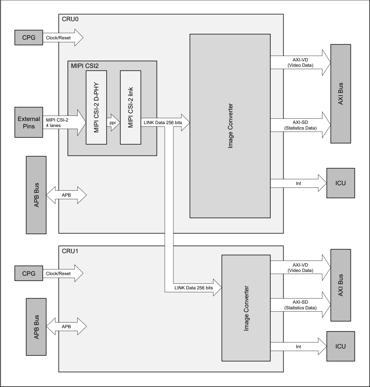
Figure 1.5 CRU0 and CRU1 Block Diagram for VC Camera Case
