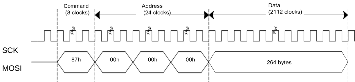
Figure 5: Transferring data to the Buffer 2 SRAM
