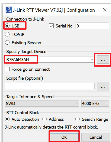
Figure 26. Launch SEGGER RTT Viewer
