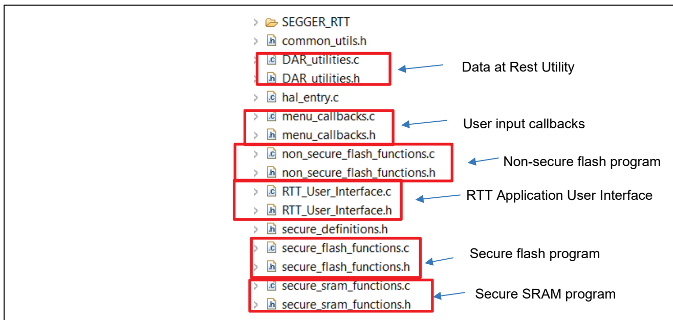
Figure 23. Source Code
