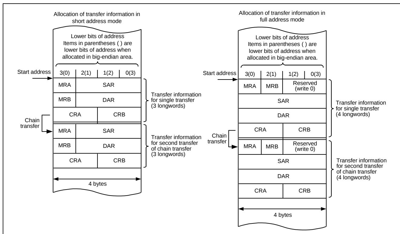
Figure 2.10 Allocation of Transfer Information
