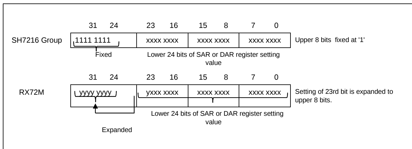
Figure 2.9 Transfer Source and Transfer Destination Addresses in Short Address Mode
