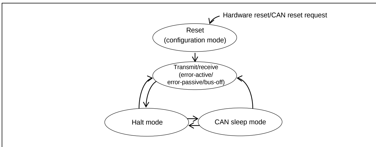
Figure 2.21 SH7216 Group State Transitions
