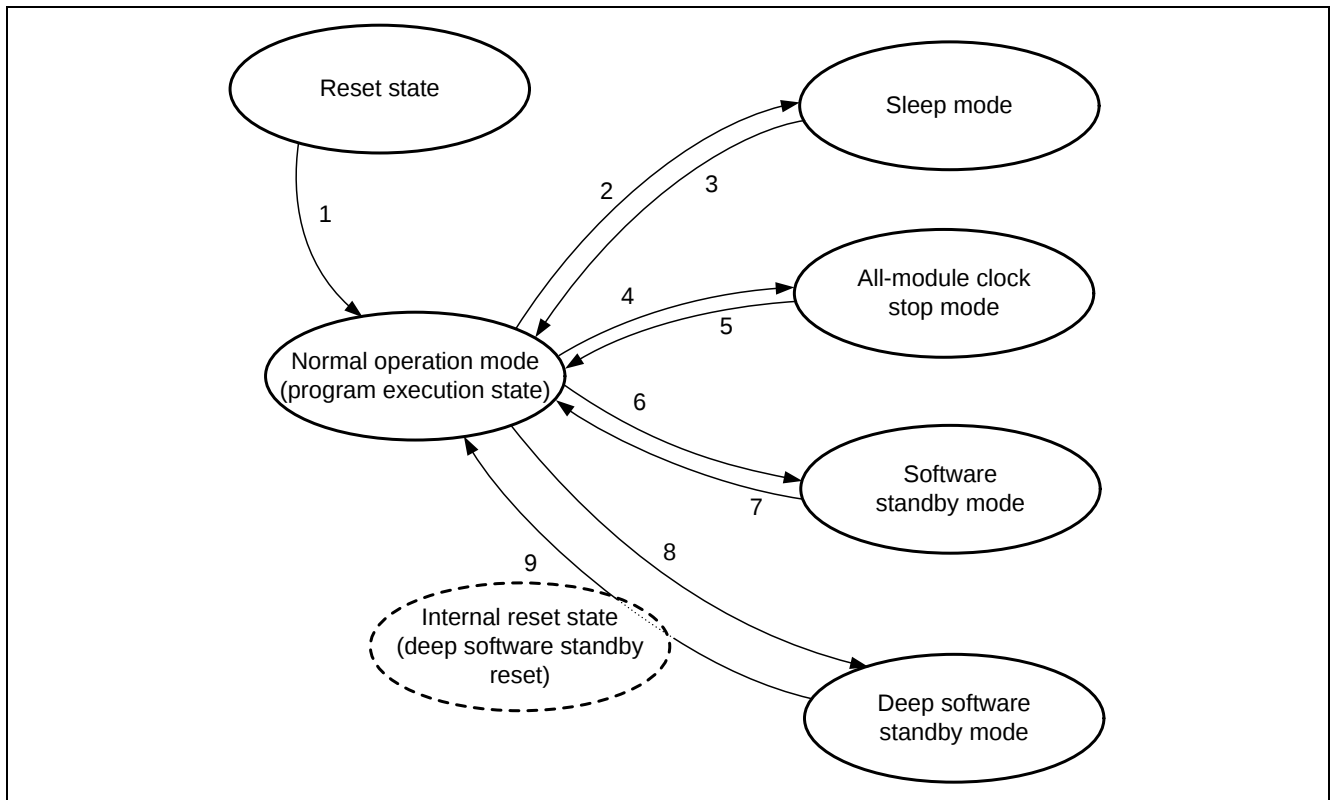
Figure 2.23 RX72M Mode Transitions
