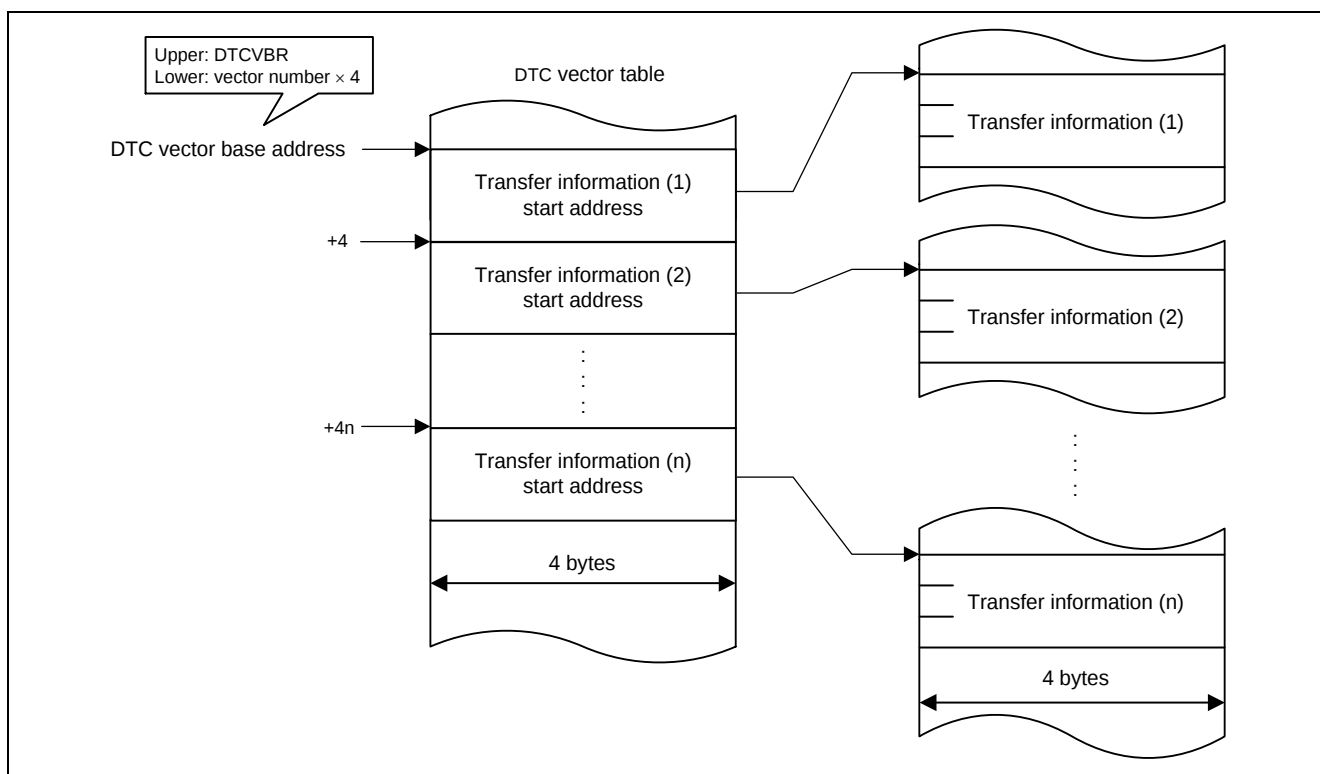
Figure 2.8 DTC Vector Configuration on RX72M
