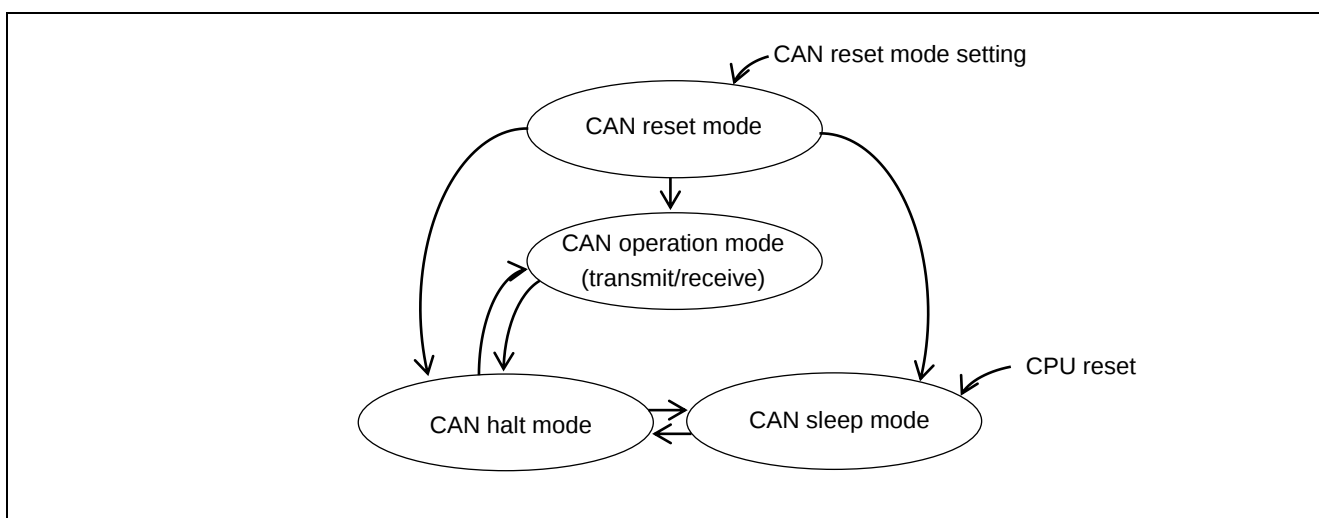
Figure 2.22 RX72M State Transitions
