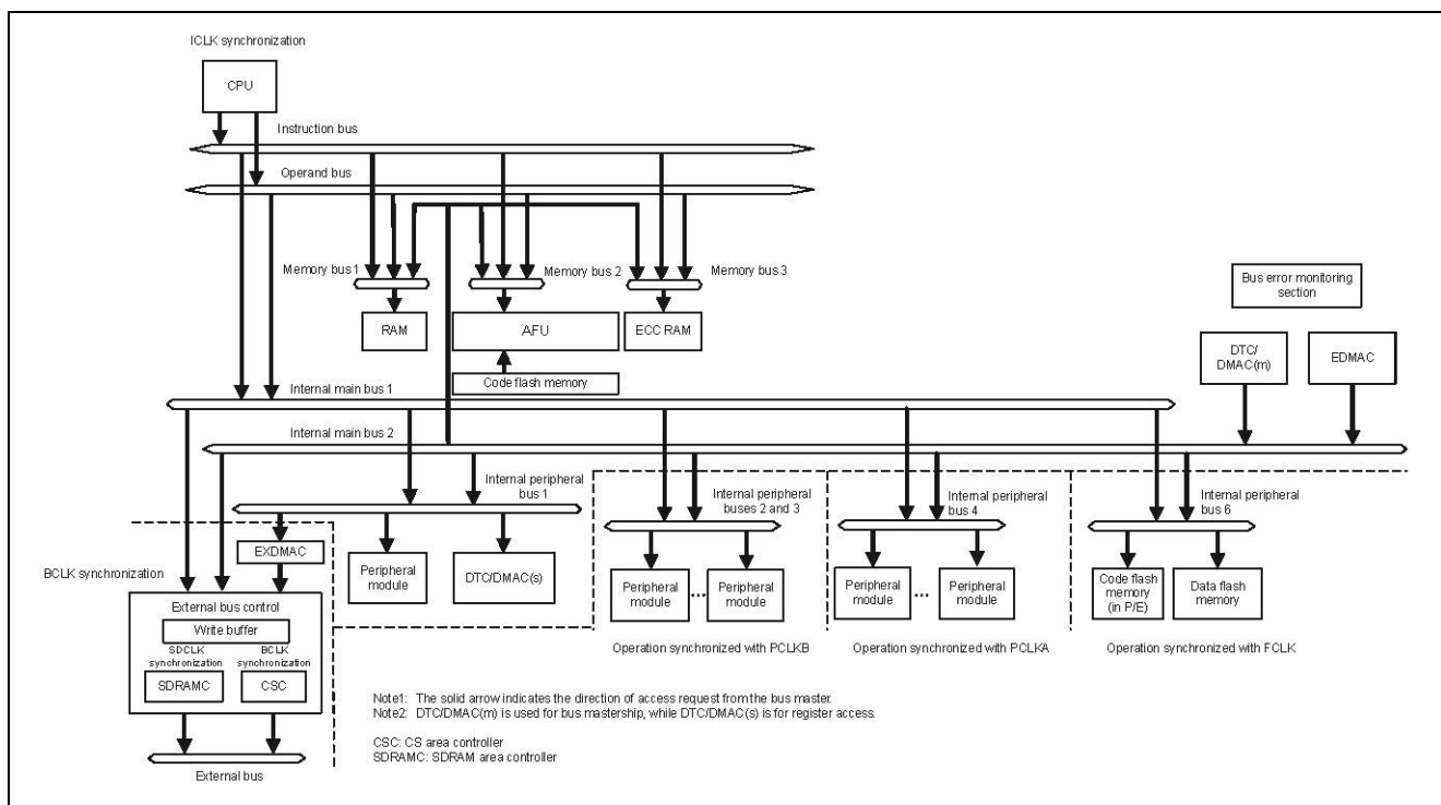
Figure 2.6 RX72M Bus Block Diagram
