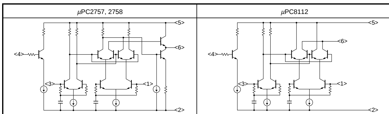
Figure 4-4. Internal Equivalent Circuits
