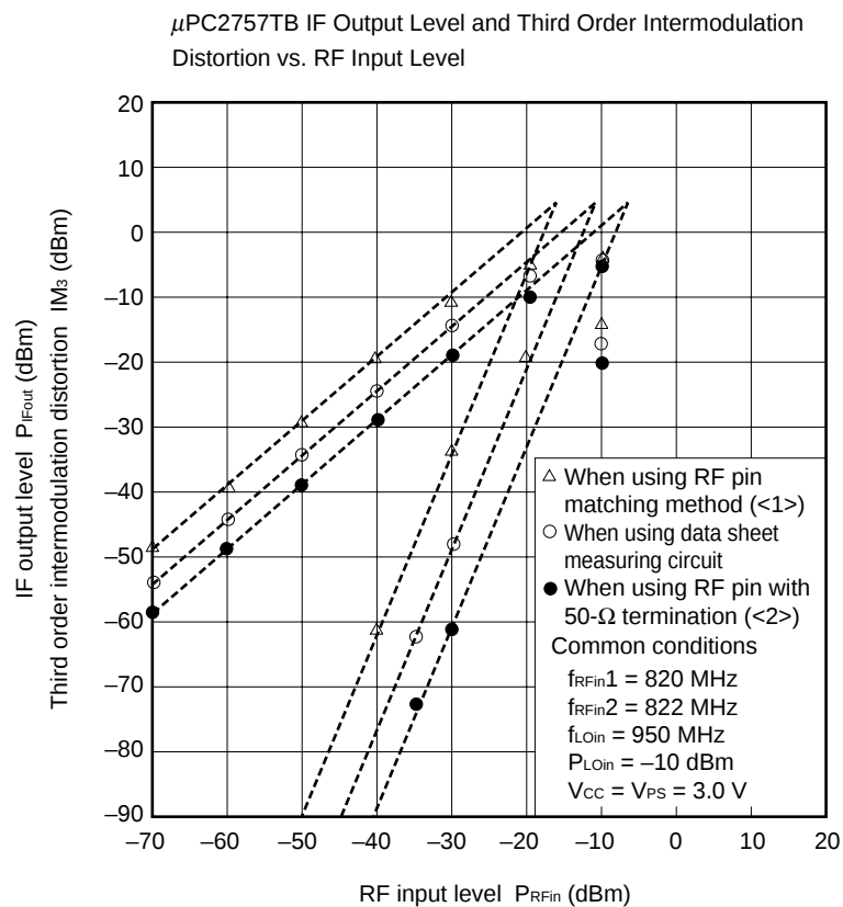
Figure 4-7. Comparison of Characteristics from External Circuit Connection to RF Pin (Super mini mold) (1/2)
