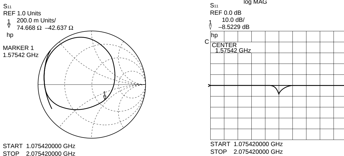
★ Figure 4-3. Input Port External Circuit Example (Example of RF Input of \mu PC2757/58) (1/2)
