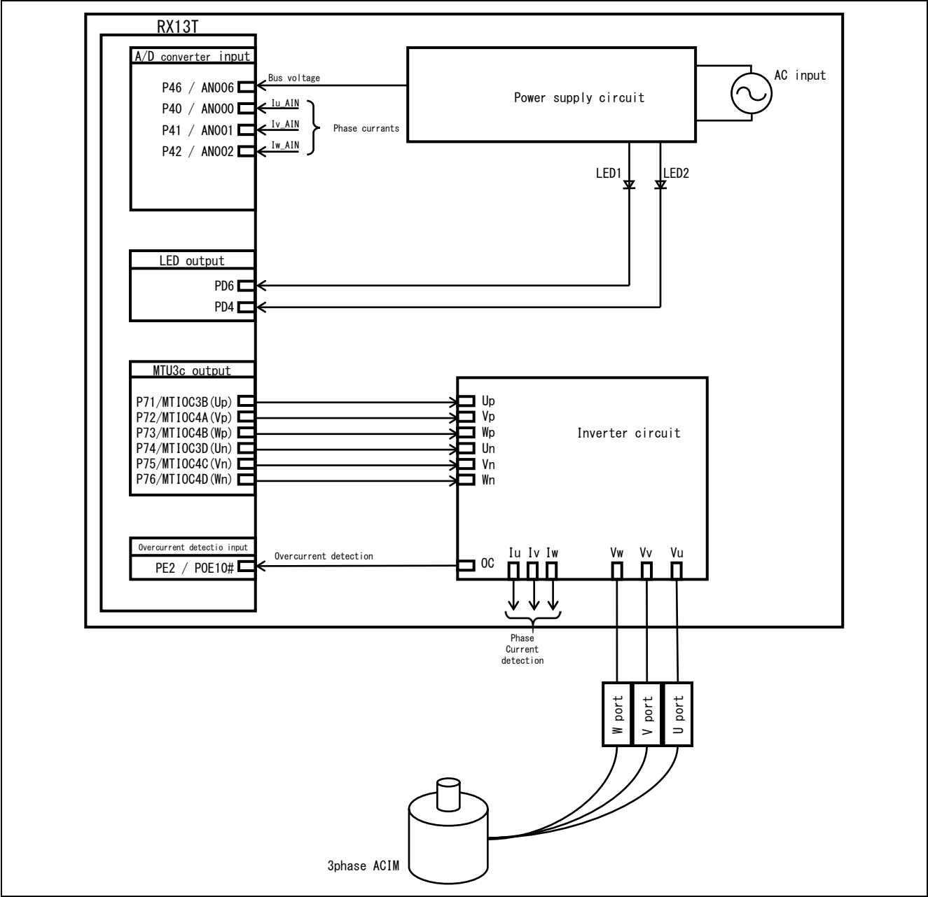
Figure 2.1 Hardware Configuration
