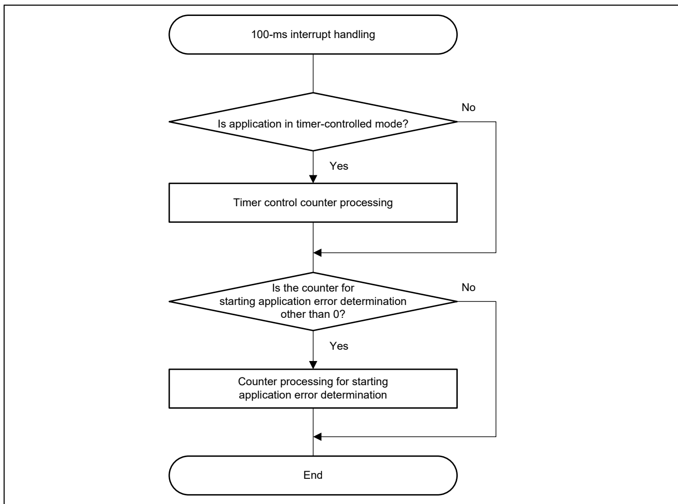
Figure 3.8 100-ms Interrupt Handling
