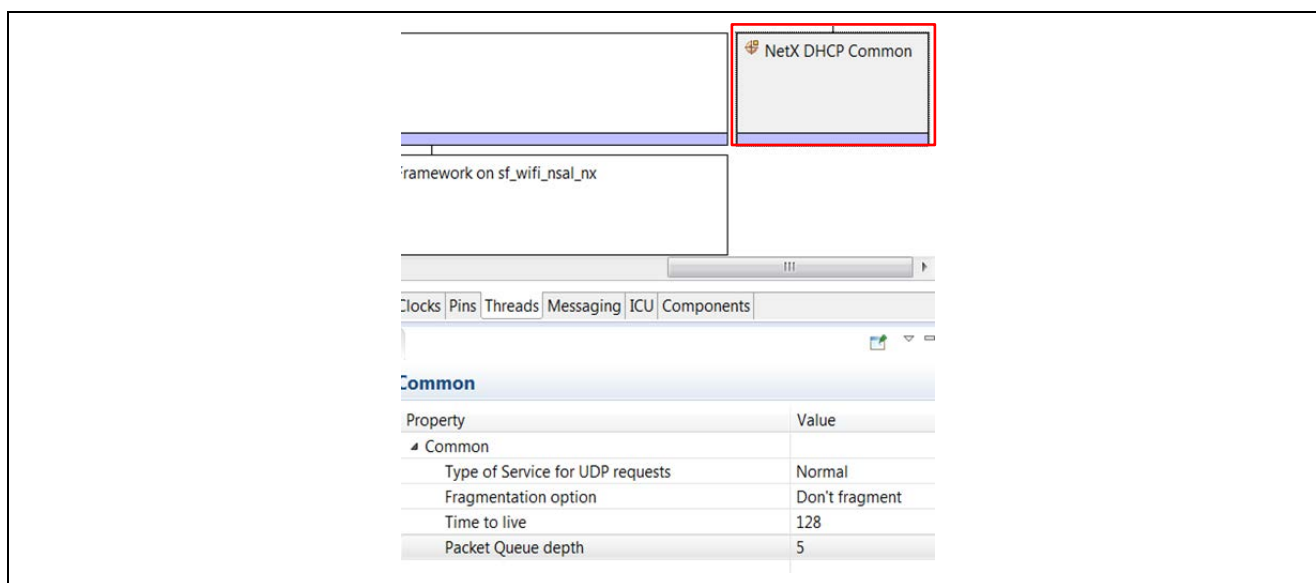
Figure 43. NetX DHCP Common configurations
