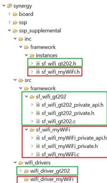
Figure 62. Setting up the Wi-Fi module driver directory file structure
