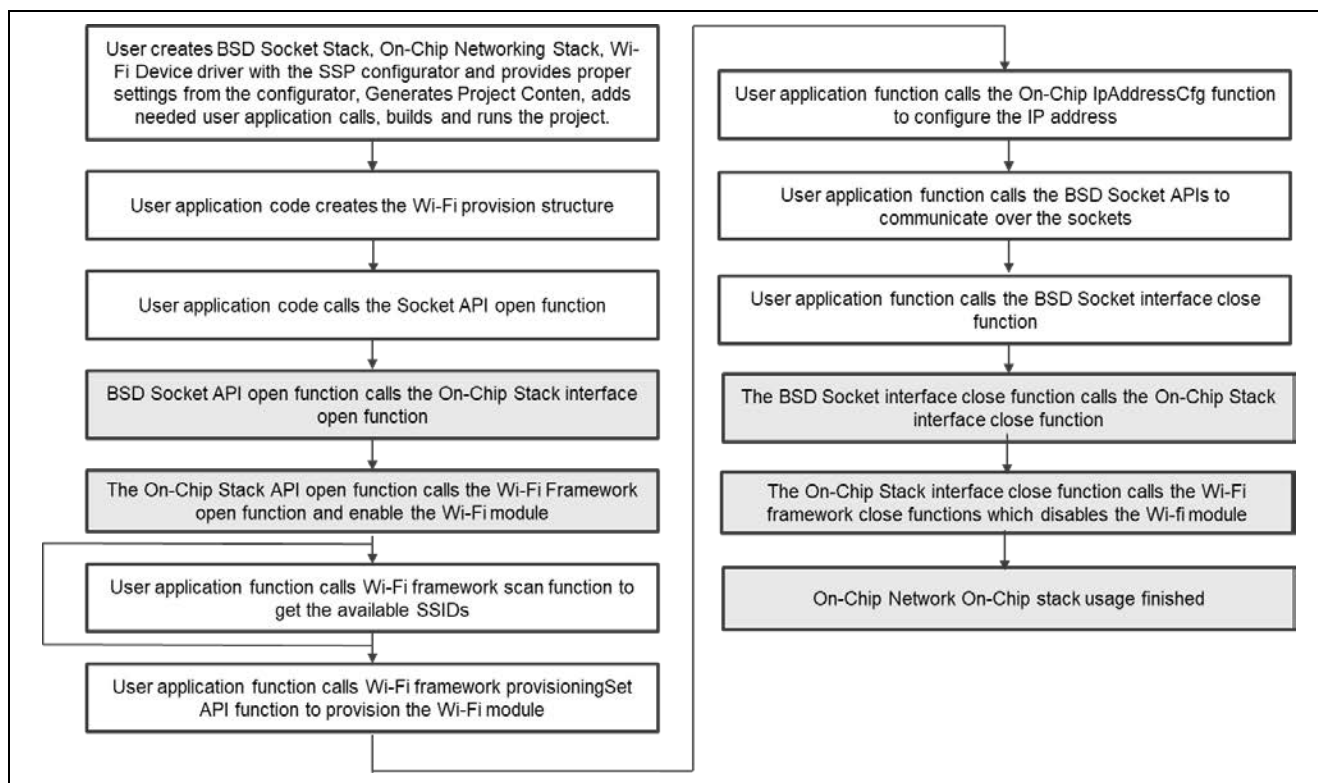
Figure 5. Wi-Fi operational flow with On-chip networking stack support
