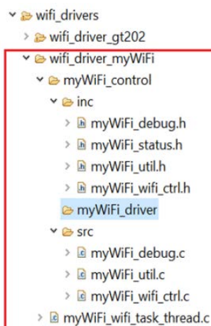
Figure 66. Custom Wi-Fi driver directory structure
