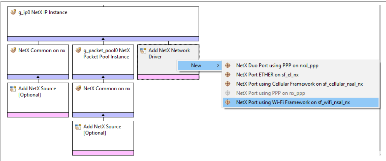
Figure 22. Adding NetX Port using Wi-Fi Framework on sf_wifi_nsal_nx
