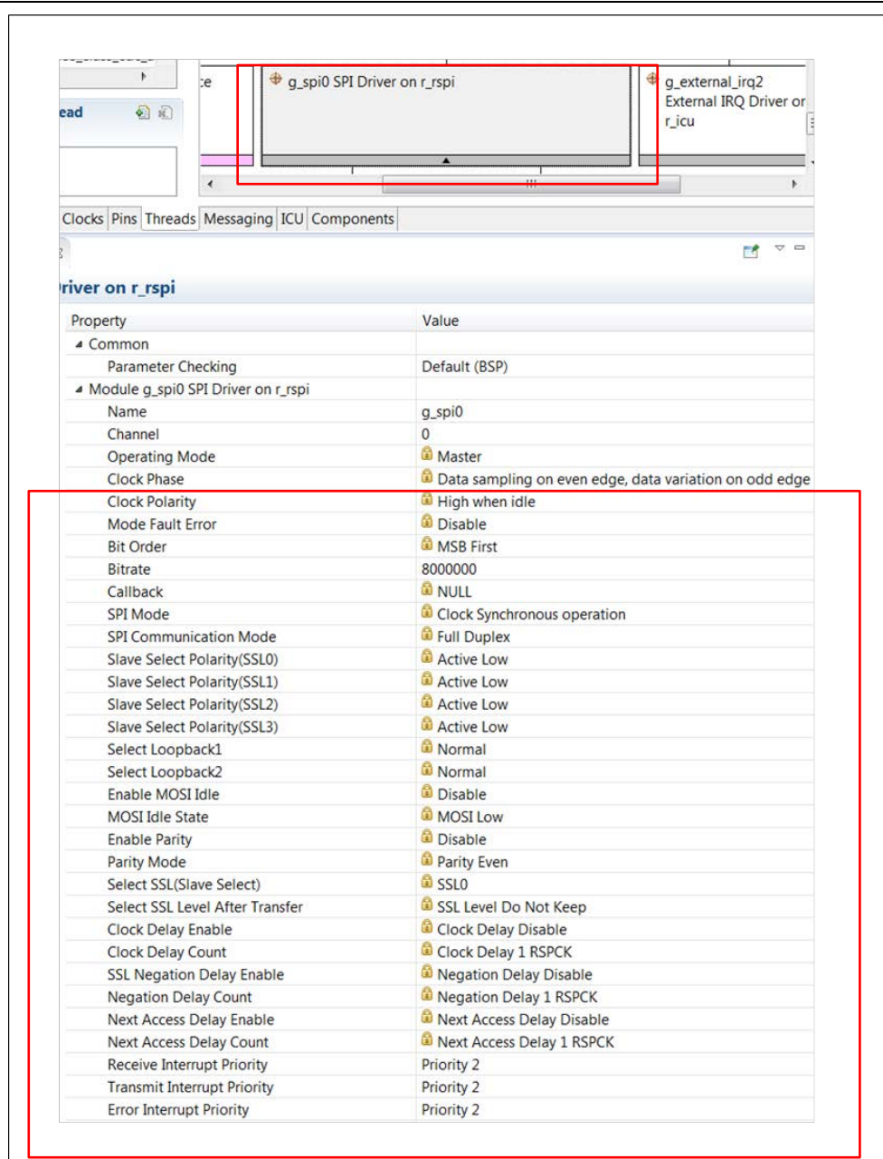
Figure 48. R_SPI configuration
